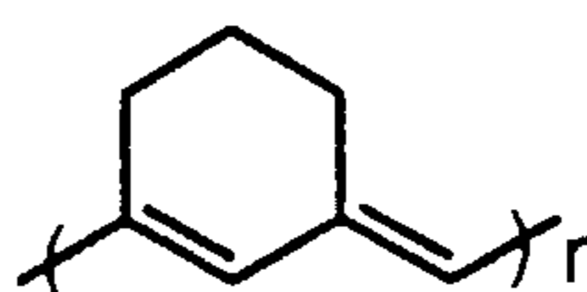
POLY(1,6-HEPTADIYNE) (PHT)
