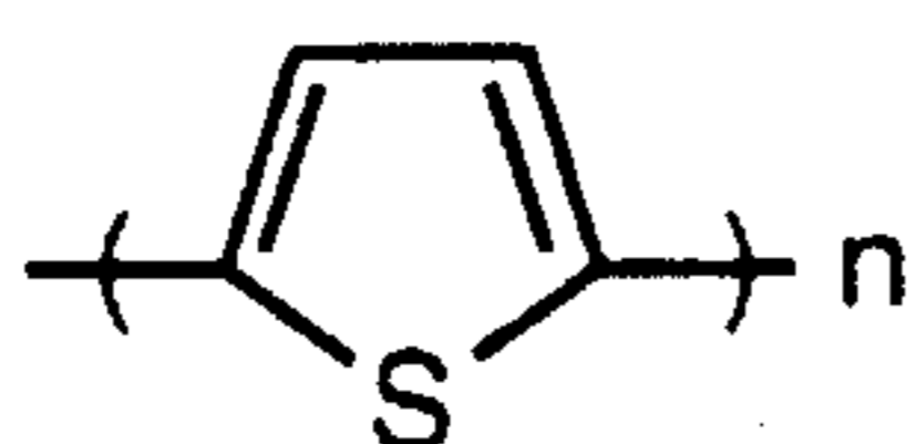
POLYTHIOPHENE (PT)
