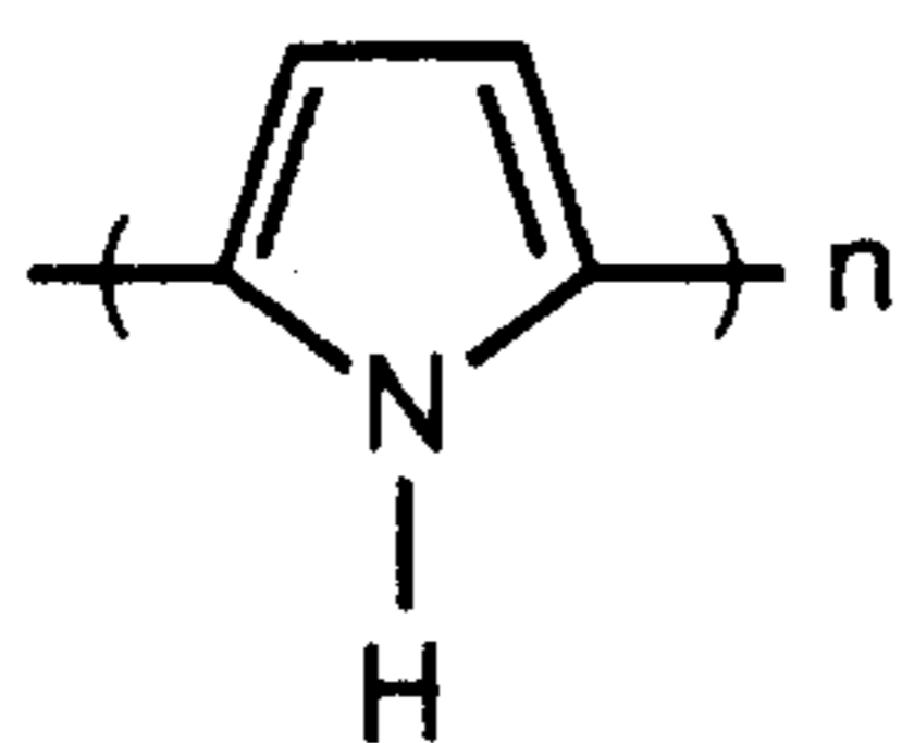
POLYPYRROLE (PP)
