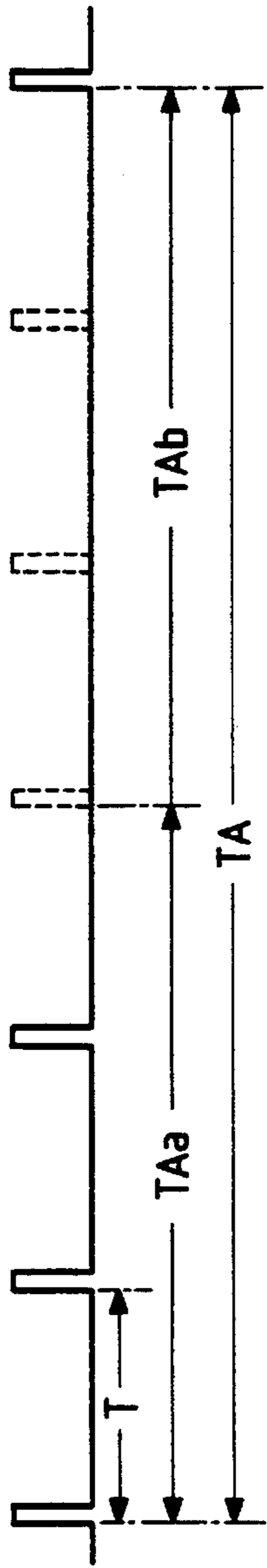
OPTICAL PULSE
