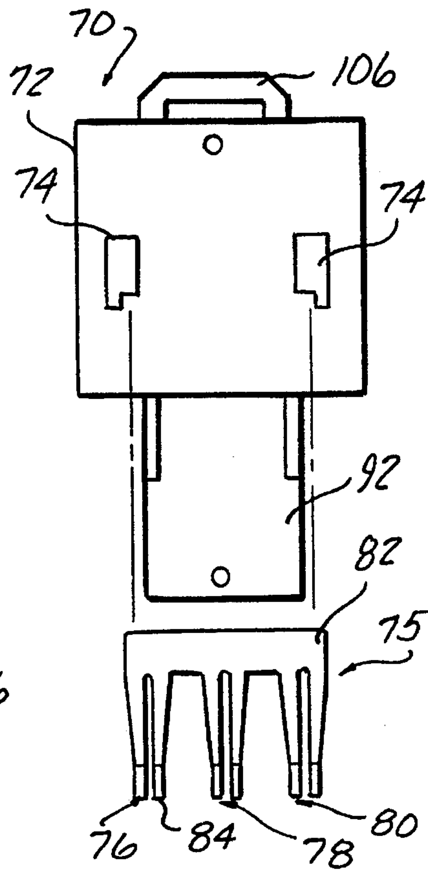
FIG-7
