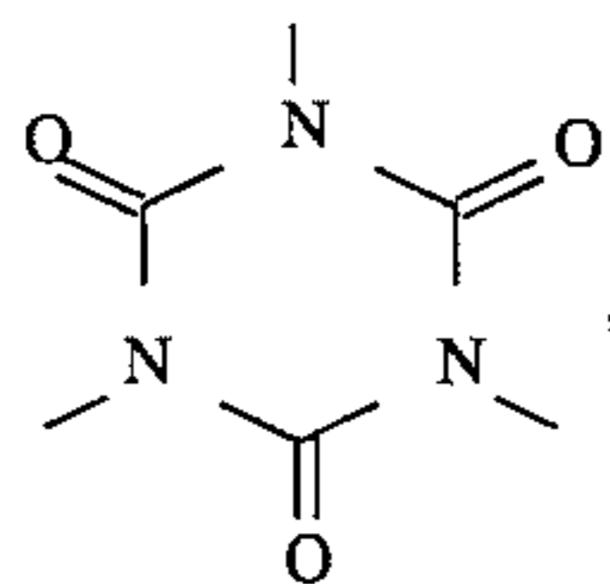
isocyanuratlylene
