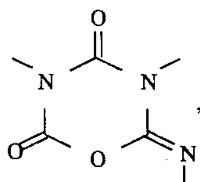
imino-4,6-dioxohexahydro-,3,5-oxdiazinylene
