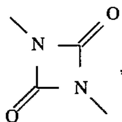
diazetidine-2,4-dionylene
