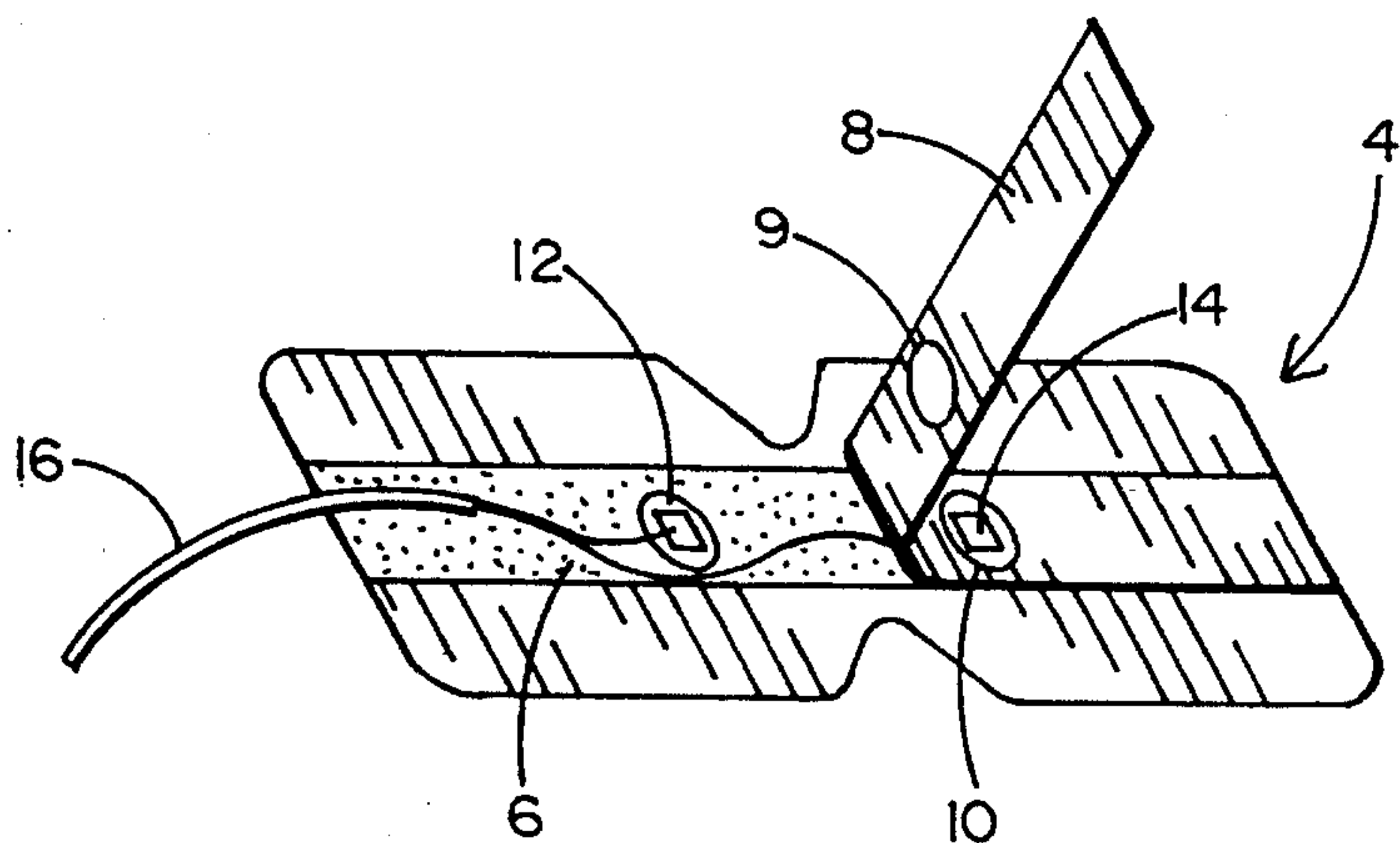
FIG. 2 PRIOR ART
