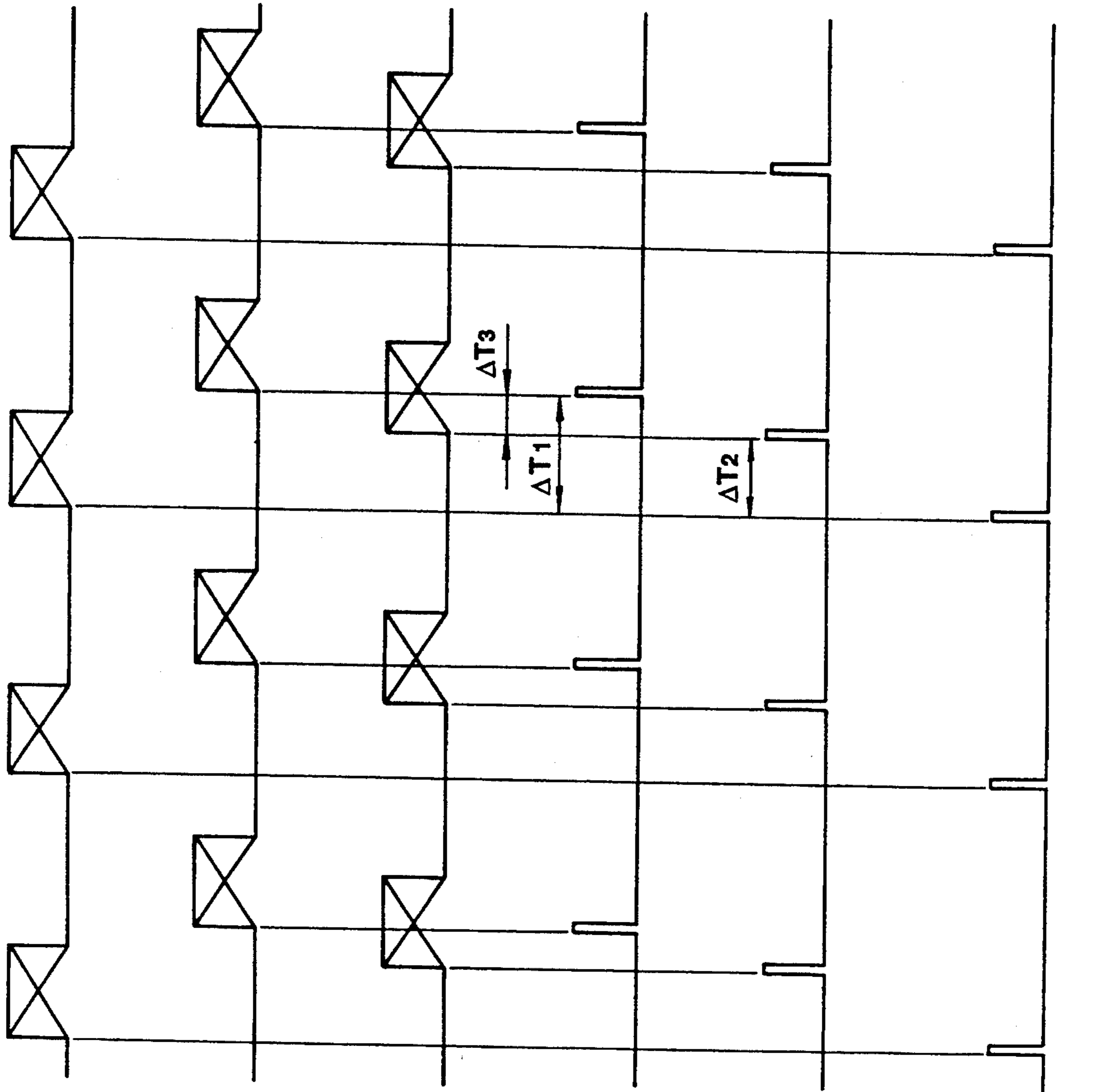
POSITION-DETECTING REFERENCE SIGNAL
