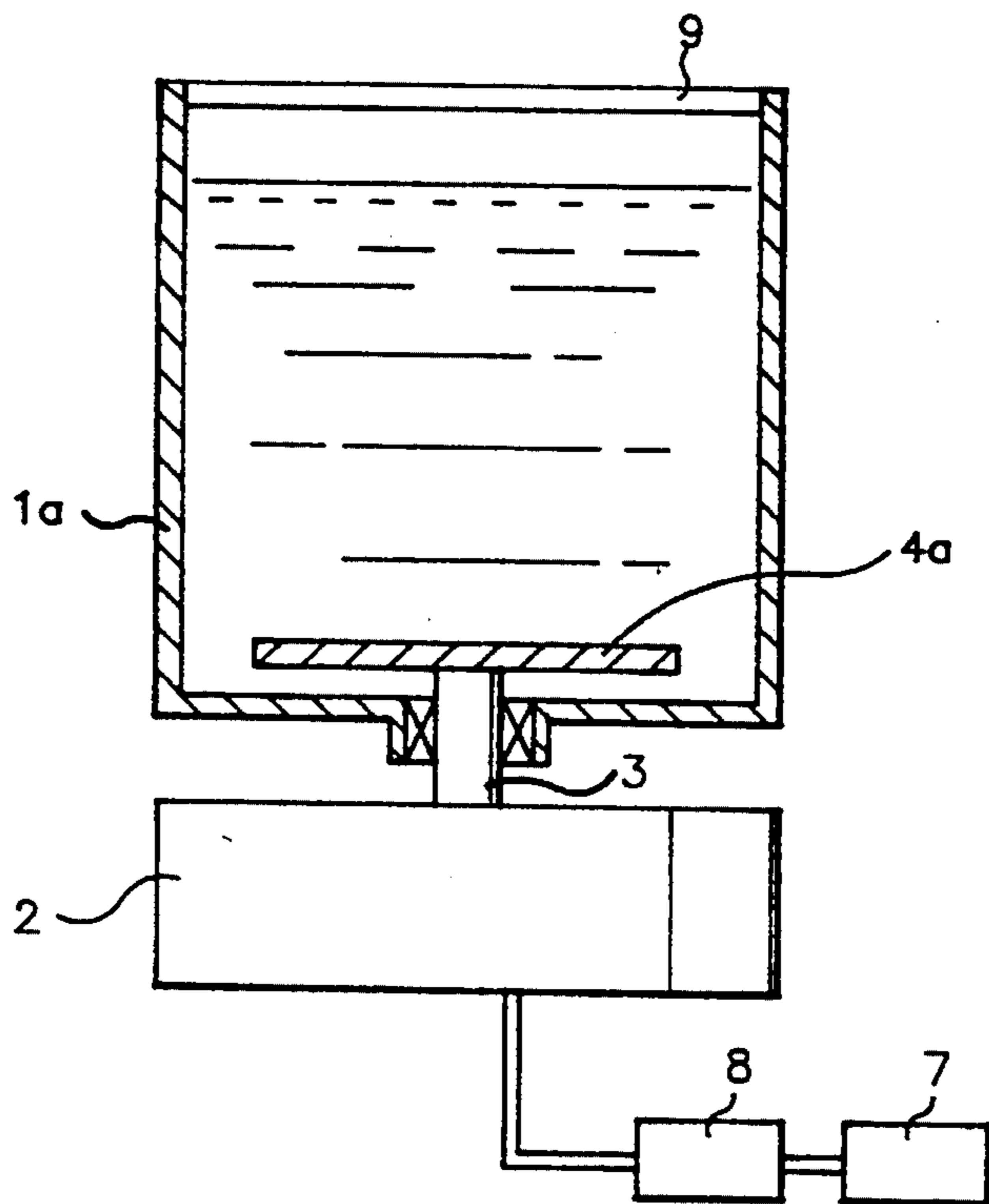
FIG. 1 PRIOR ART
