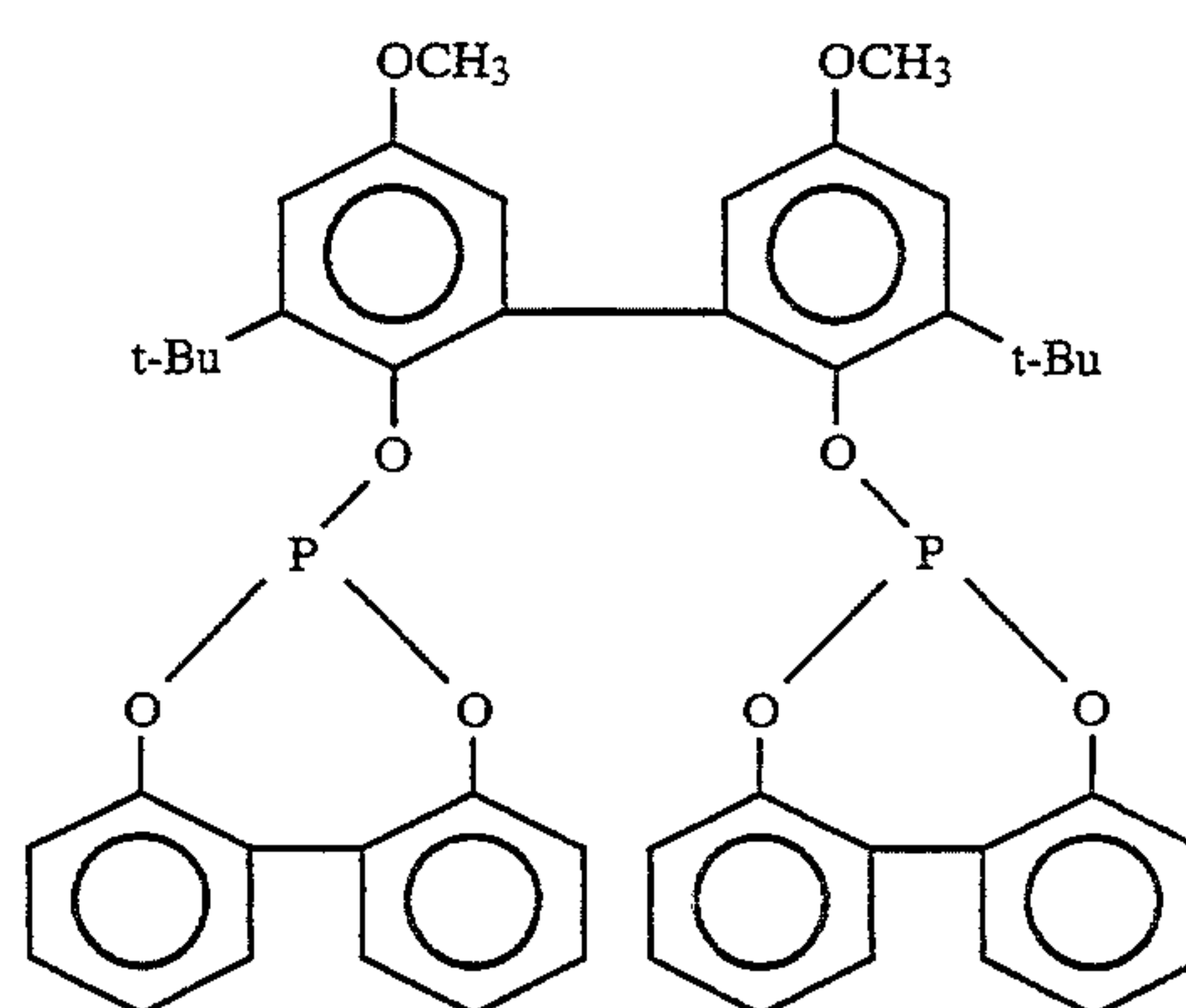
LIGAND III
