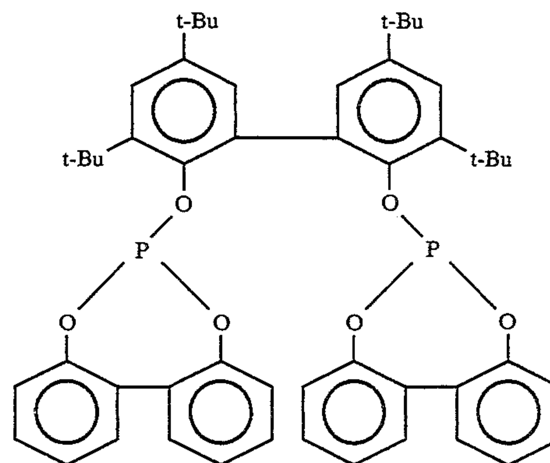
LIGAND IV
