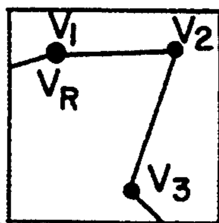
FIRST VORTEX
