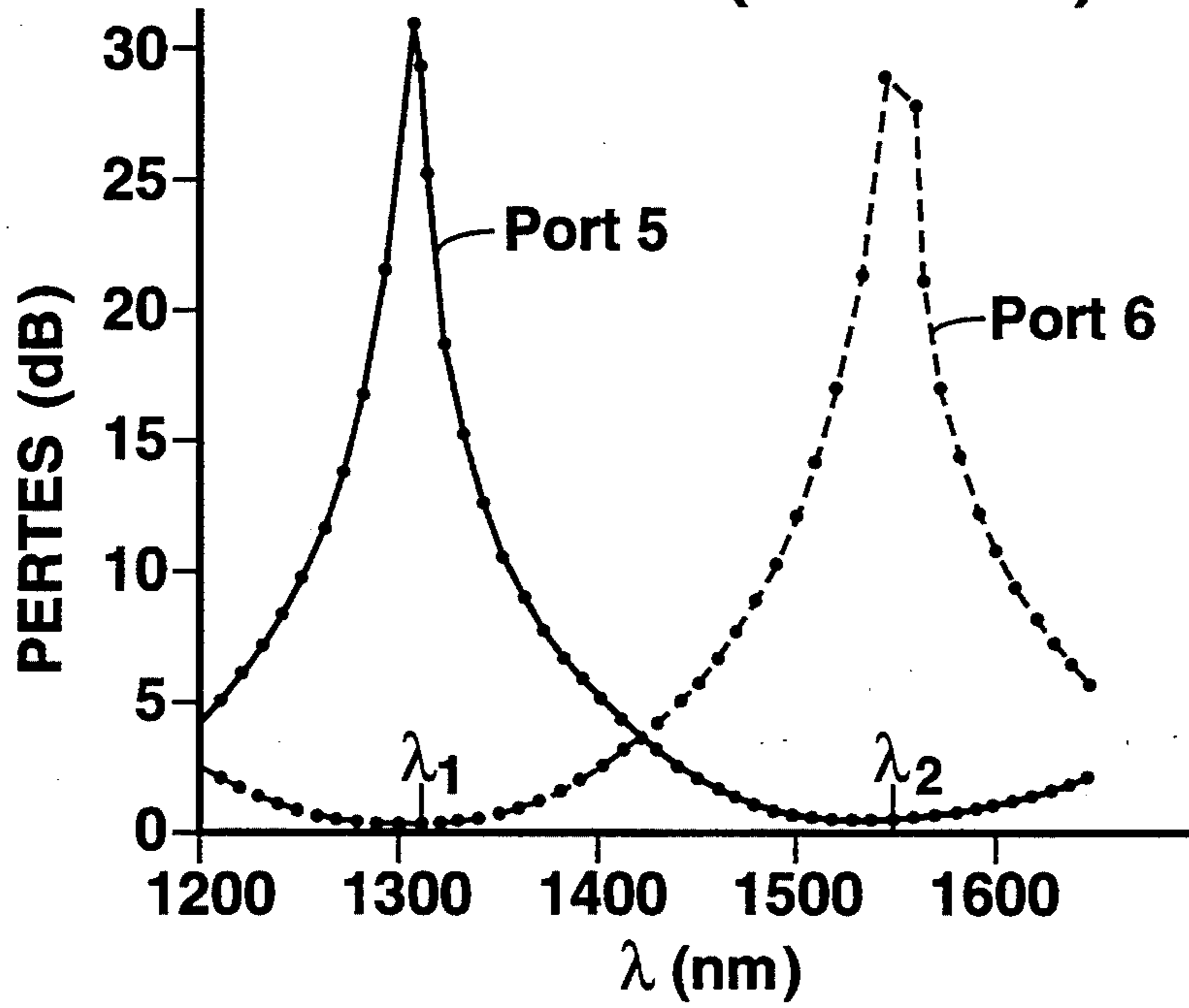
FIG. 2 (Prior Art)
