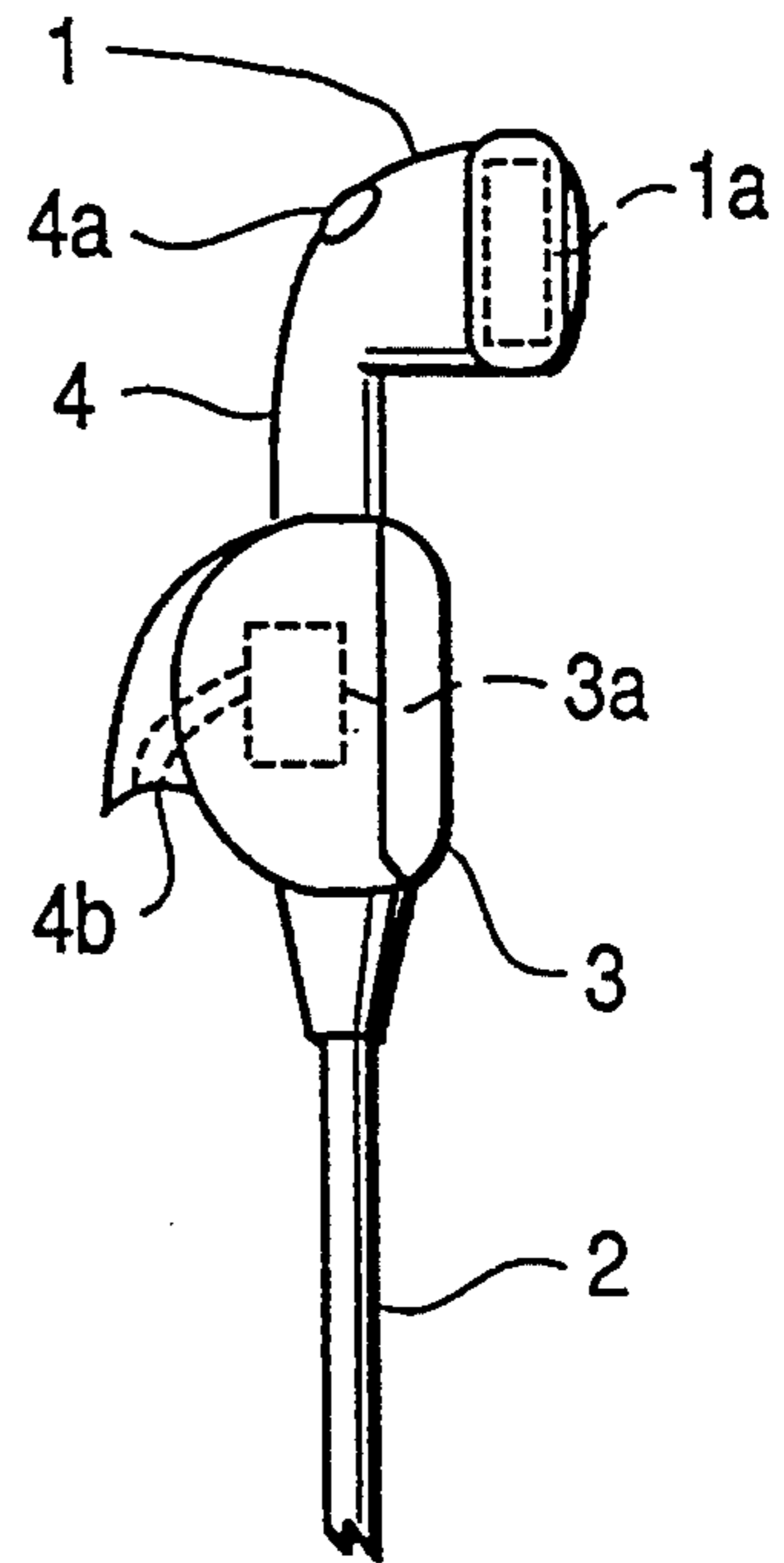
FIG. 2 PRIOR ART
