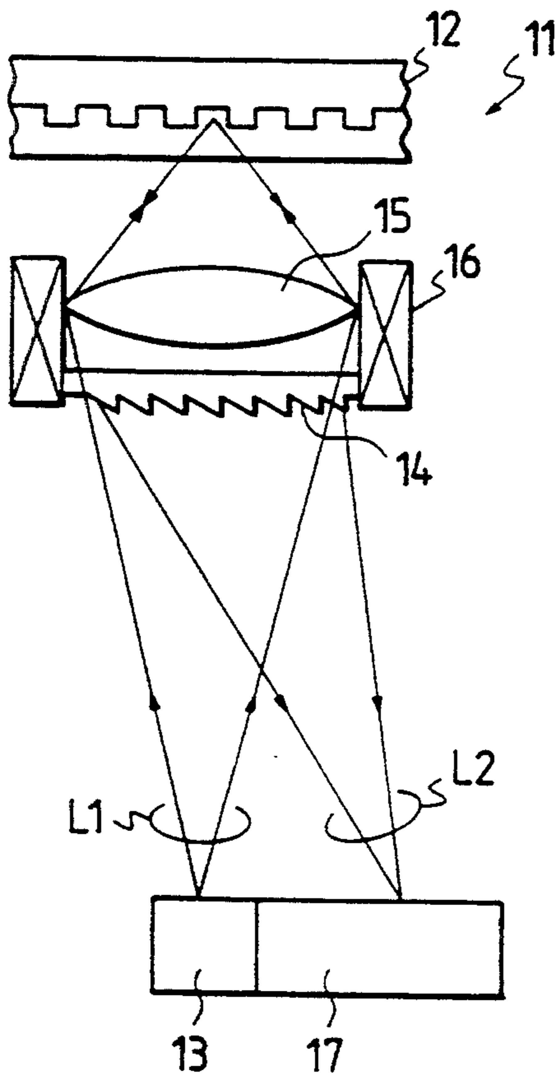
FIG. 1 PRIOR ART
