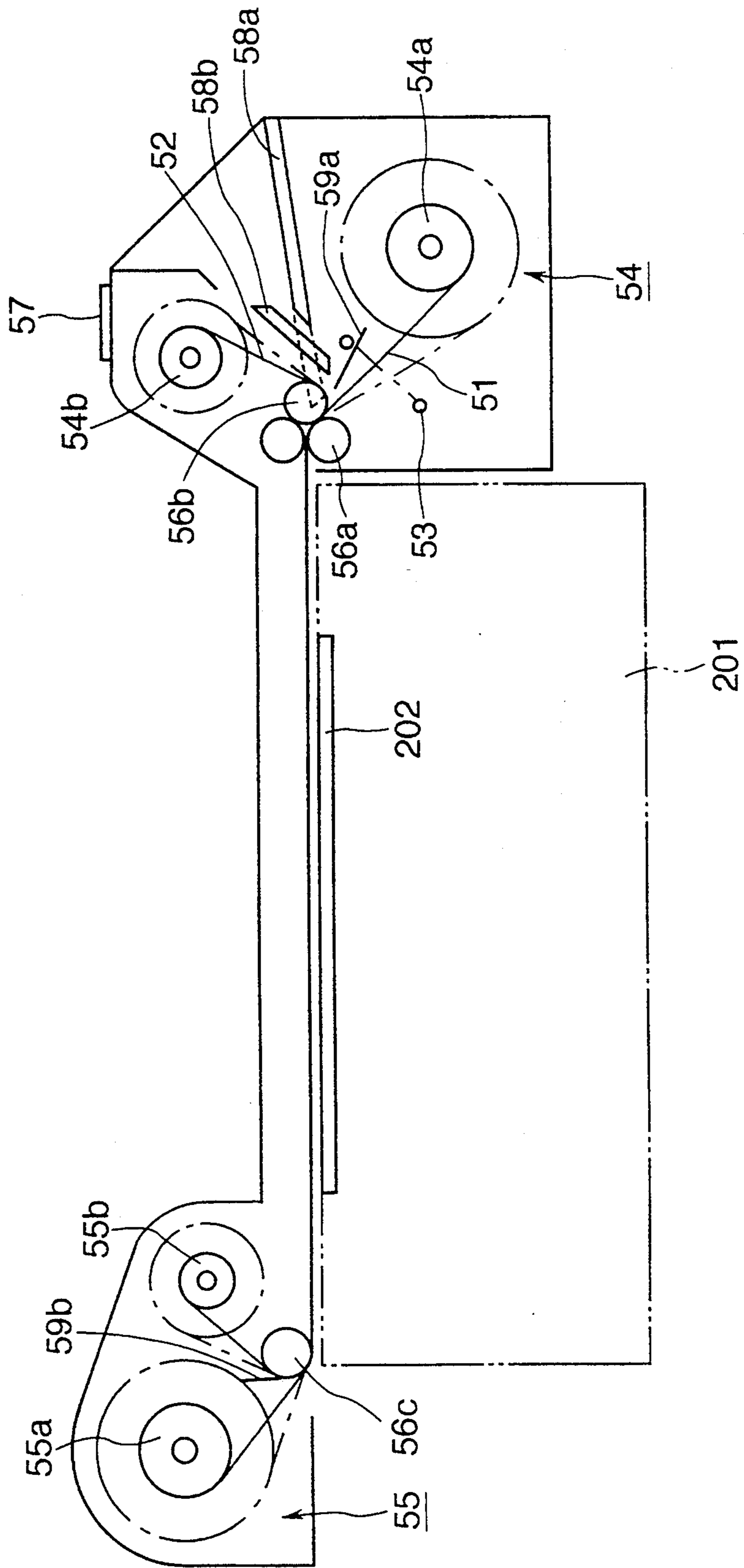
FIG. 7 PRIOR ART
