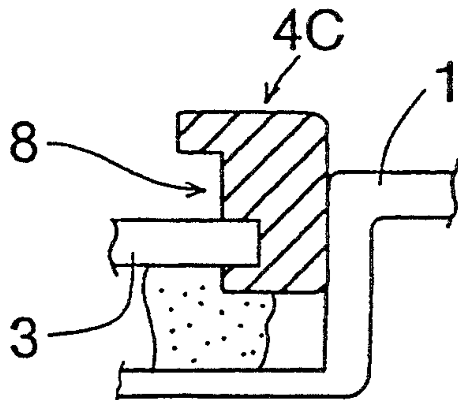
FIG.20 (C) PRIOR ART
