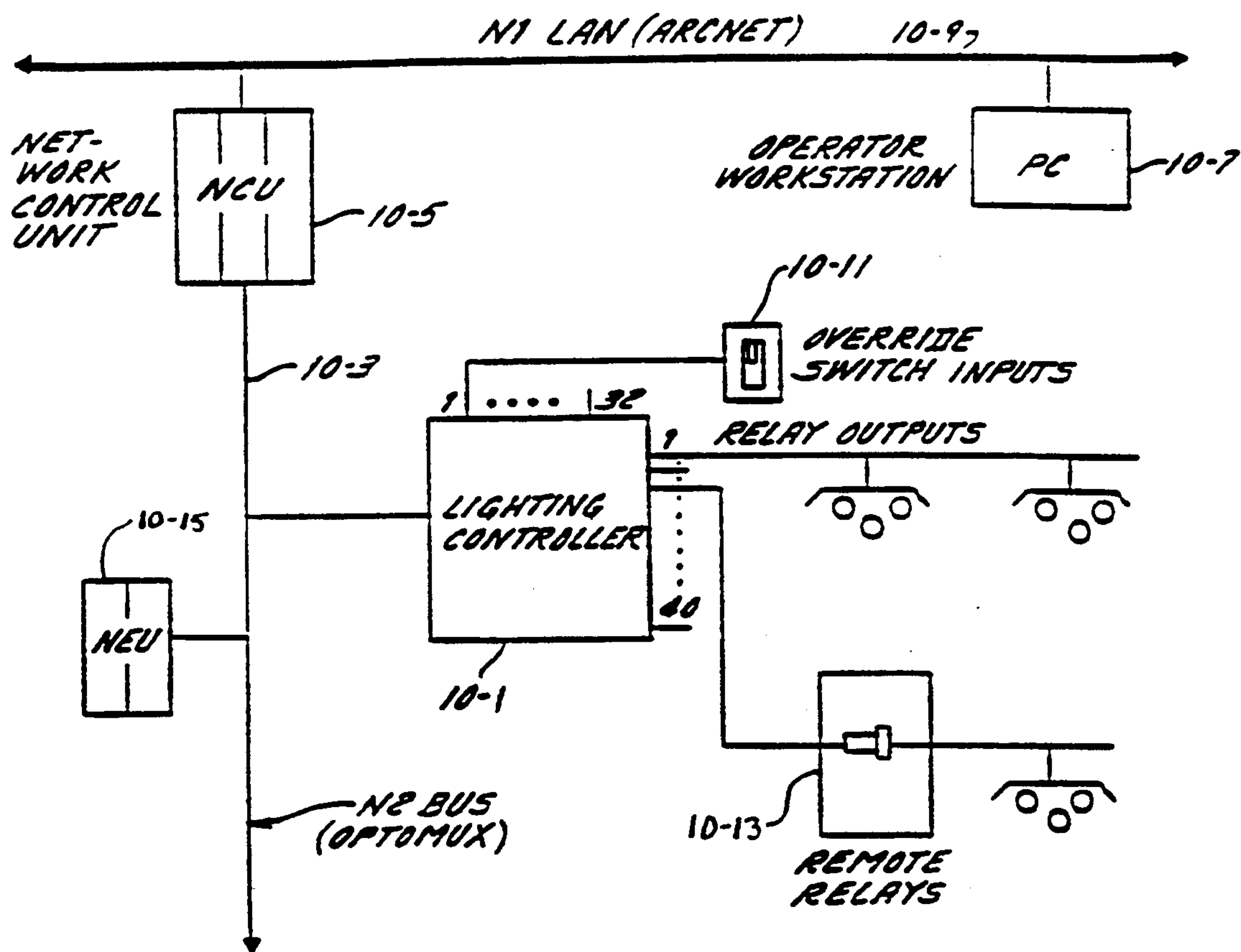
LIGHTING CONTROLLER FIG. 10
