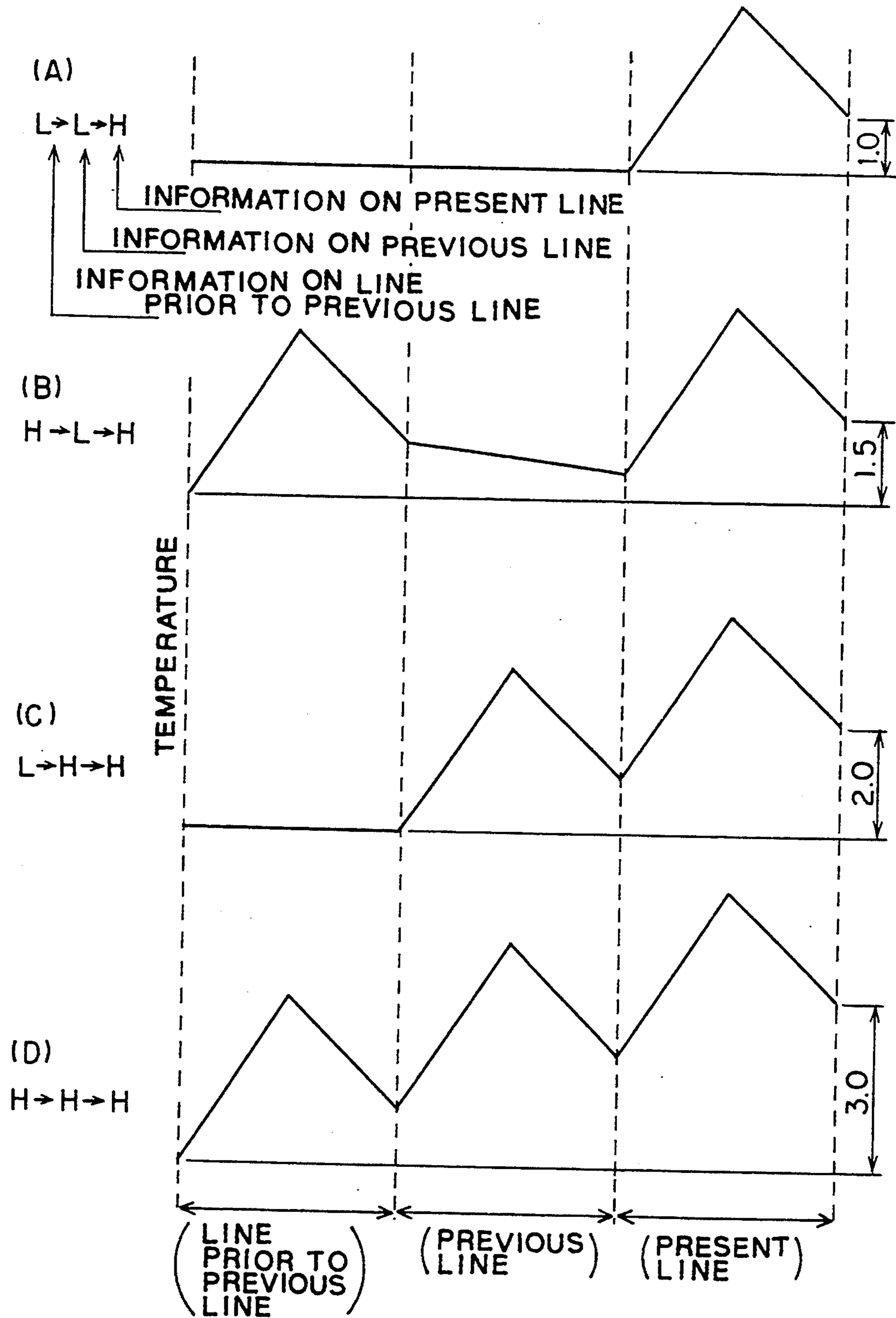
FIG. 3 (PRIOR ART)
