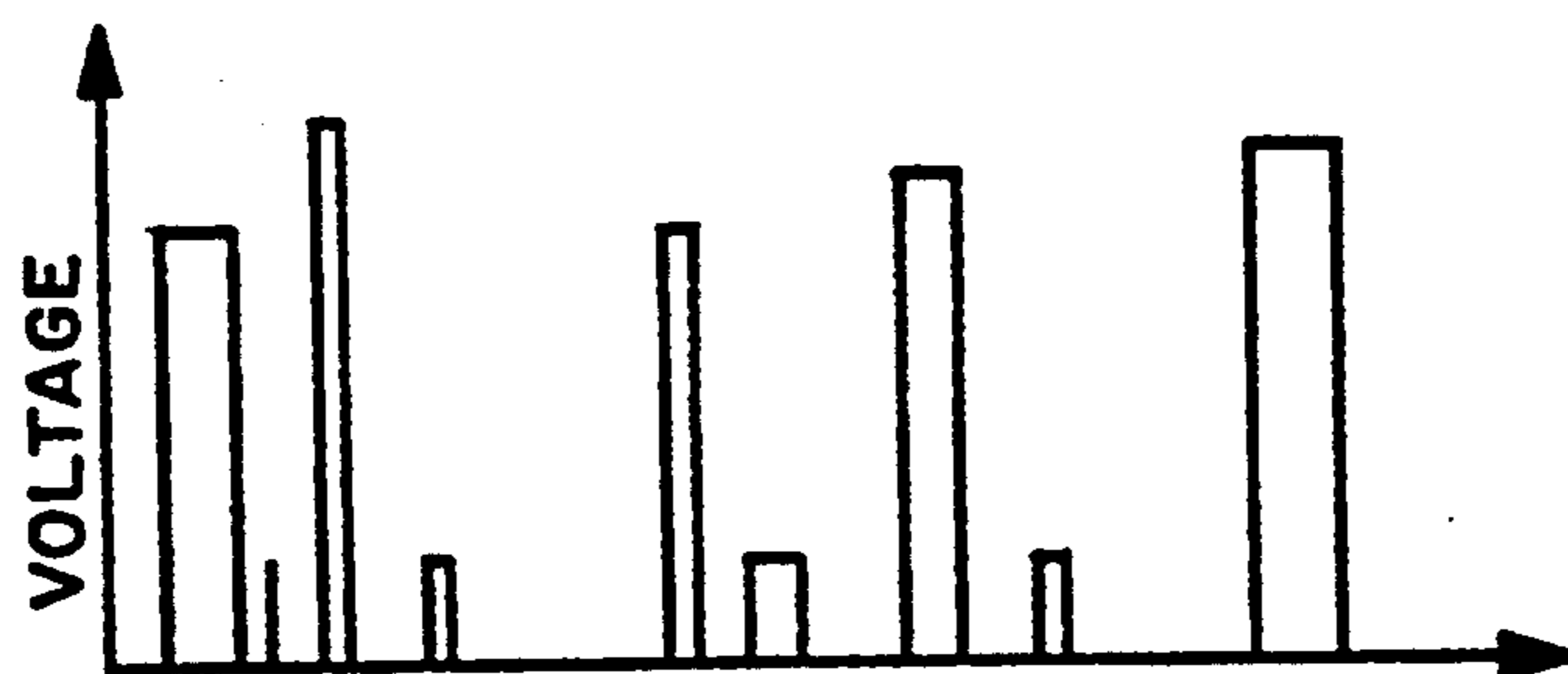
EXAMPLE OF DRIVE VOLTAGES FOR PIXEL WITH SELECTIVE VOLTAGE, DWELL AND FREQUENCY.
