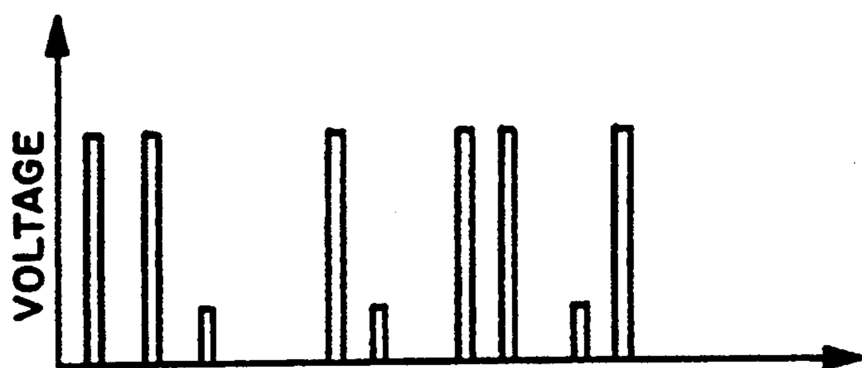
EXAMPLE OF DRIVE VOLTAGES FOR PIXEL WITH SELECTIVE FREQUENCY.
