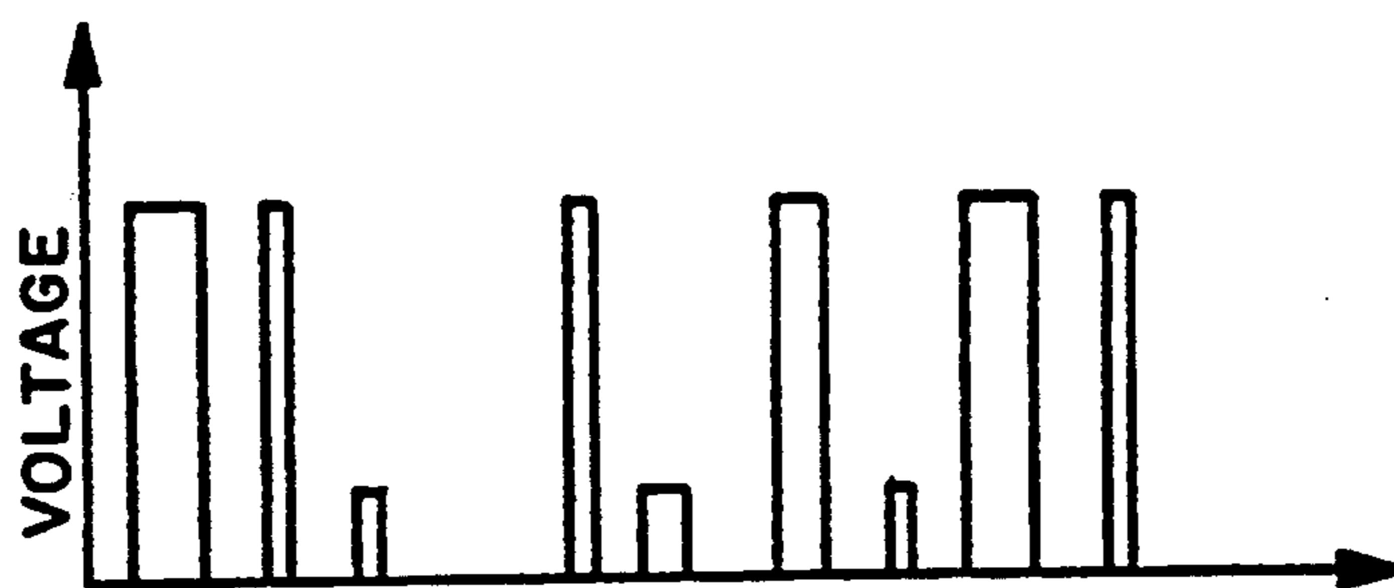
EXAMPLE OF DRIVE VOLTAGES FOR PIXEL WITH SELECTIVE DWELL.
