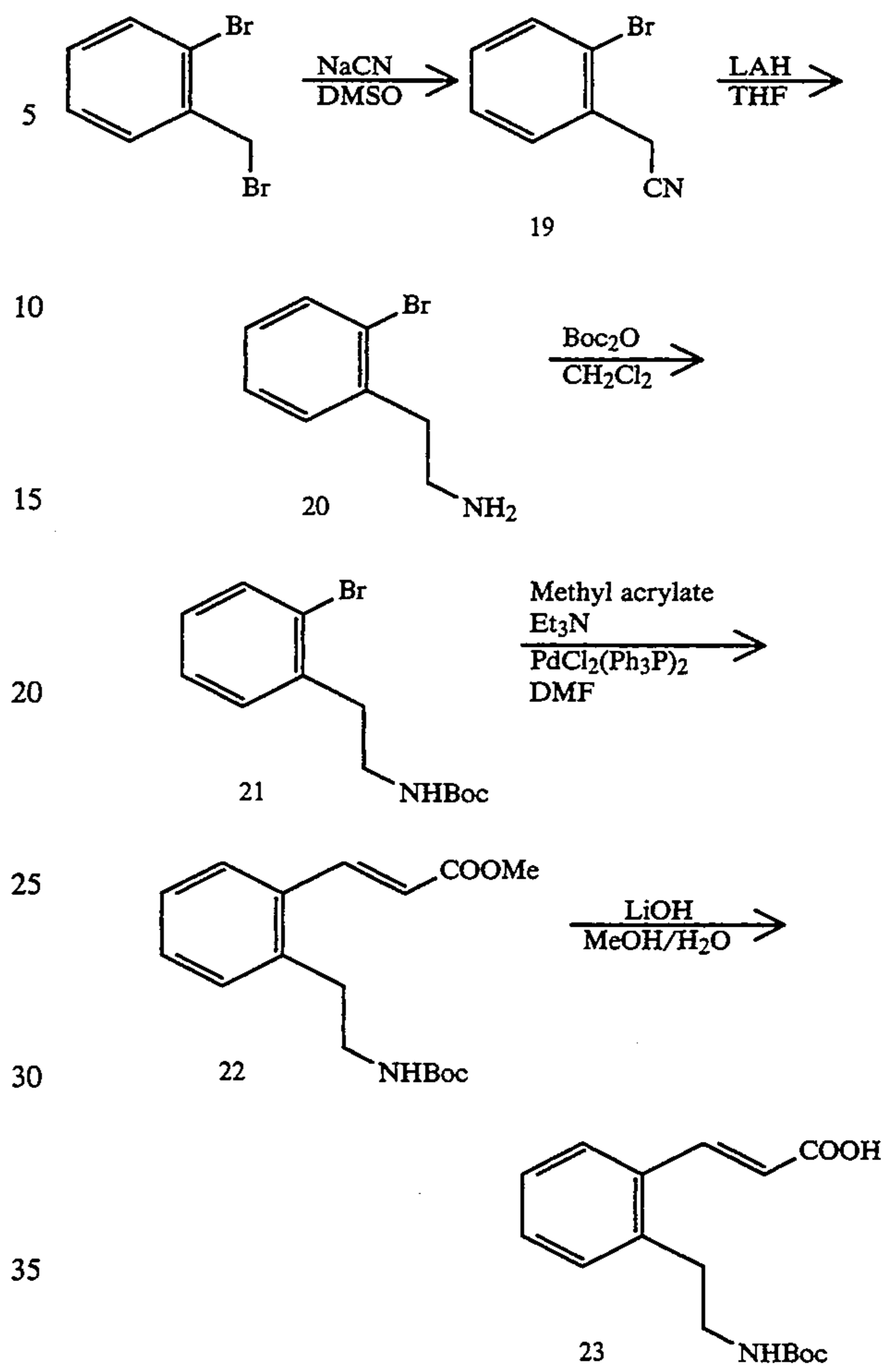
Scheme V
