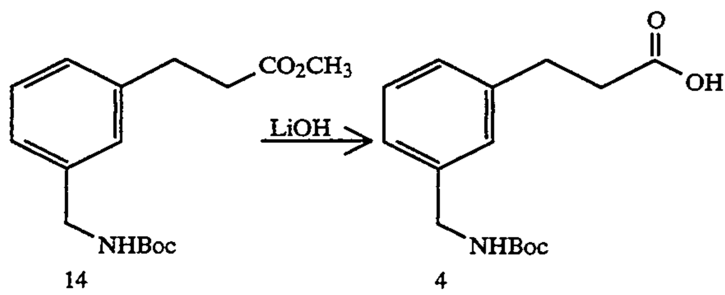
Scheme III
