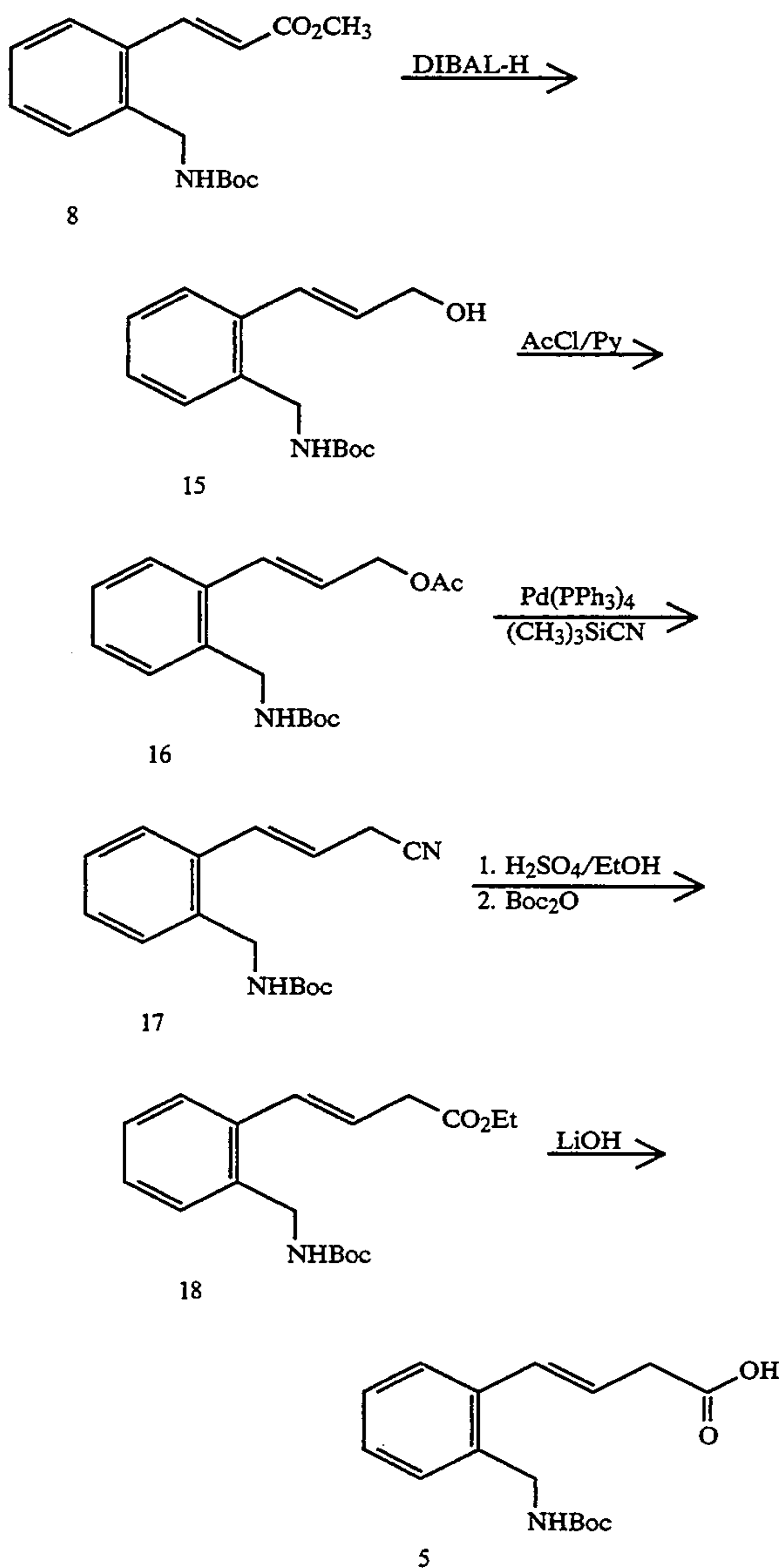
Scheme IV
