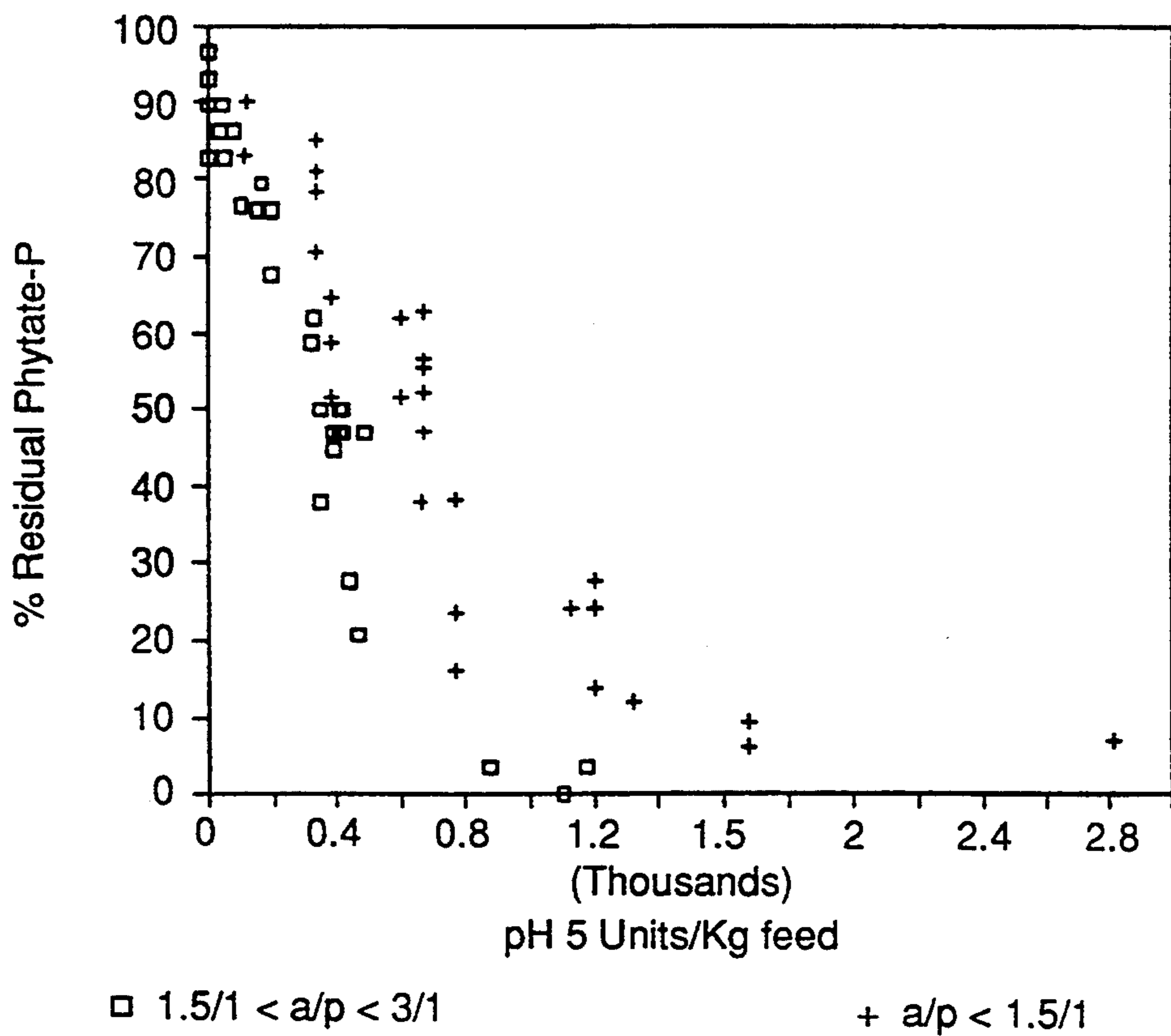
in vitro phytin hydrolysis by A. ficuum phytase preparations in function of pH 5.0 activity
