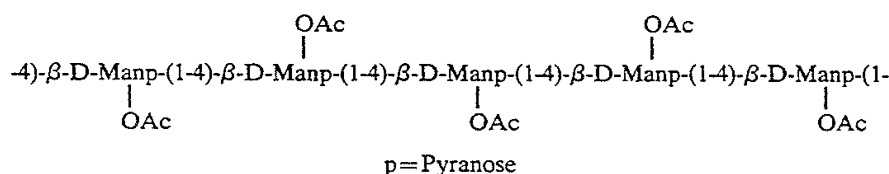
General Structure of Ultrapure Acemannan
