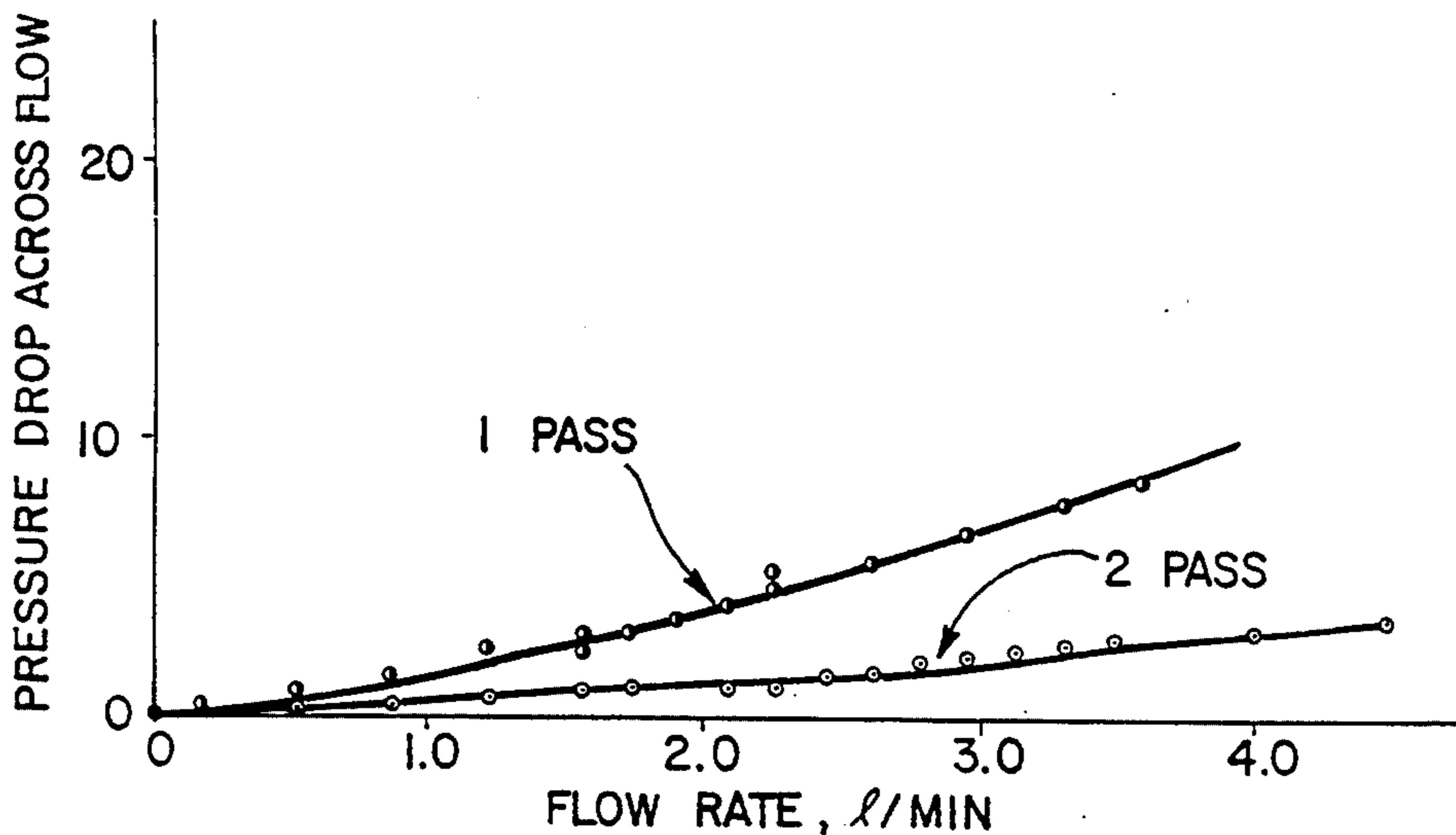
PRESSURE DROP AS A FUNCTION OF HYDROGEN FLOW RATE FOR DIFFERENT ANODE FLOW FIELD PASSAGE LENGTHS
