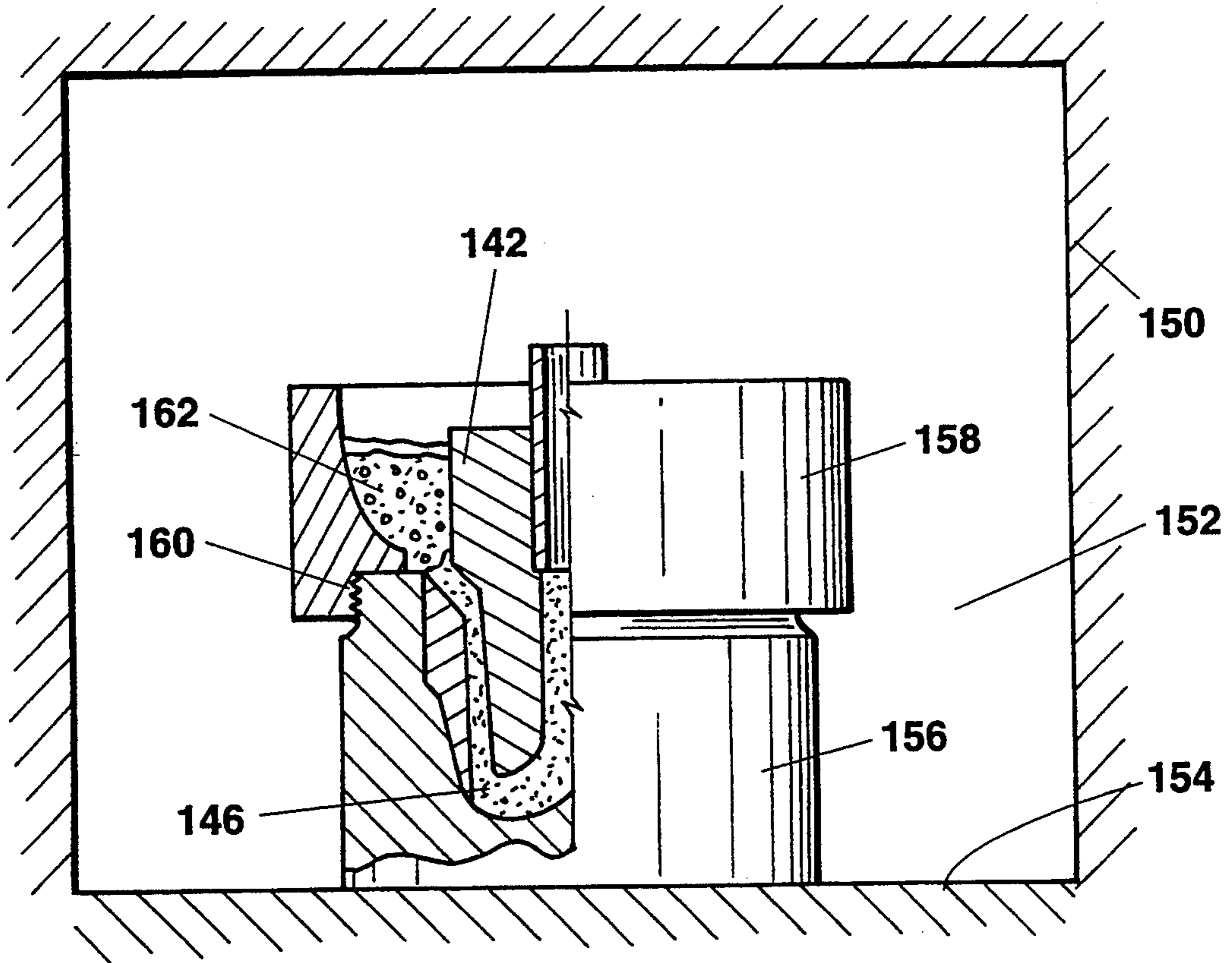
Fig. 19 (PRIOR ART)
