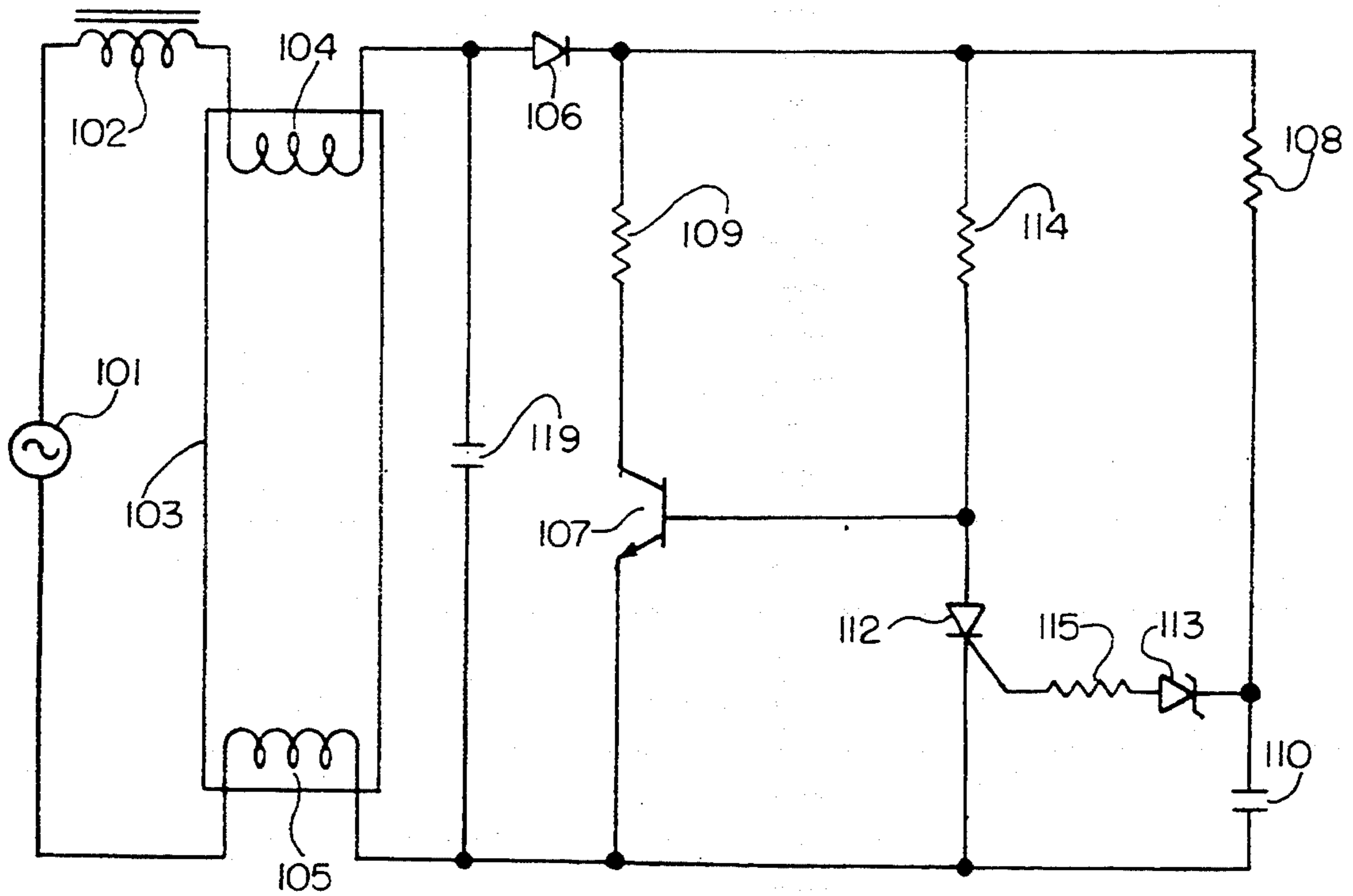
FIG. 5 PRIOR ART
