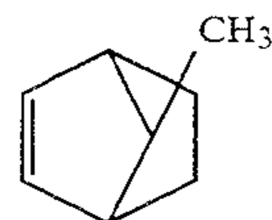
7-Methylbicyclo[2.2.1]hept-2-ene
