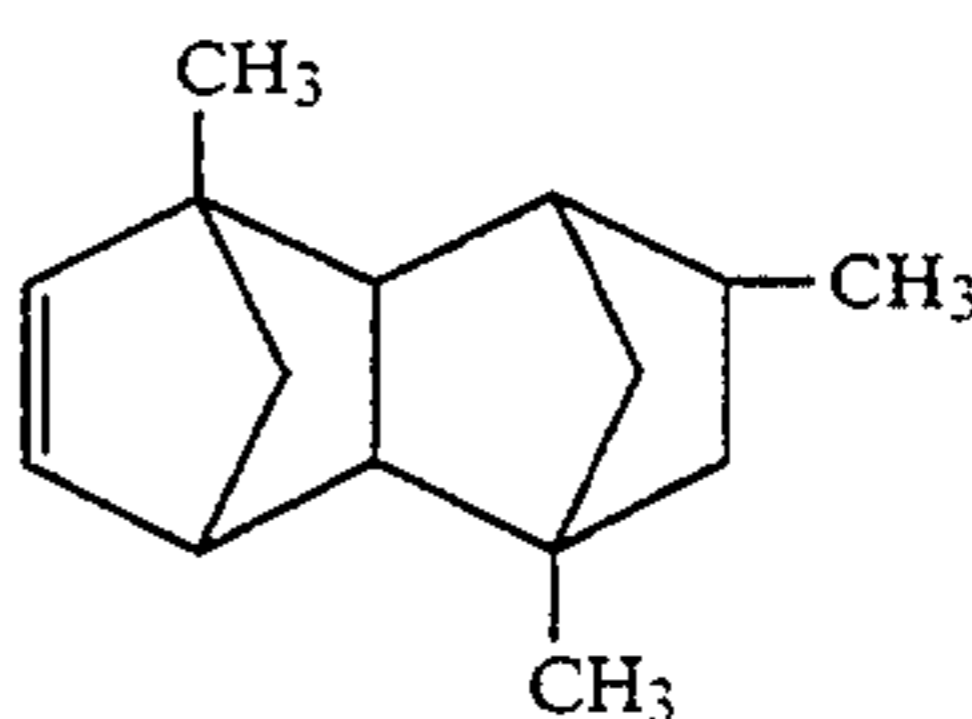
2,7,9-Trimethyltetracyclo[4,4,0,1 2.5 ,1 7.10 ]-3-dodecene
