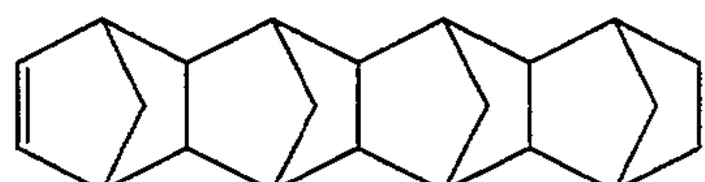
Octacyclo[8.8.0.1 2.9 .1 4.7 .1 11.18 .1 13.16 .0 3.8 .0 12.17 ]-5-docosene
