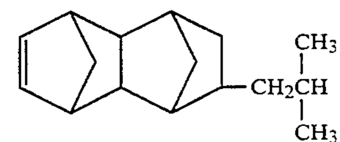
8-Isobutyltetracyclo[4,4,0,1 2.5 ,1 7.10 ]-3-dodecene
