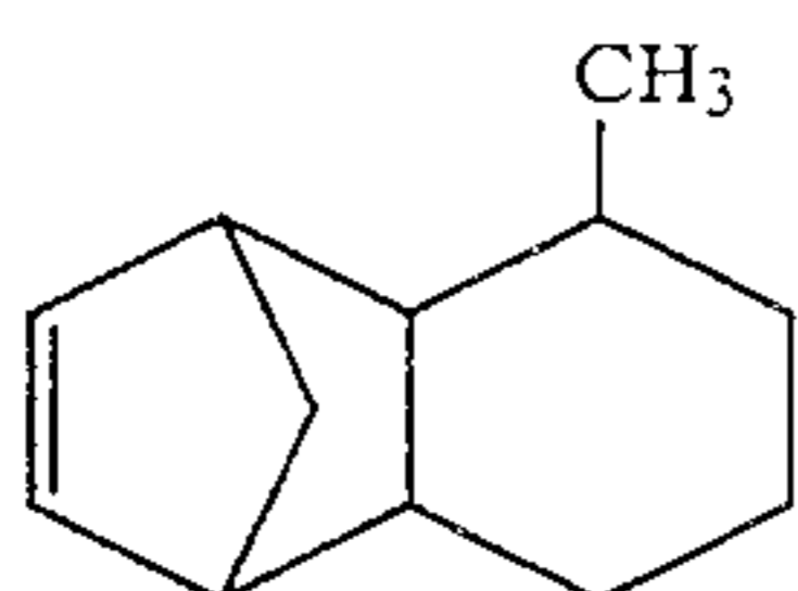
10-Methyltricyclo[4,4,0,1 2,5 ]-3-undecene
