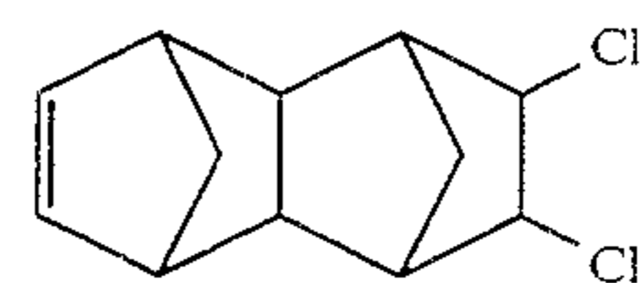
8,9-Dichloro-tetracyclo- [4,4,0,1 2.5 ,1 7.10 ]-3-dodecene
