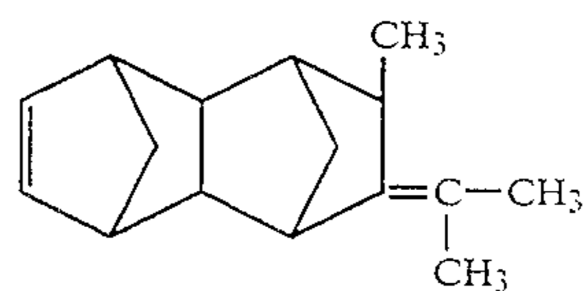
8-Isopropylidene-9-methyl-tetracyclo- [4,4,0,1 2.5 ,1 7.10 ]-3-dodecene
