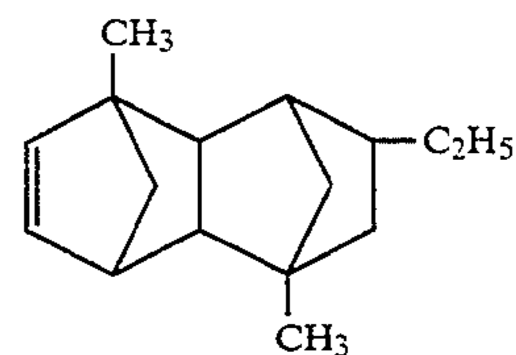
9-Ethyl-2,7-dimethyltetracyclo[4,4,0,1 2.5 ,1 7.10 ]-3-dodecene
