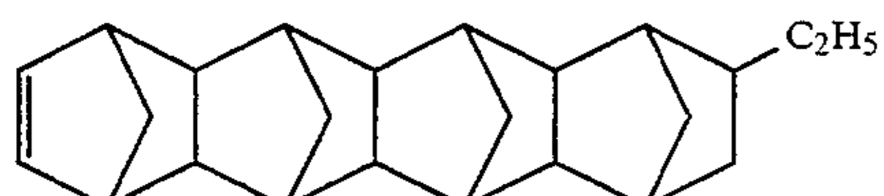
15-Ethyloctacyclo[8.8.0.1 2.9 .1 4.7 .1 11.18 .1 13.16 .0 3.8 .0 12.17 ]-5-docosene
