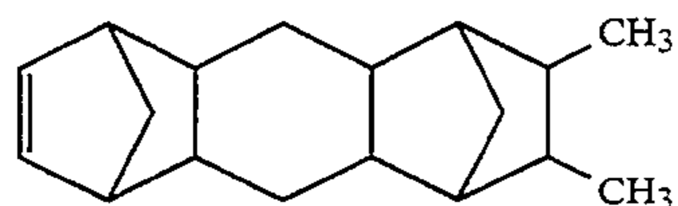
10,11-Dimethylpentacyclo[8,4,0,1 2,5 ,1 9,12 ,0 8,13 ]-3-hexadecene;
