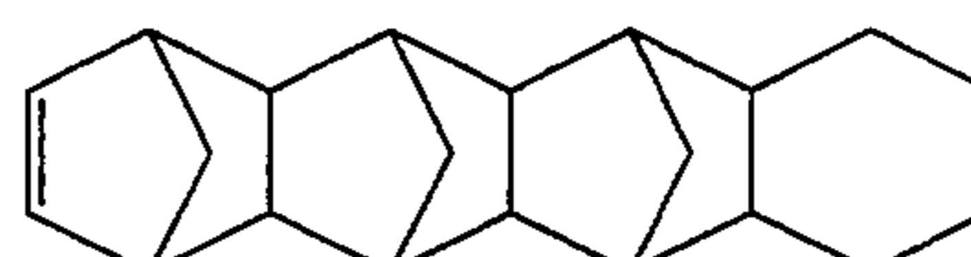
Heptacyclo[8.7.0.1 2.9 .1 4.7 .1 11.18 .0 3.8 .0 12.17 ]-5-heneicosene
