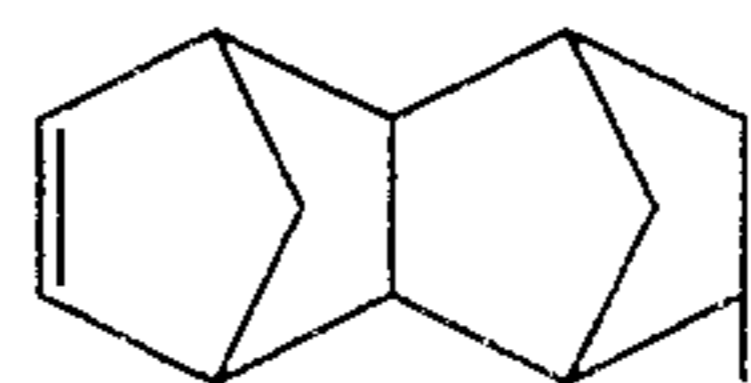
8-Ethyltetracyclo[4.4.0.1 2,5 .1 7,10 ]-3-dodecene
