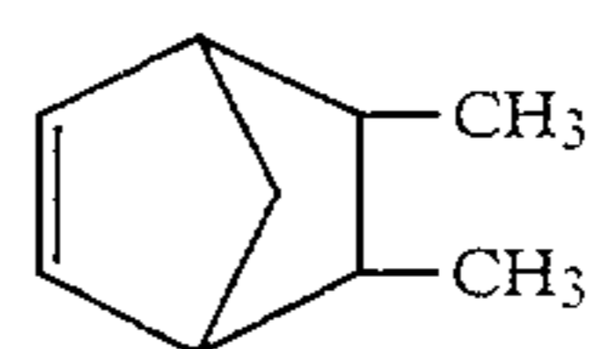
5,6-Dimethylbicyclo[2.2.1]hept-2-ene
