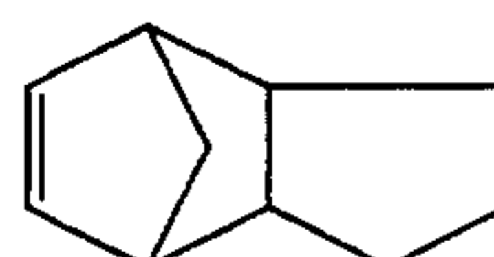
Tricyclo[4.3.0.1 2.5 ]-3-decene
