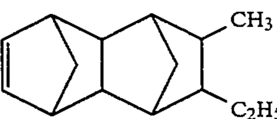
8-Ethyl-9-methyltetracyclo[4,4,0,1 2.5 ,1 7.10 ]-3-dodecene
