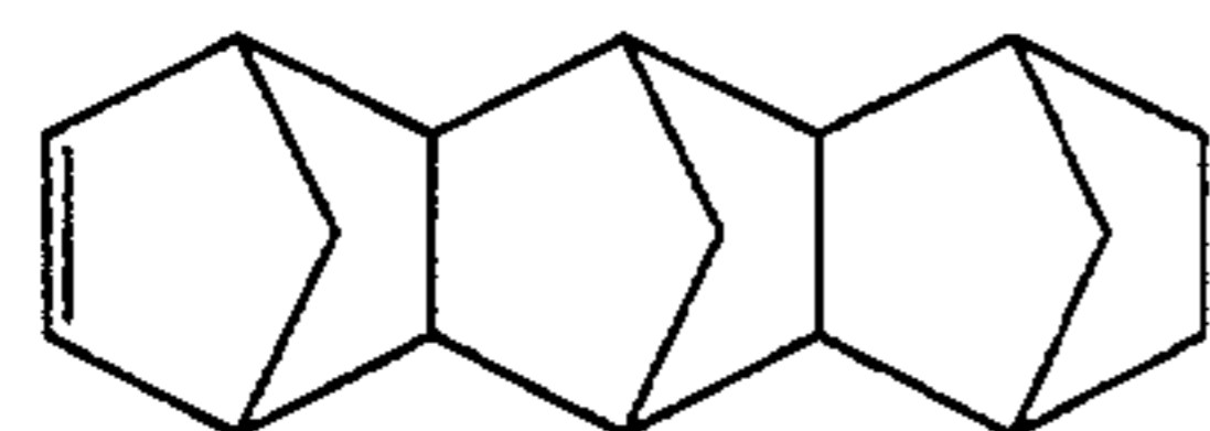
Hexacyclo[6.6.1.1 3.6 .1 10.13 .0 2.7 .0 9.14 ]-4-heptadecene
