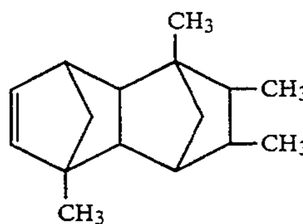
5,8,9,10-Trimethyltetracyclo[4,4,0,1 2.5 ,1 7.10 ]-3-dodecene
