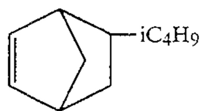
6-Isobutylbicyclo[2.2.1]hept-2-ene
