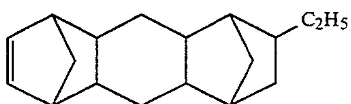
11-Ethylpentacyclo[8,4,0,1 2,5 ,1 9,12 ,0 8,13 ]-3-hexadecene
