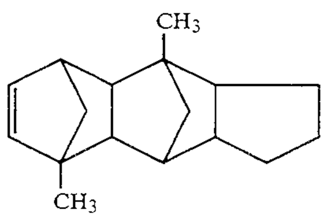
1,6-Dimethylpentacyclo[6,5,1,1 3,6 ,0 2,7 ,0 9,13 ]-4-pentadecene
