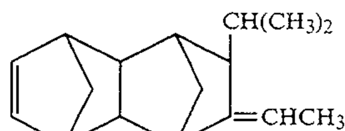
8-Ethylidene-9-isopropyl-tetracyclo- [4,4,0,1 2.5 ,1 7.10 ]-3-dodecene
