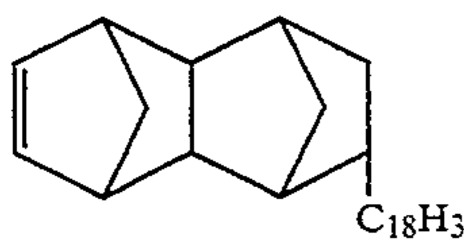
8-Stearyltetracyclo[4,4,0,1 2.5 ,1 7.10 ]-3-dodecene
