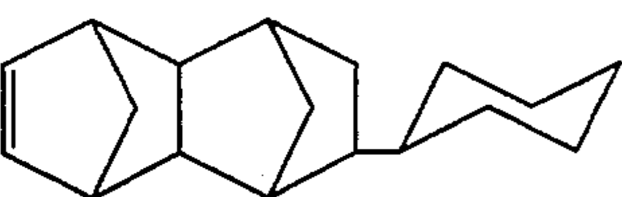
8-Cyclohexyltetracyclo[4,4,0,1 2.5 ,1 7.10 ]-3-dodecene
