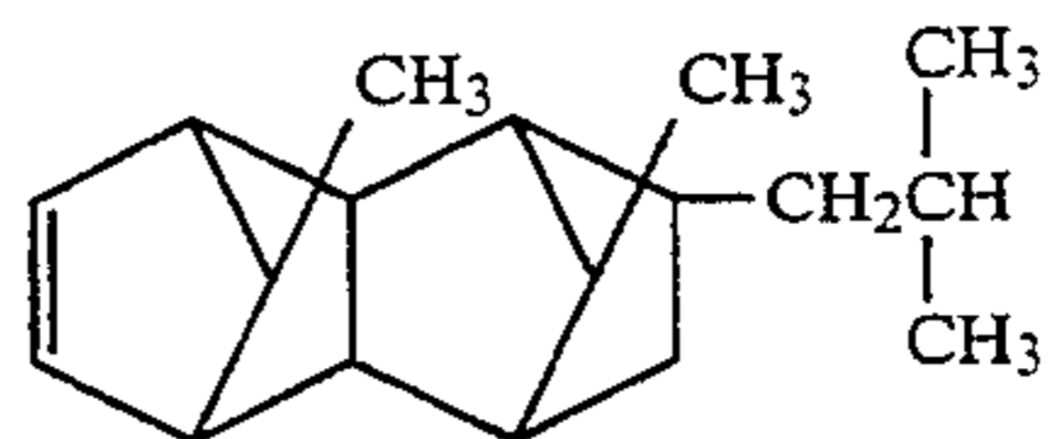
9-Isobutyl-11,12-dimethyltetracyclo[4,4,0,1 2.5 ,1 7.10 ]-3-dodecene
