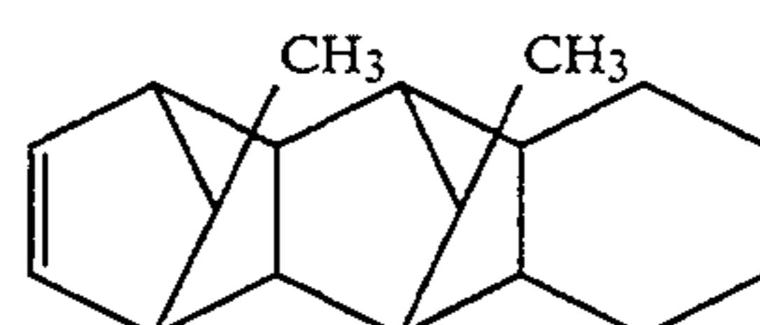
15,16-Dimethylpentacyclo[6.6.1.1 3.6 .0 2.7 .0 9.14 ]-4-hexadecene
