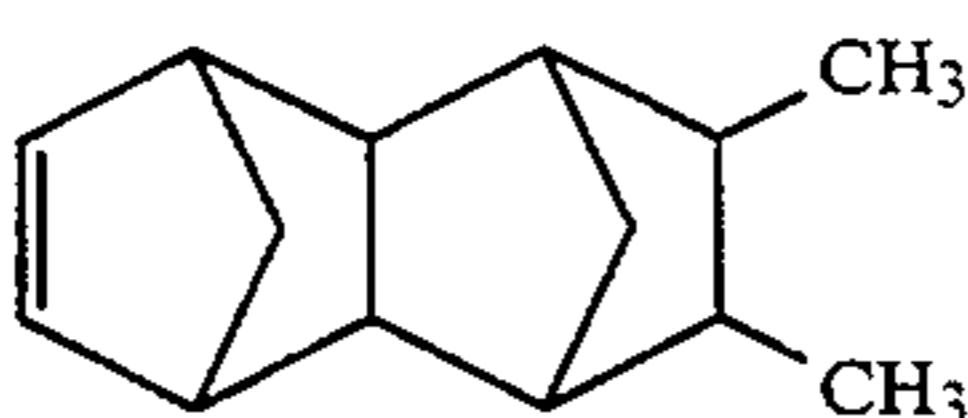
8,9-Dimethyltetracyclo[4,4,0,1 2.5 ,1 7.10 ]-3-dodecene
