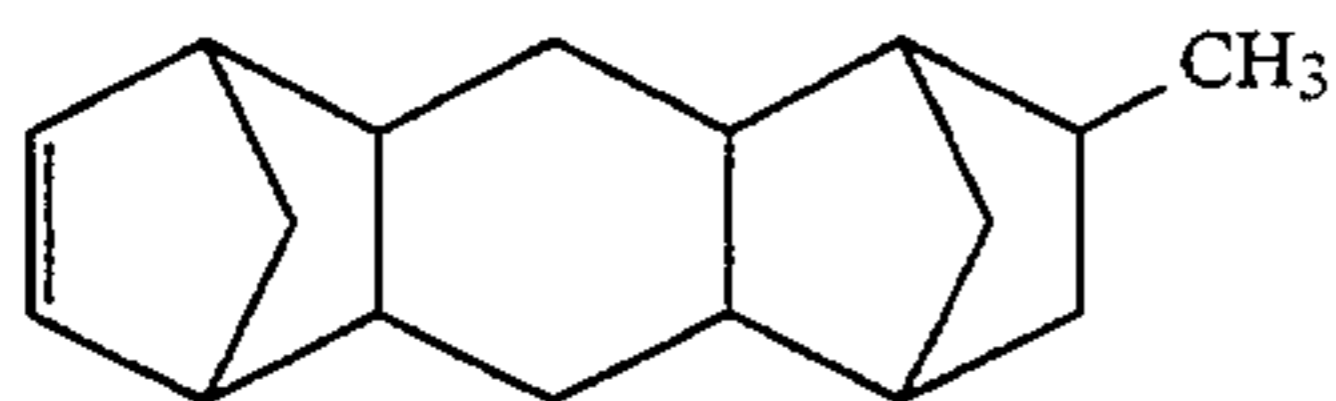
11-Methylpentacyclo[8,4,0,1 2,5 ,1 9,12 ,0 8,13 ]-3-hexadecene
