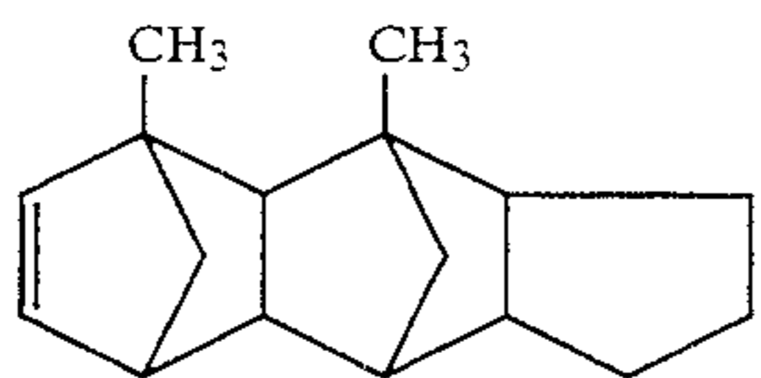
1,3-Dimethylpentacyclo[6,5,1,1 3,6 ,0 2,7 ,0 9,13 ]-4-pentadecene
