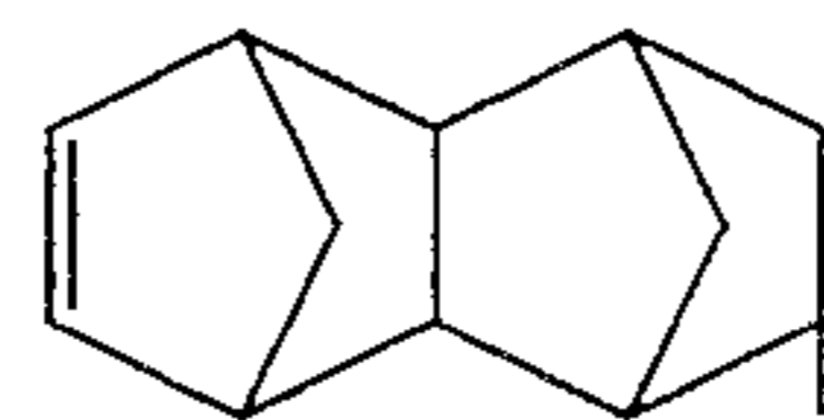
8-Methyltetracyclo[4.4.0.1 2,5 .1 7,10 ]-3-dodecene
