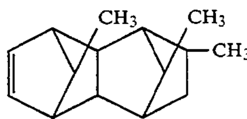
9,11,12-Trimethyltetracyclo[4,4,0,1 2.5 ,1 7.10 ]-3-dodecene
