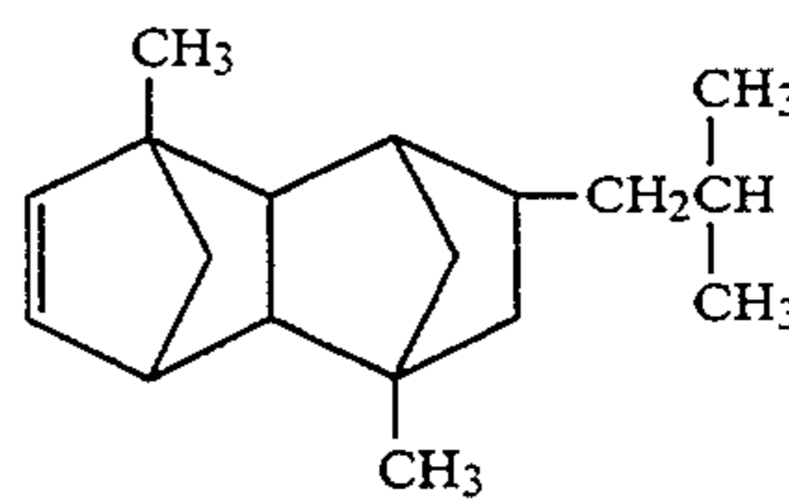
9-Isobutyl-2,7-dimethyltetracyclo[4,4,0,1 2.5 ,1 7.10 ]-3-dodecene
