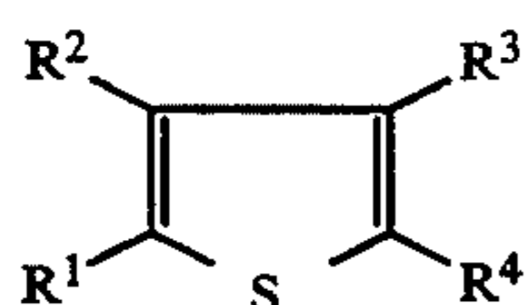
thiophenes
