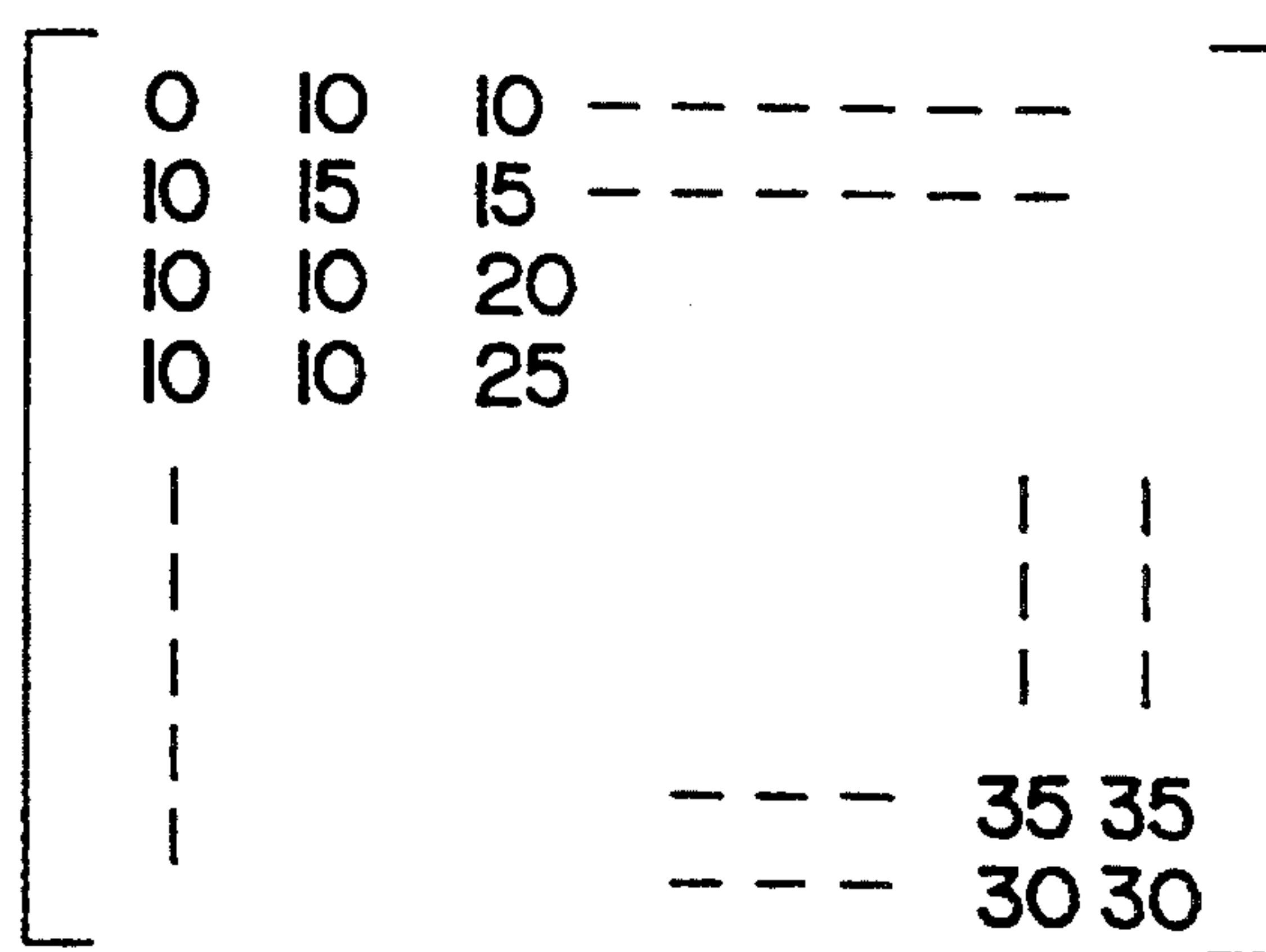
EXAMPLE OF THRESHOLD MAP FOR 64 DCT COEFFICIENTS
