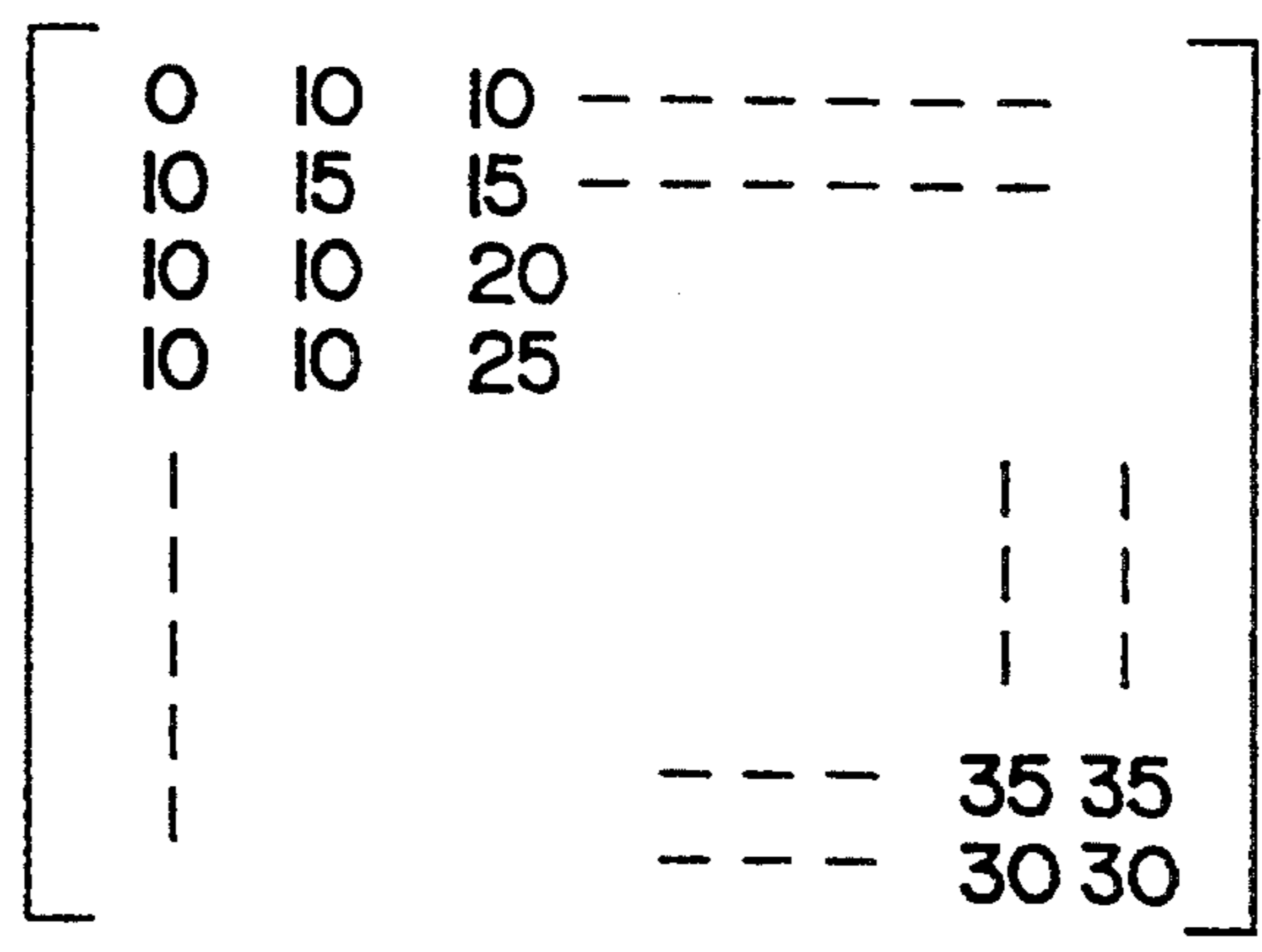
EXAMPLE OF THRESHOLD MAP FOR 64 DCT COEFFICIENTS
