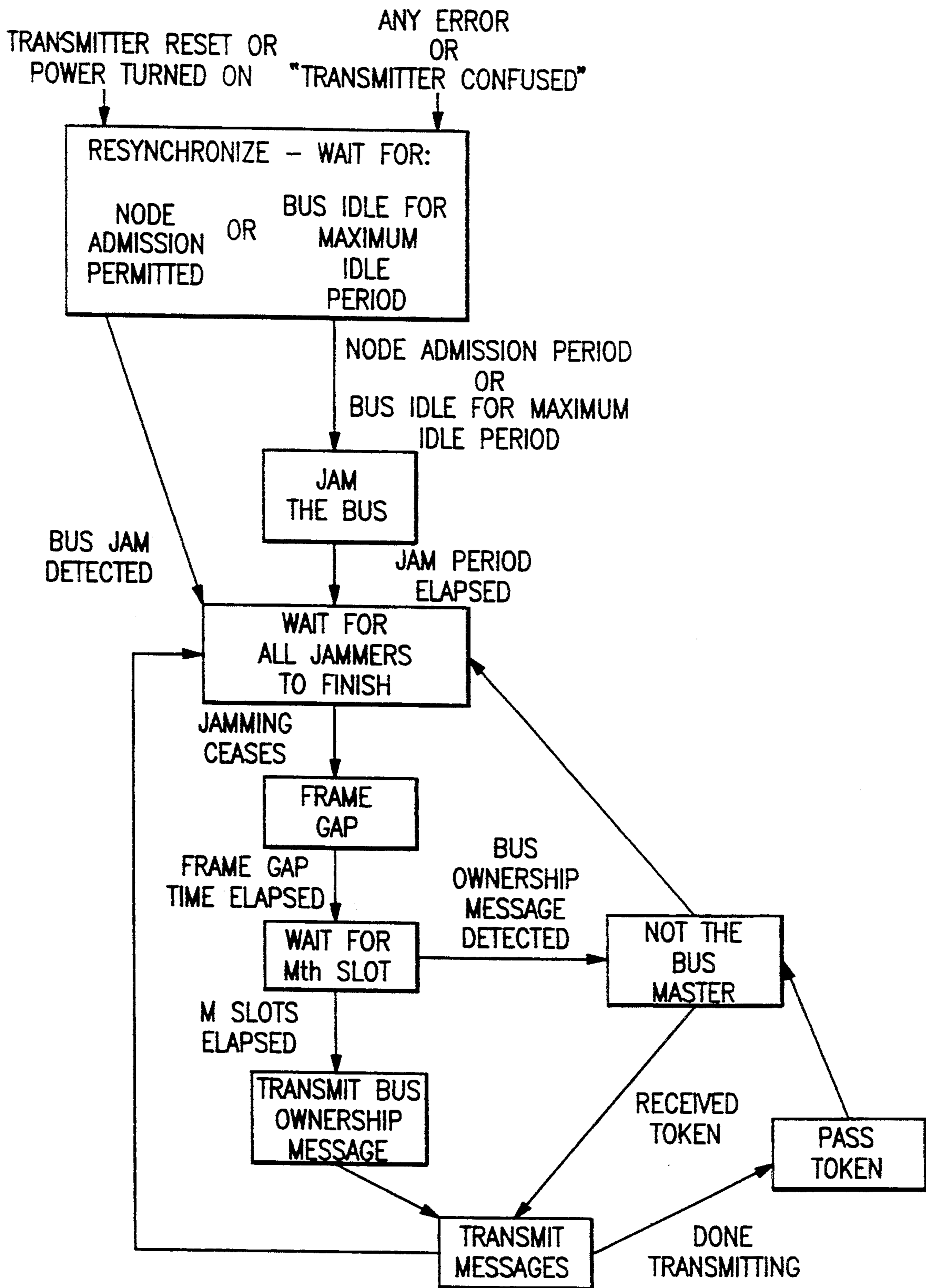
FSD FOR EXPLICIT TOKEN BUS PROTOCOL.
