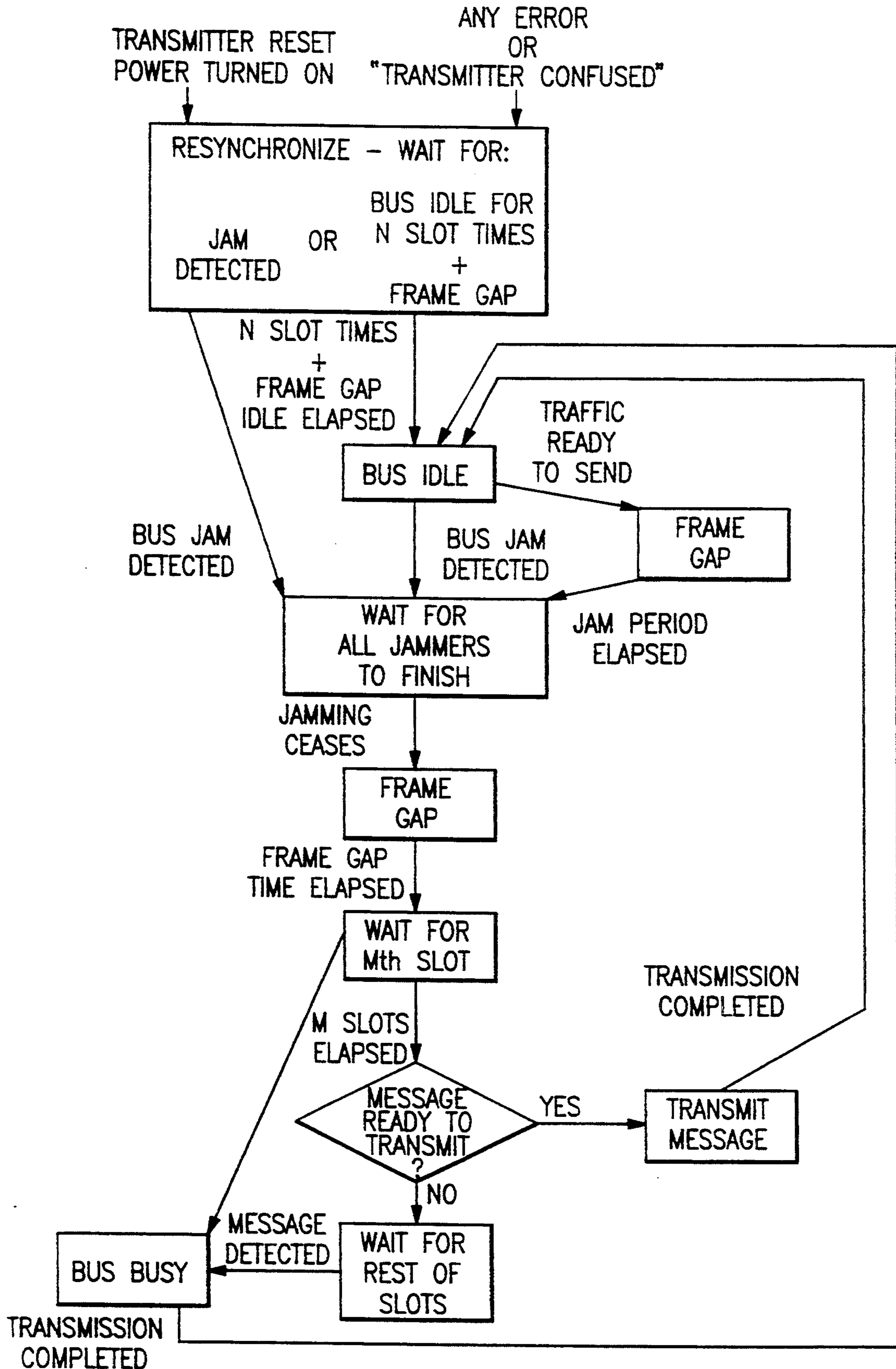
FSD FOR RESERVATION CSMA PROTOCOL WITH PER-MESSAGE RESTART.
