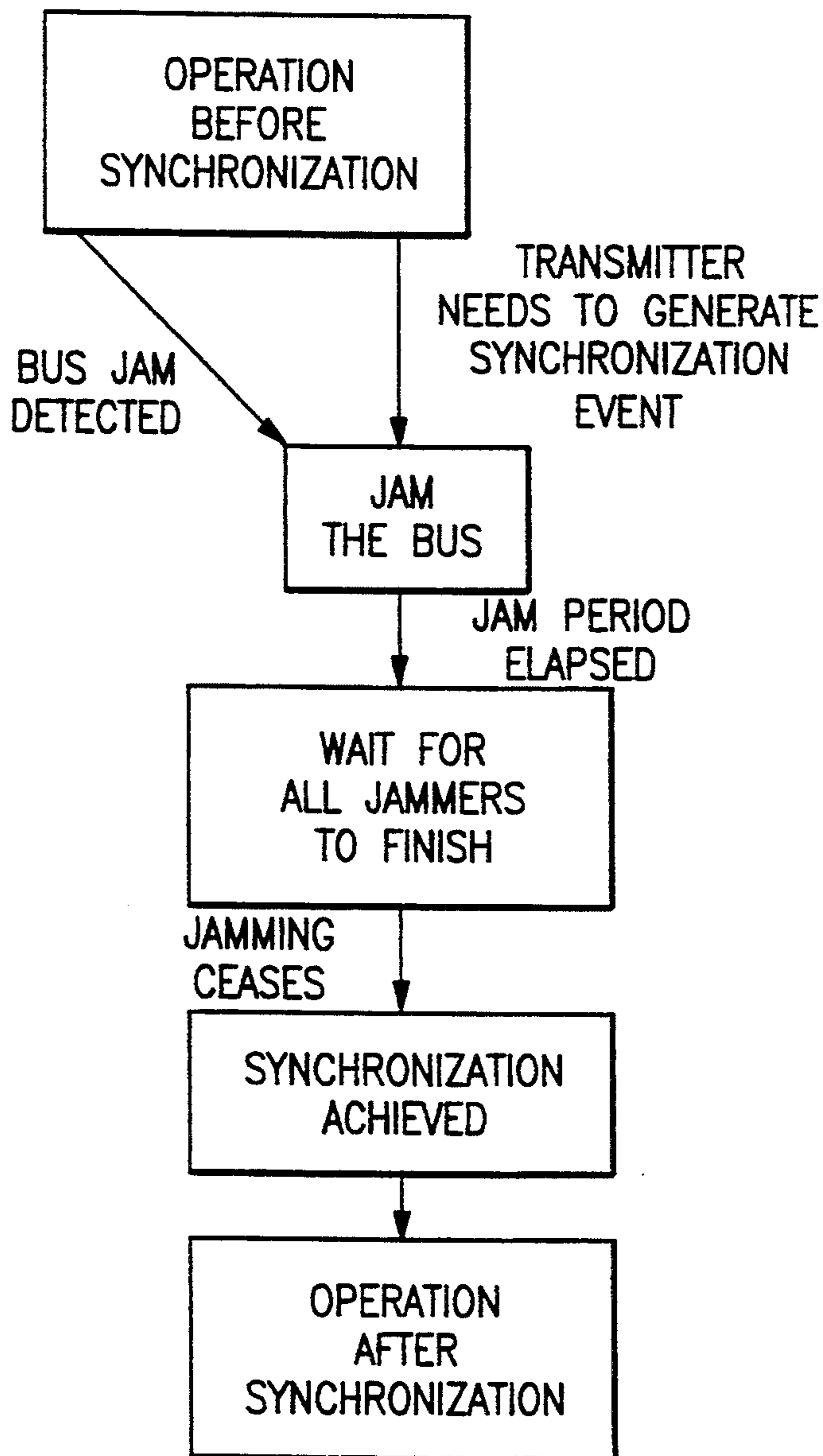
FSD FOR SYNCHRONIZATION OF MULTIPLE TRANSMITTERS.
