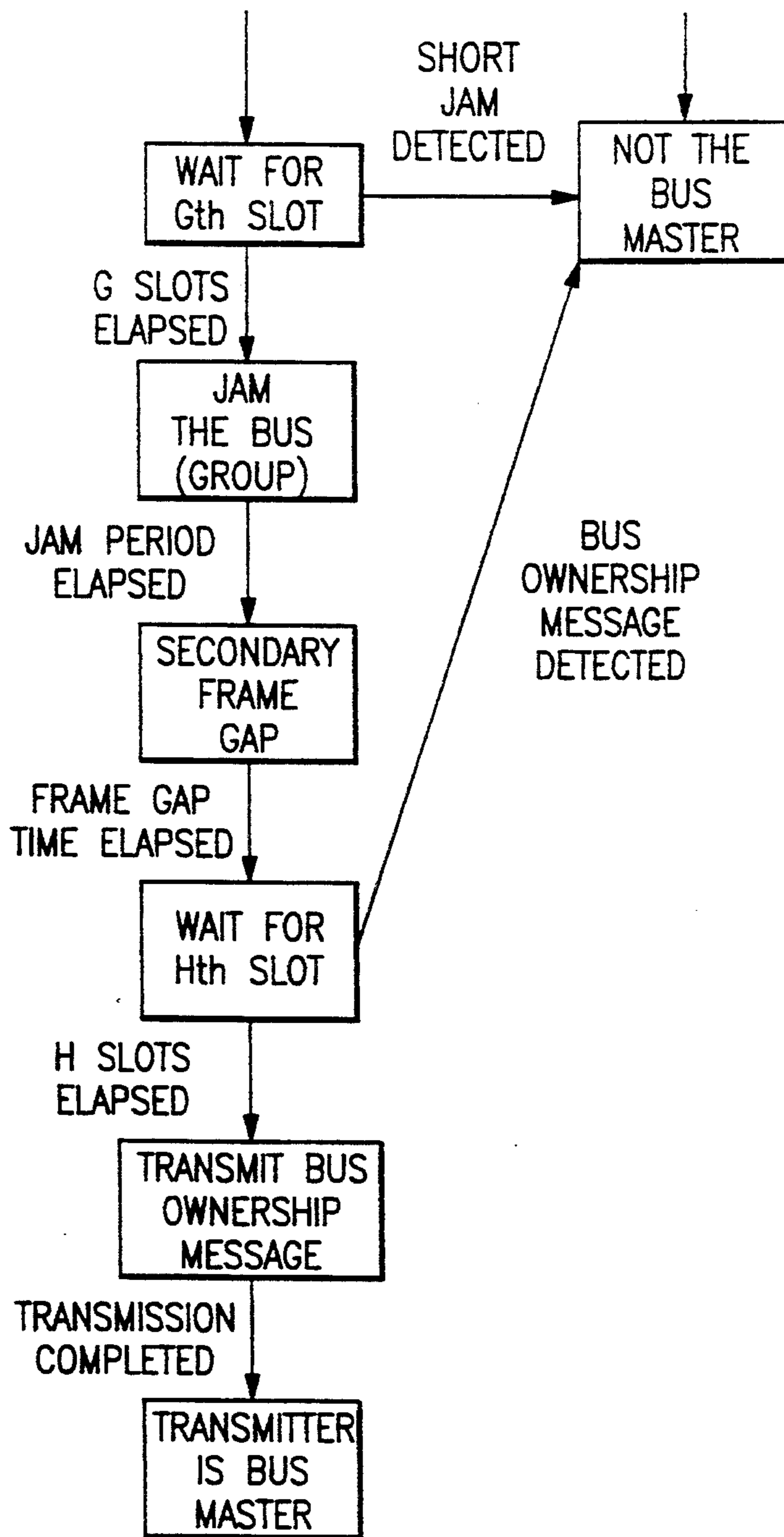
FSD FOR MULTI-LEVEL BUS MASTER ARBITRATION.
