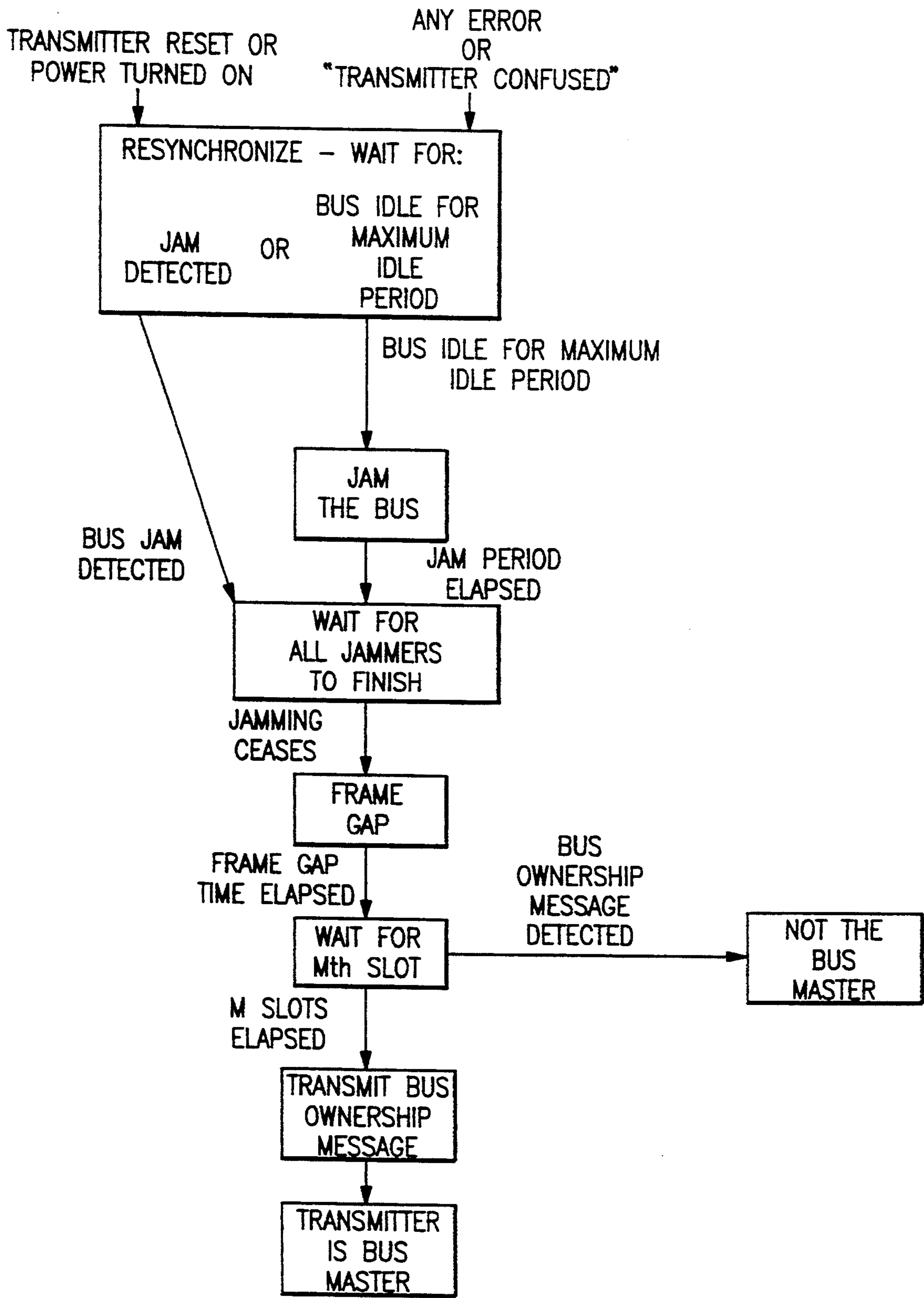
FSD FOR BUS MASTER ARBITRATION.
