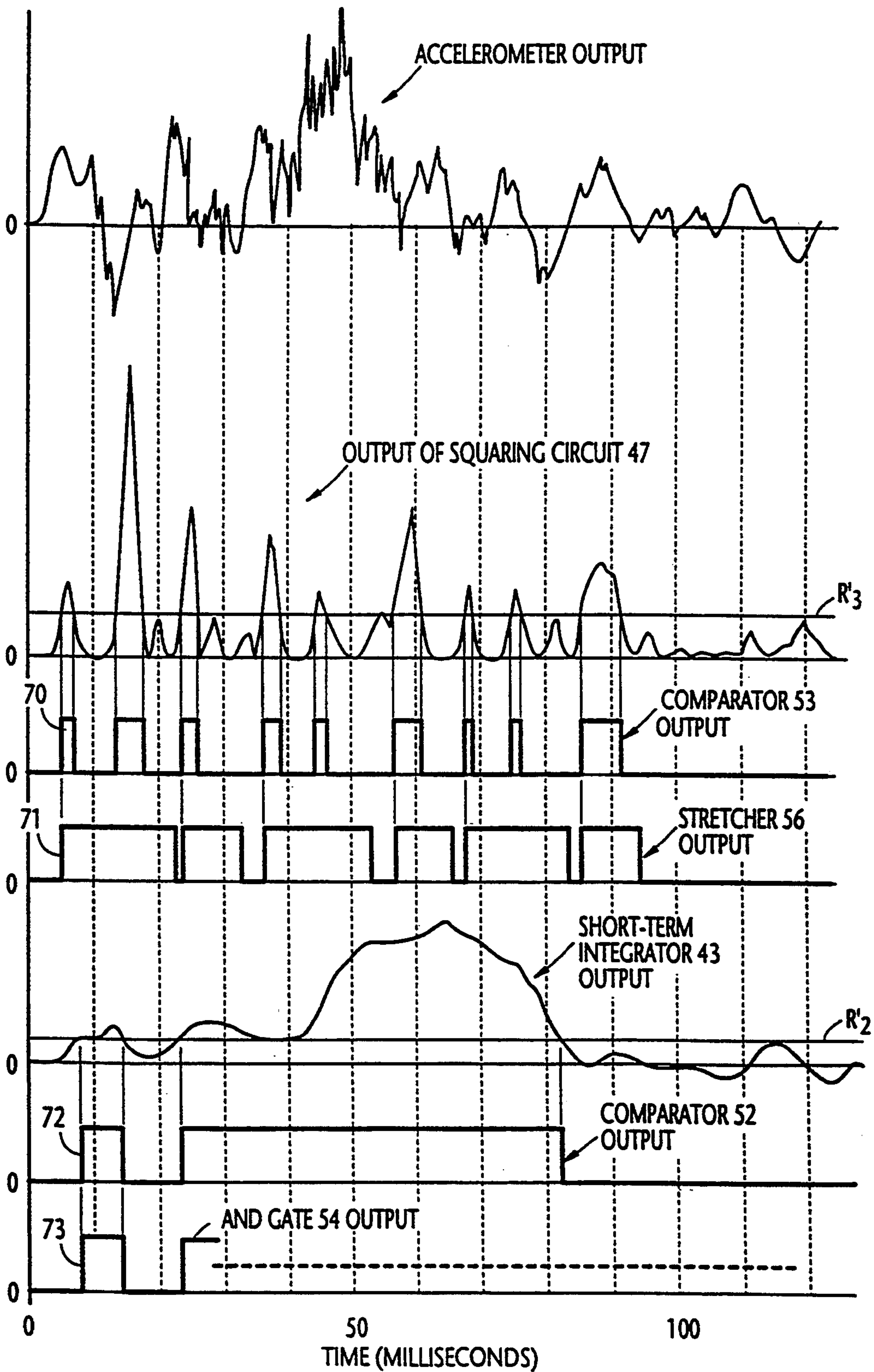
FIG. 9 FRONTAL CRASH
