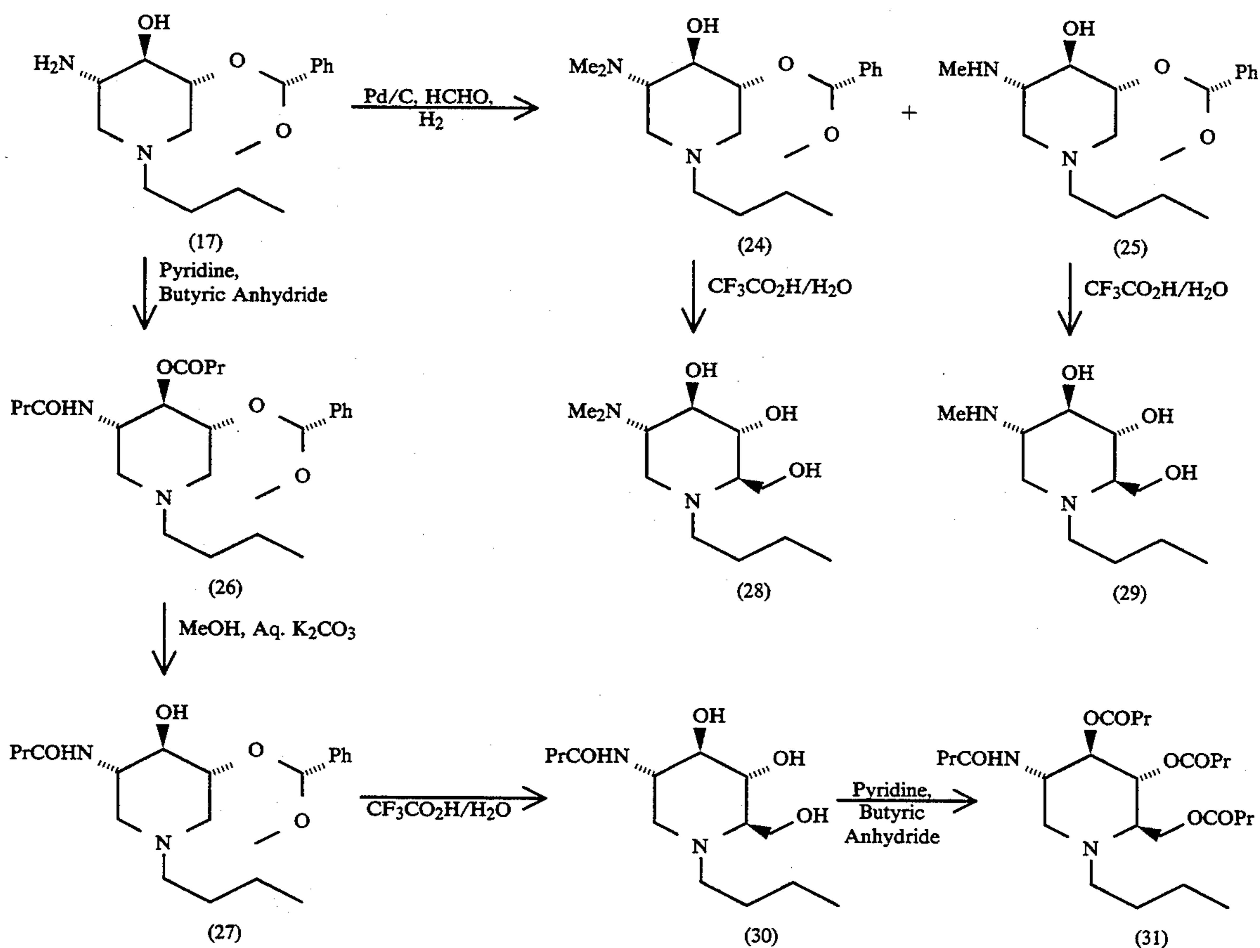
Scheme C: Synthesis of 2-alkylamino &amp; 2-acylamido 1,5-iminosugars.
