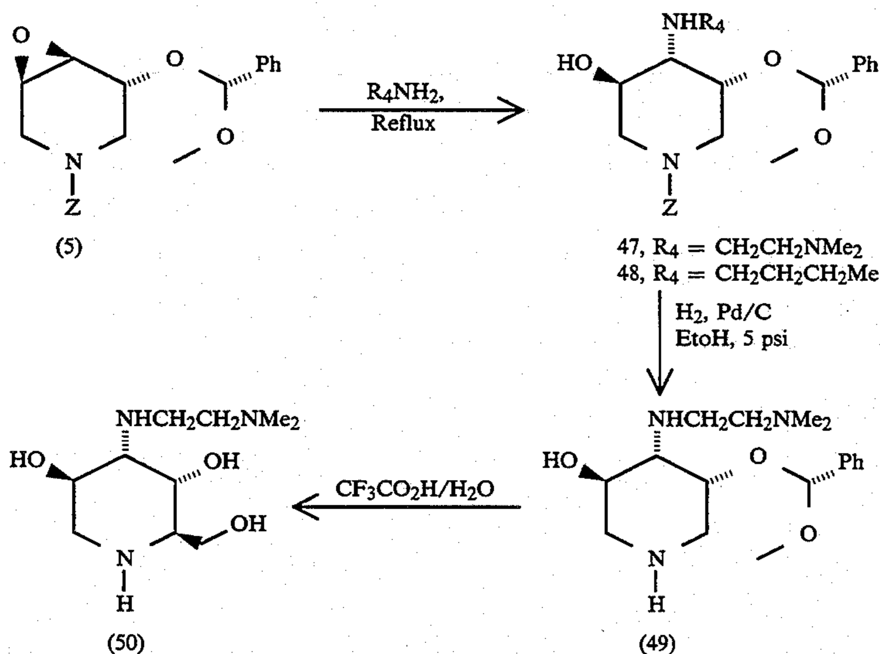
Scheme H: Synthesis of 3-amino 1,5-iminosugars.
