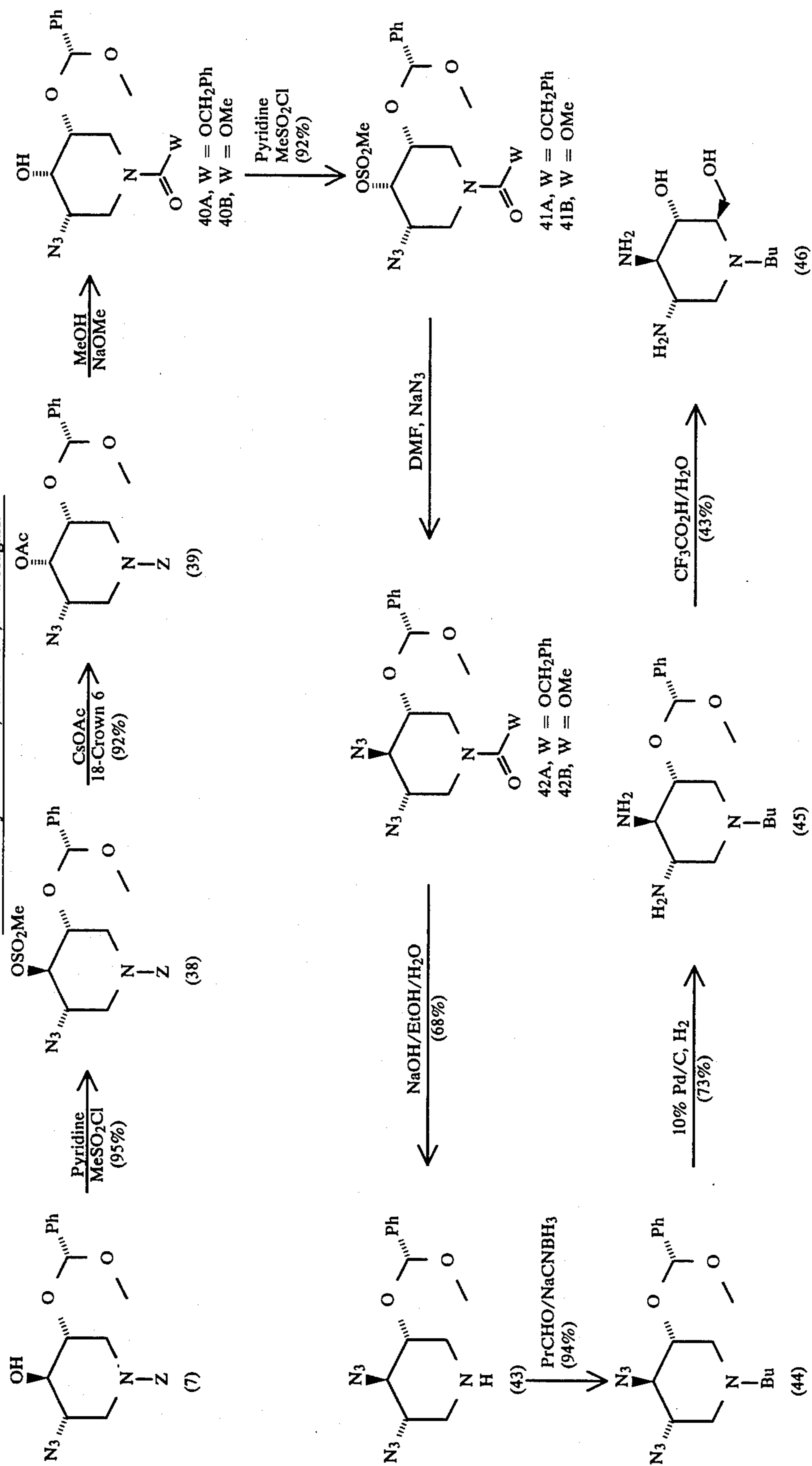
Scheme G: Synthesis of 2,3-diamino-1,5-iminosugars.
