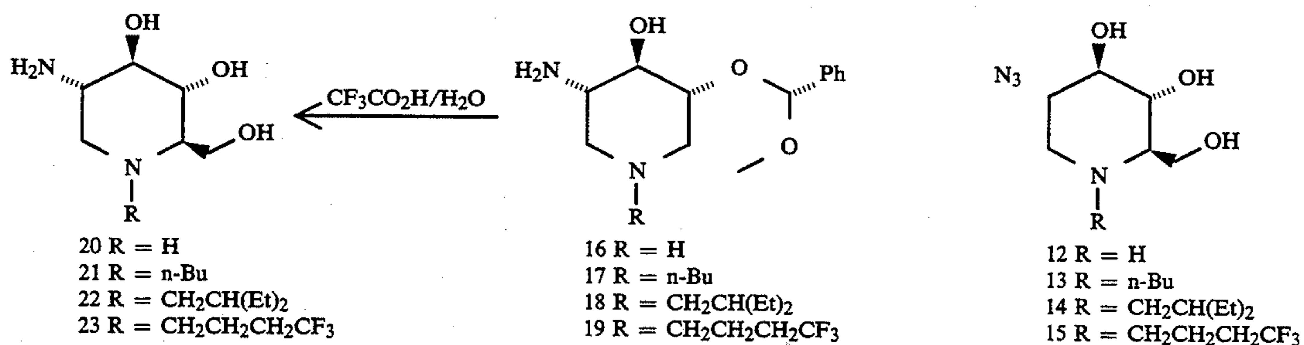
Scheme B: Synthesis of 2-azido and 2-amino 1,5-iminosugars.
