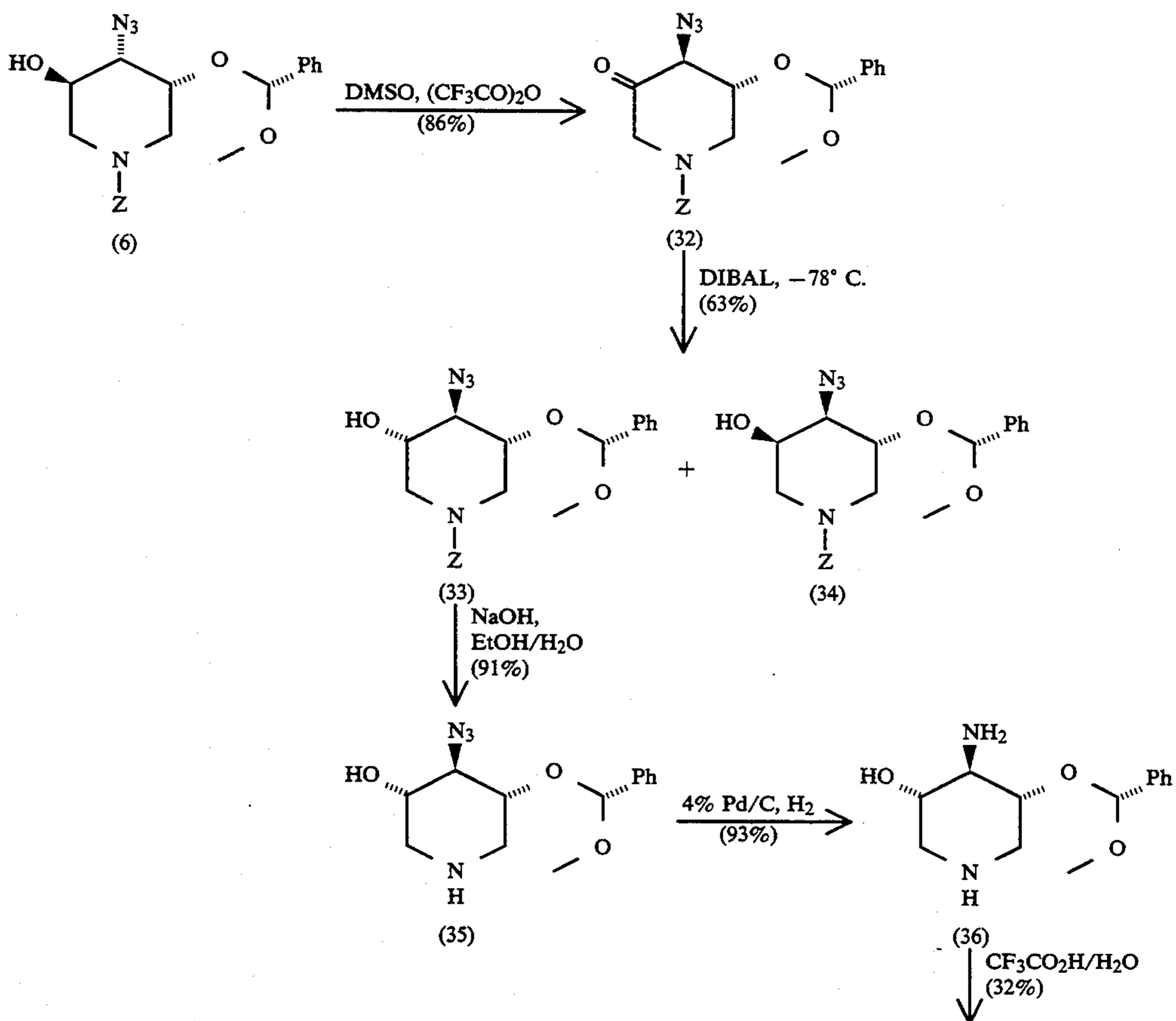
Scheme E: Synthesis of 3-amino-1,5-iminosugars.
