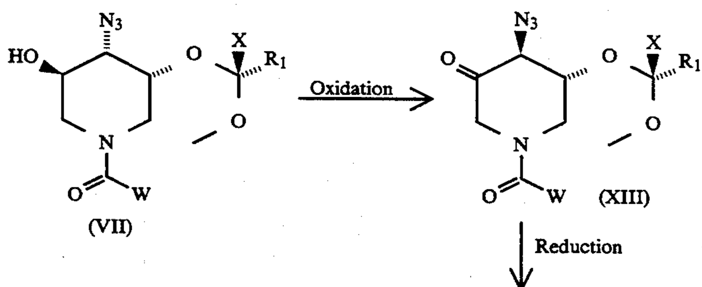
Scheme D: Generic Synthesis of 3-azido- &amp; 3-amino-1,5-iminosugar
