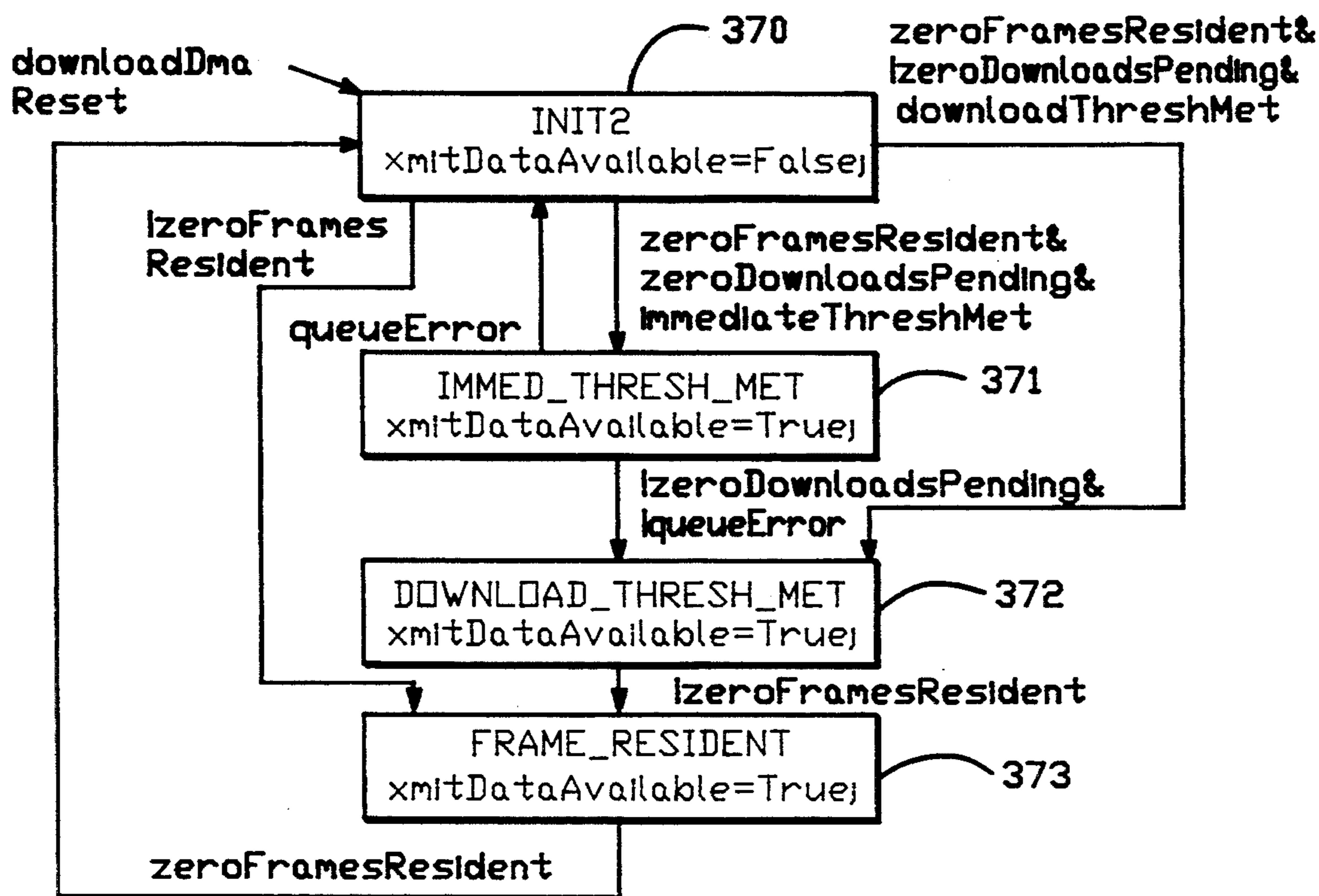
DataAvailableControlStateDiagram
