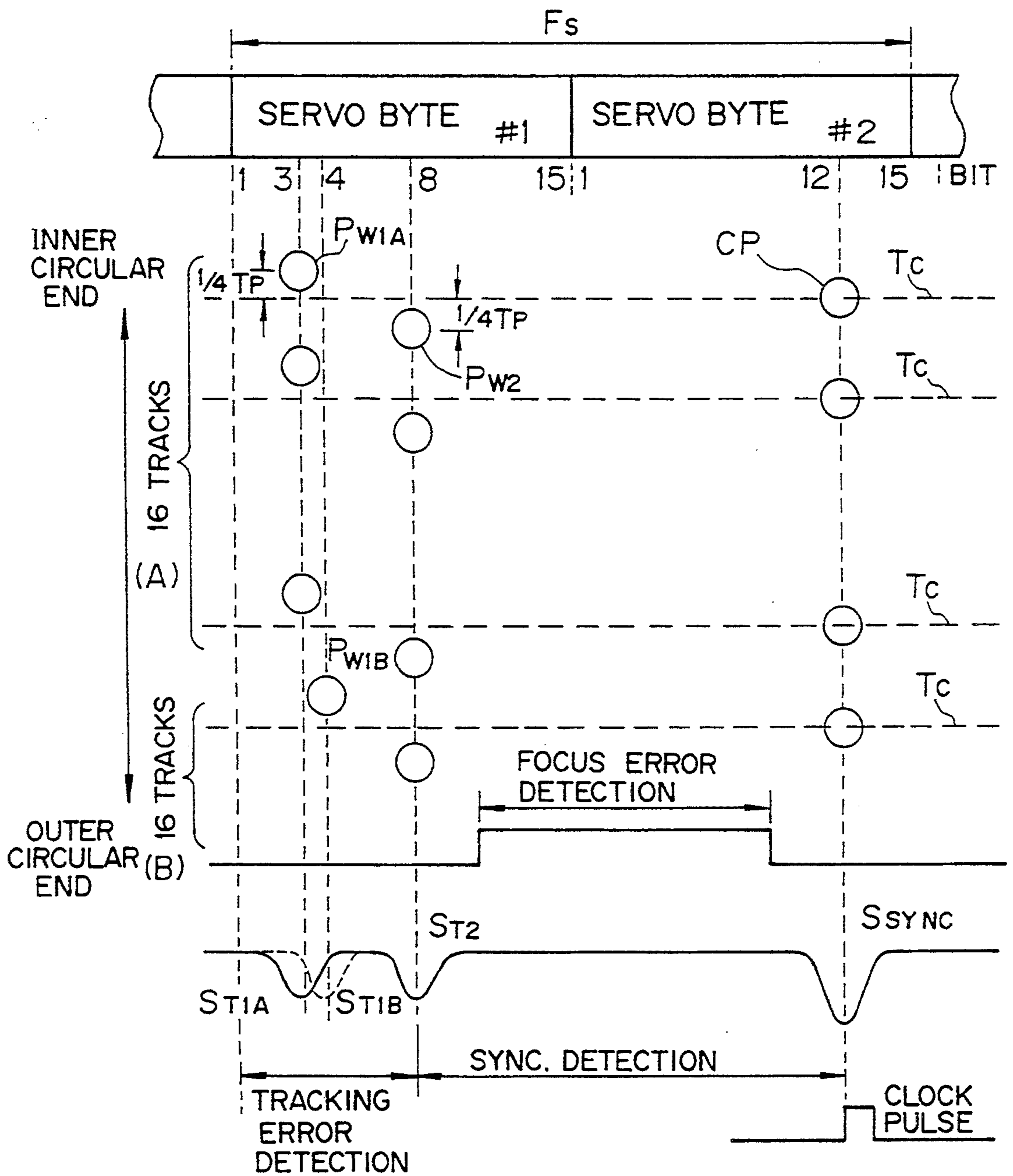
FIG. 2 PRIOR ART
