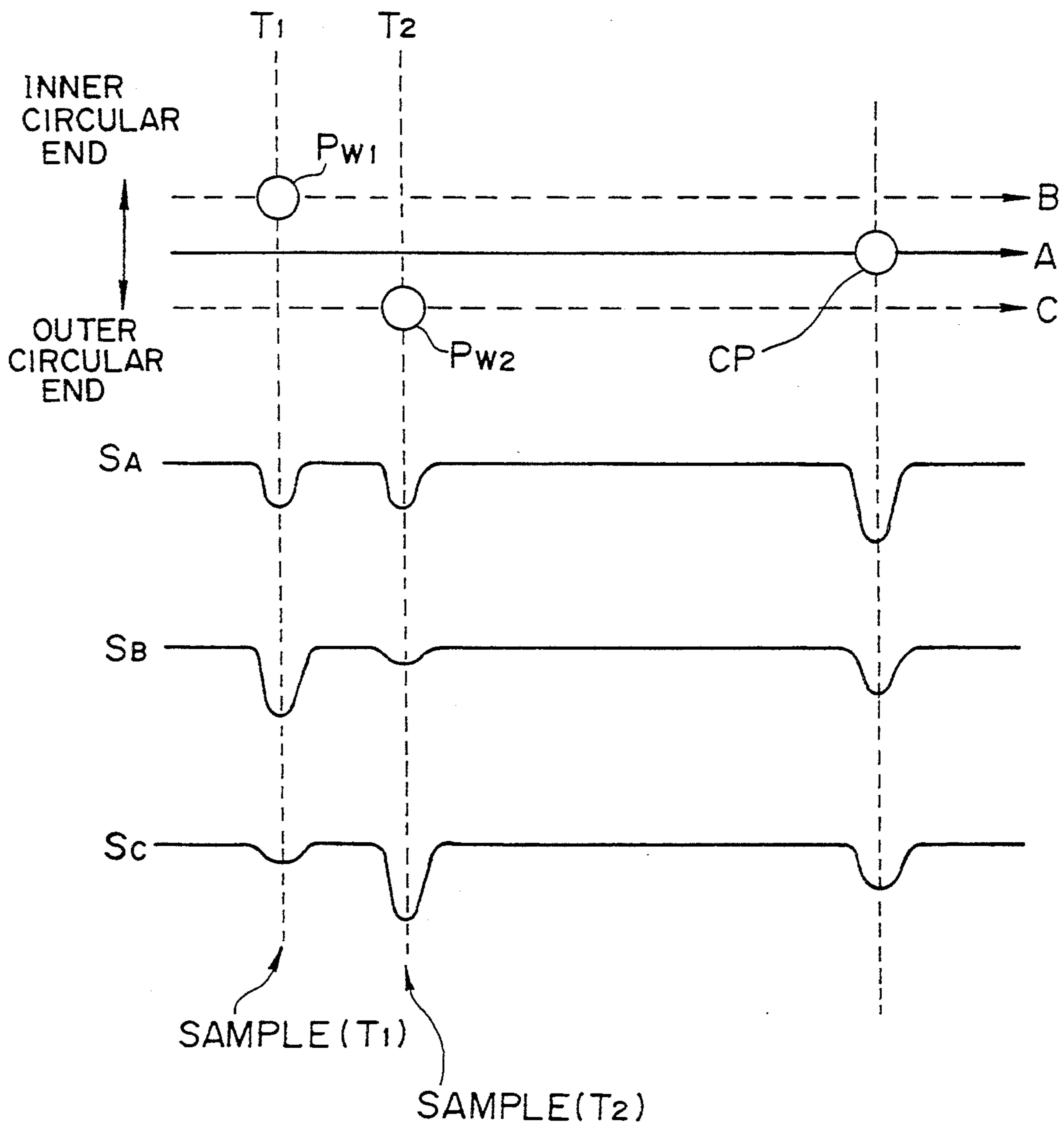
FIG. 3 PRIOR ART
