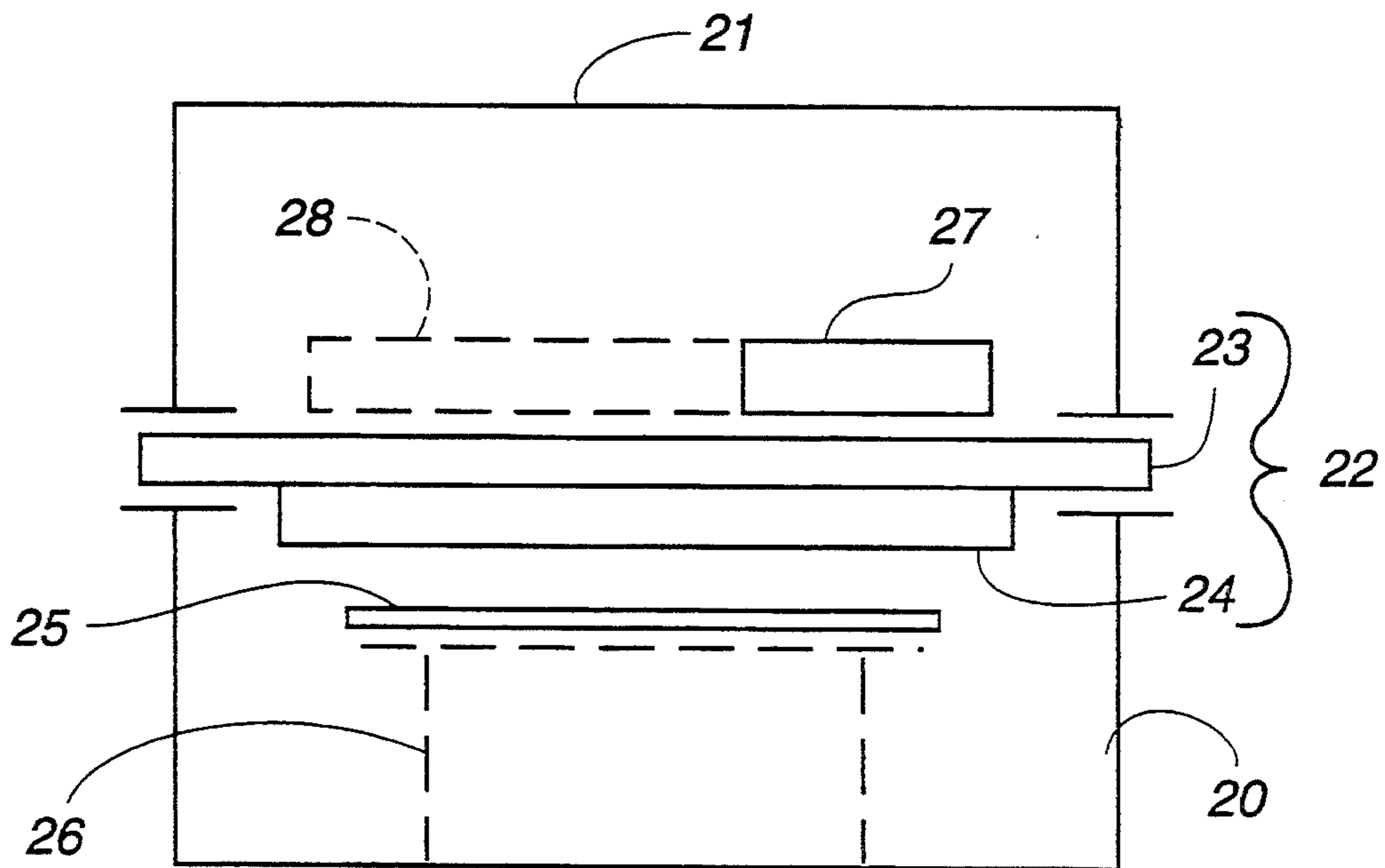
Fig. 1 (PRIOR ART)
