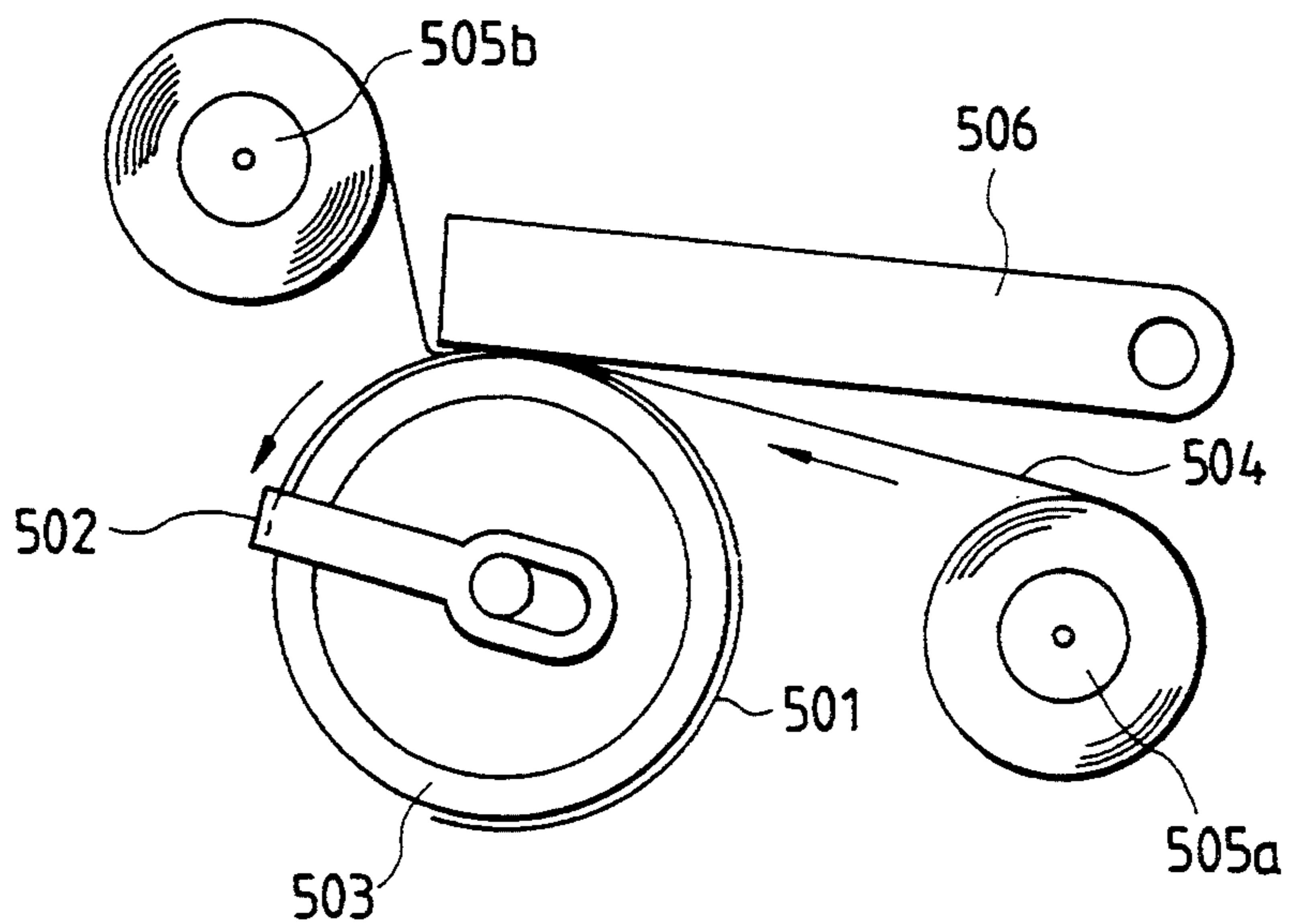
FIG. 25 PRIOR ART
