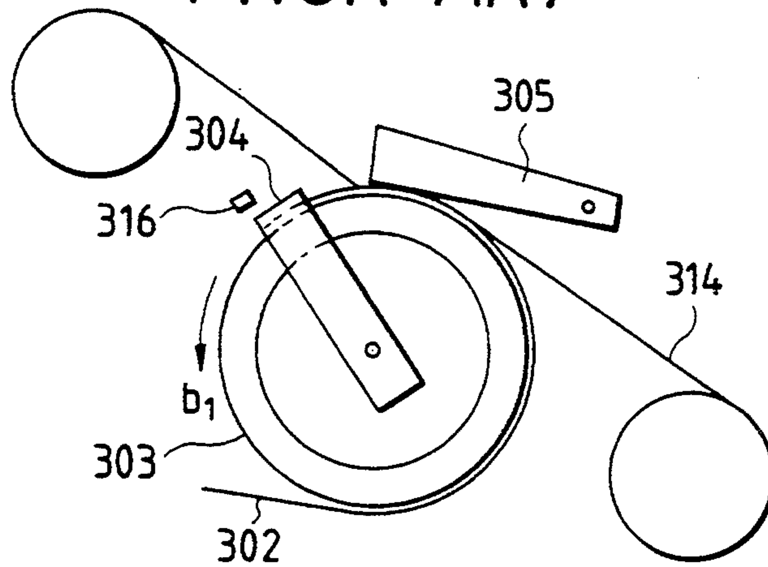
FIG. 18 PRIOR ART
