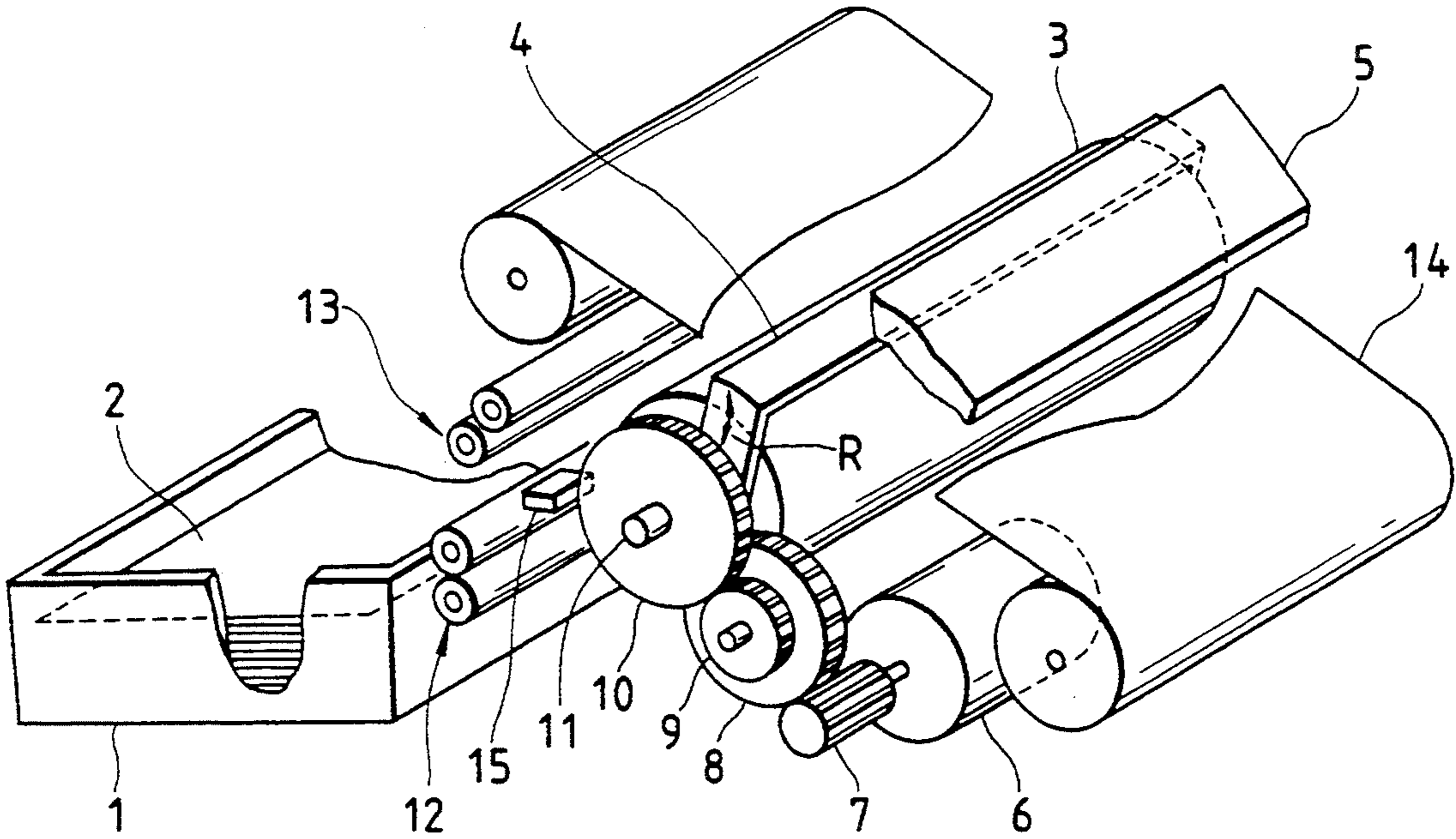
FIG. 1 PRIOR ART
