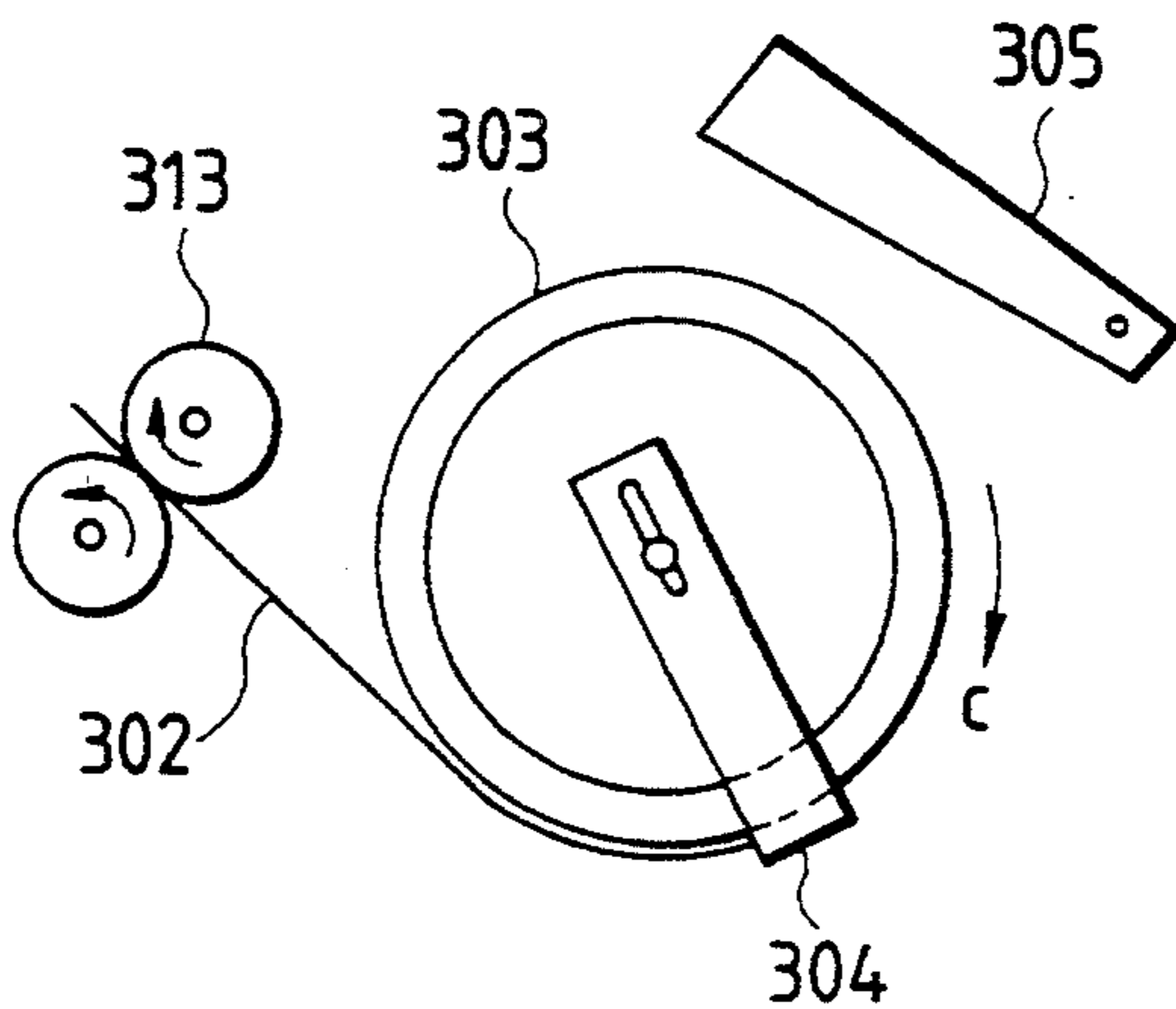
FIG. 18 PRIOR ART
