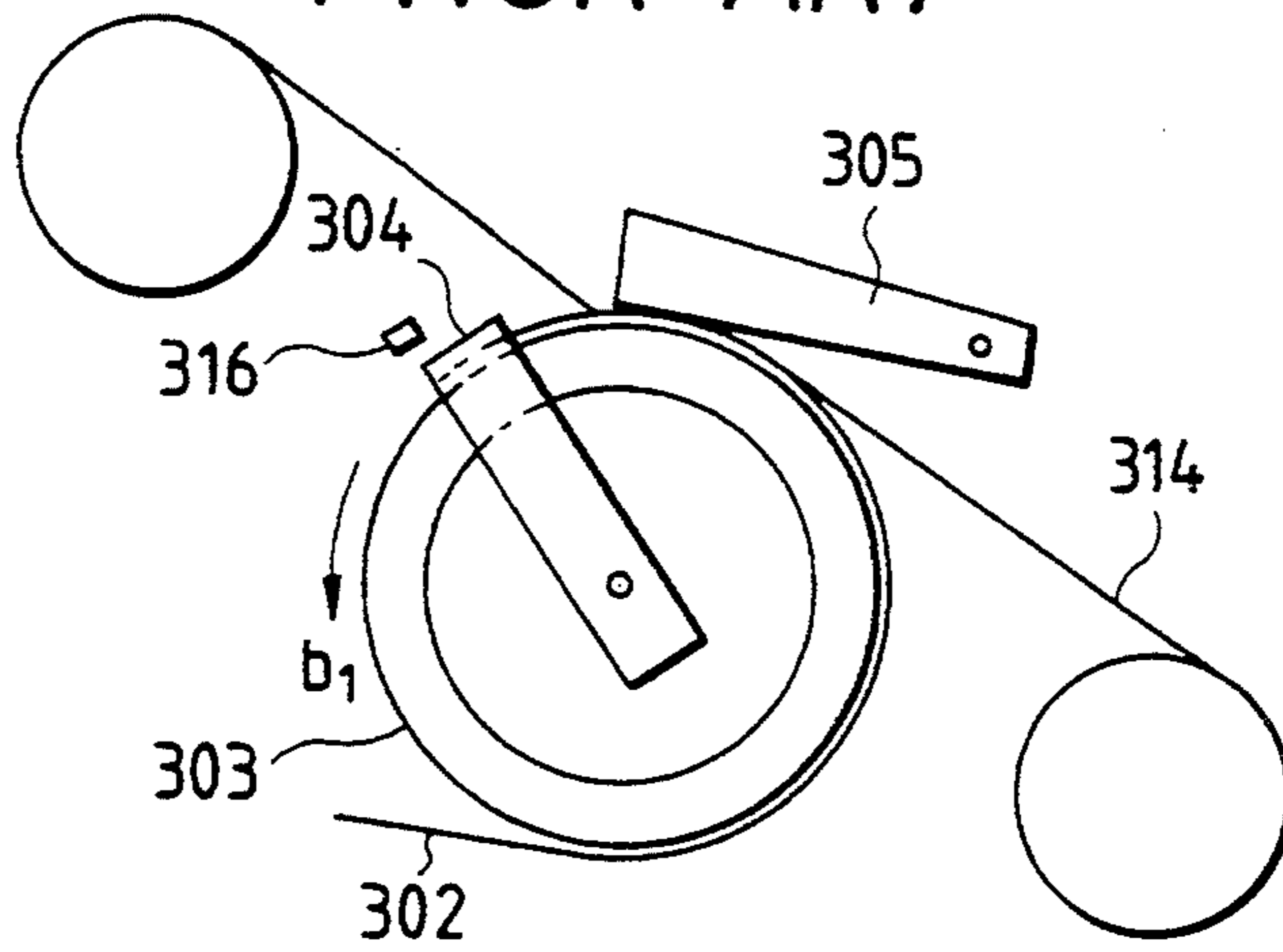
FIG. 18 PRIOR ART
