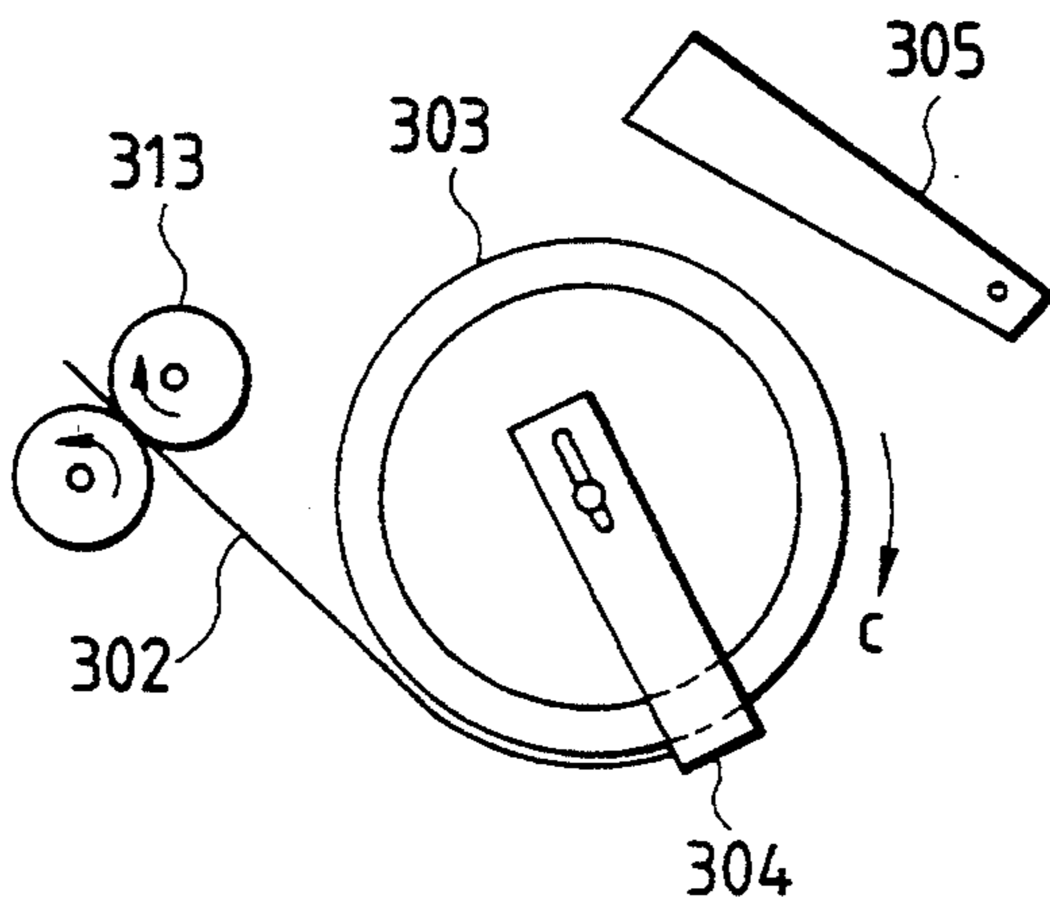
FIG. 18 PRIOR ART
