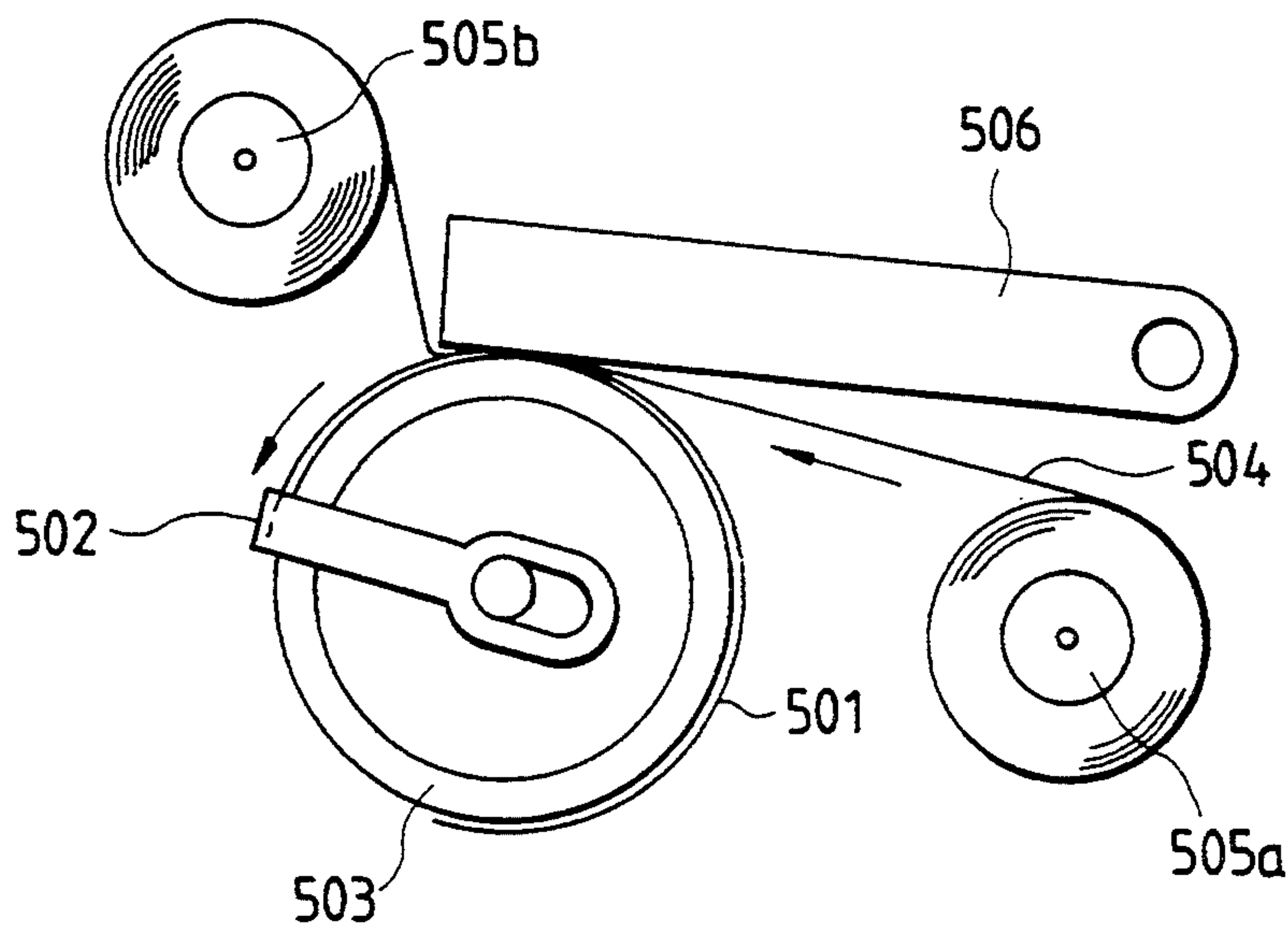
FIG. 25 PRIOR ART
