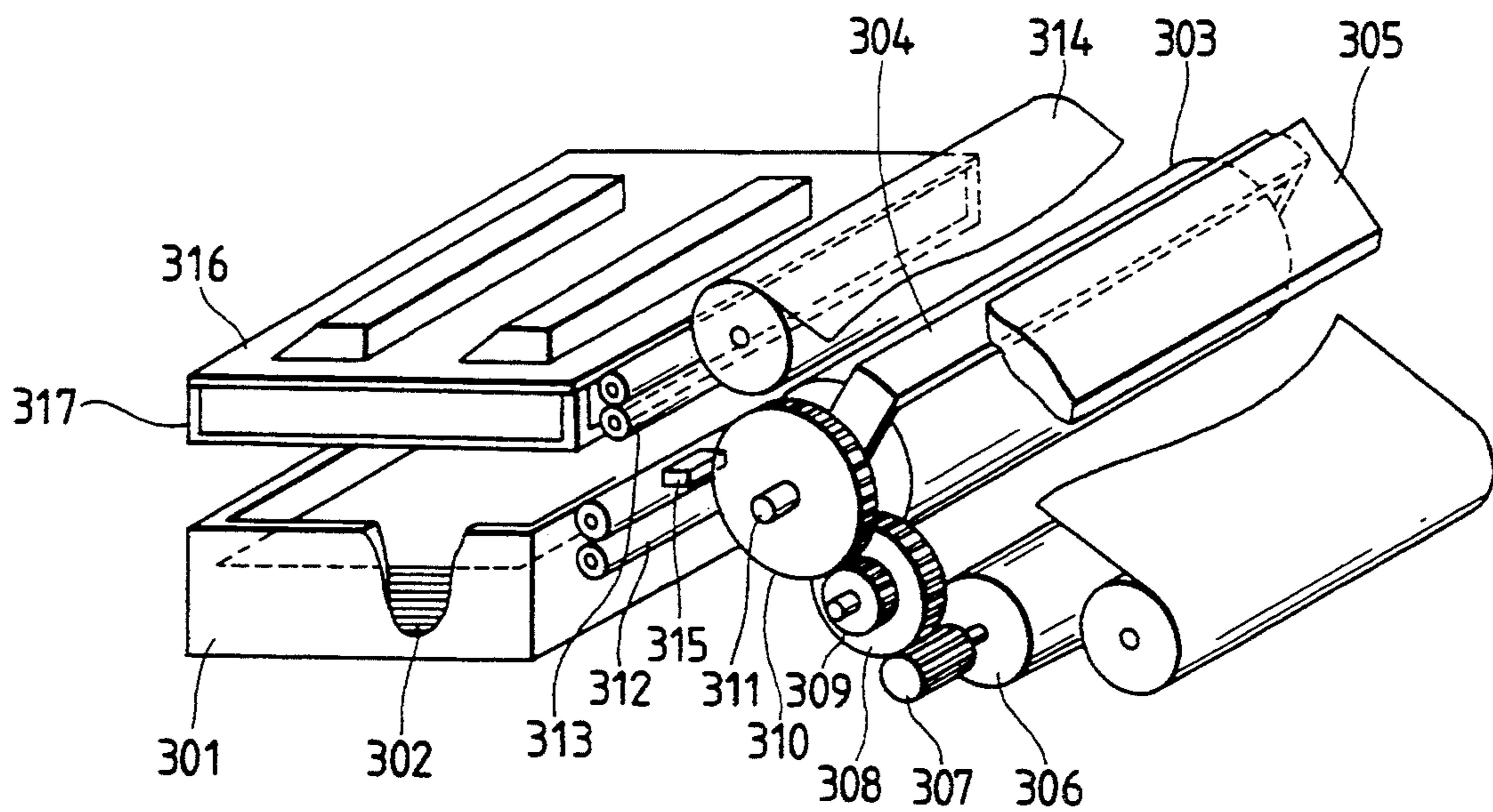
FIG. 14 PRIOR ART
