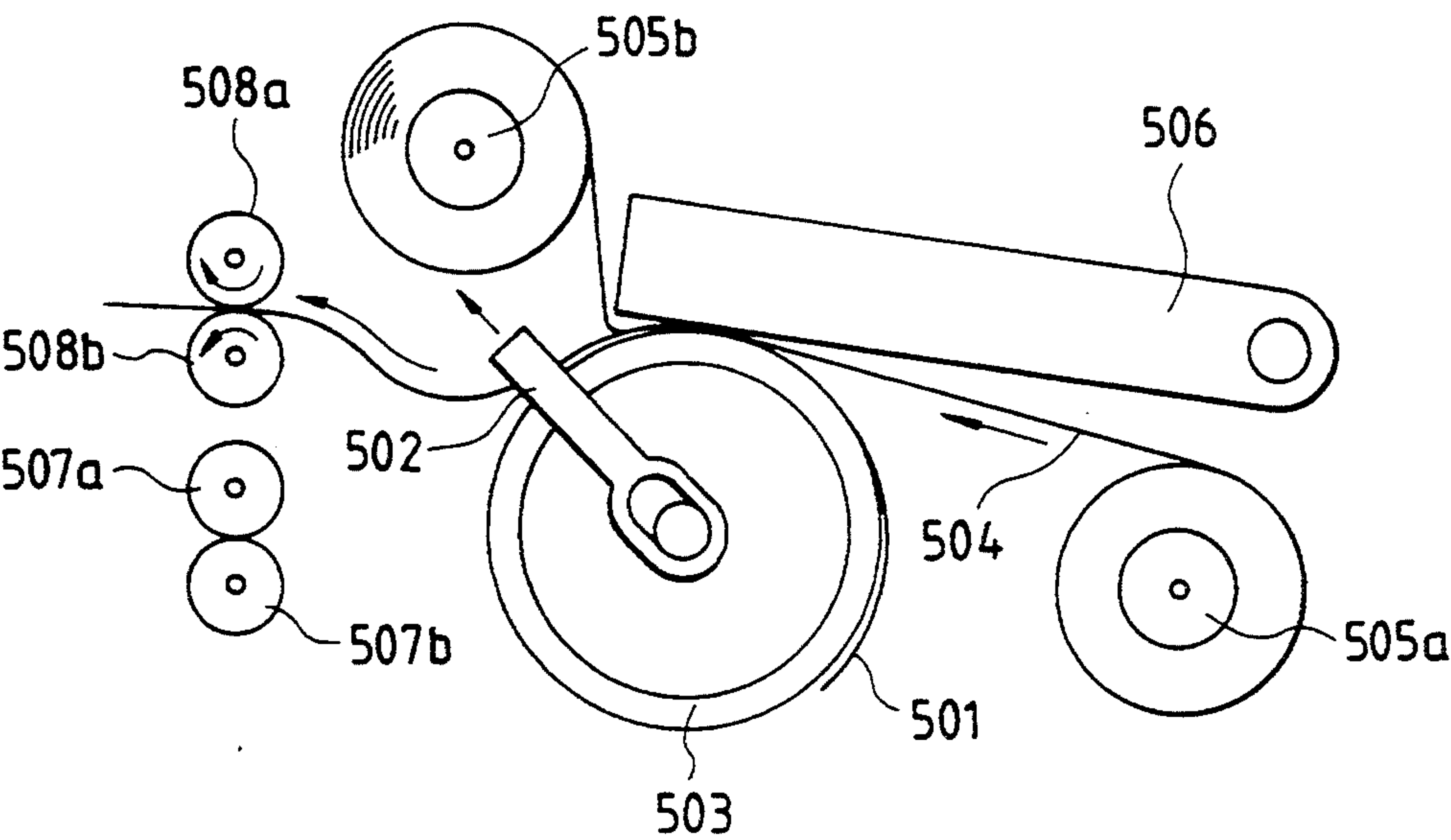
FIG. 27 PRIOR ART
