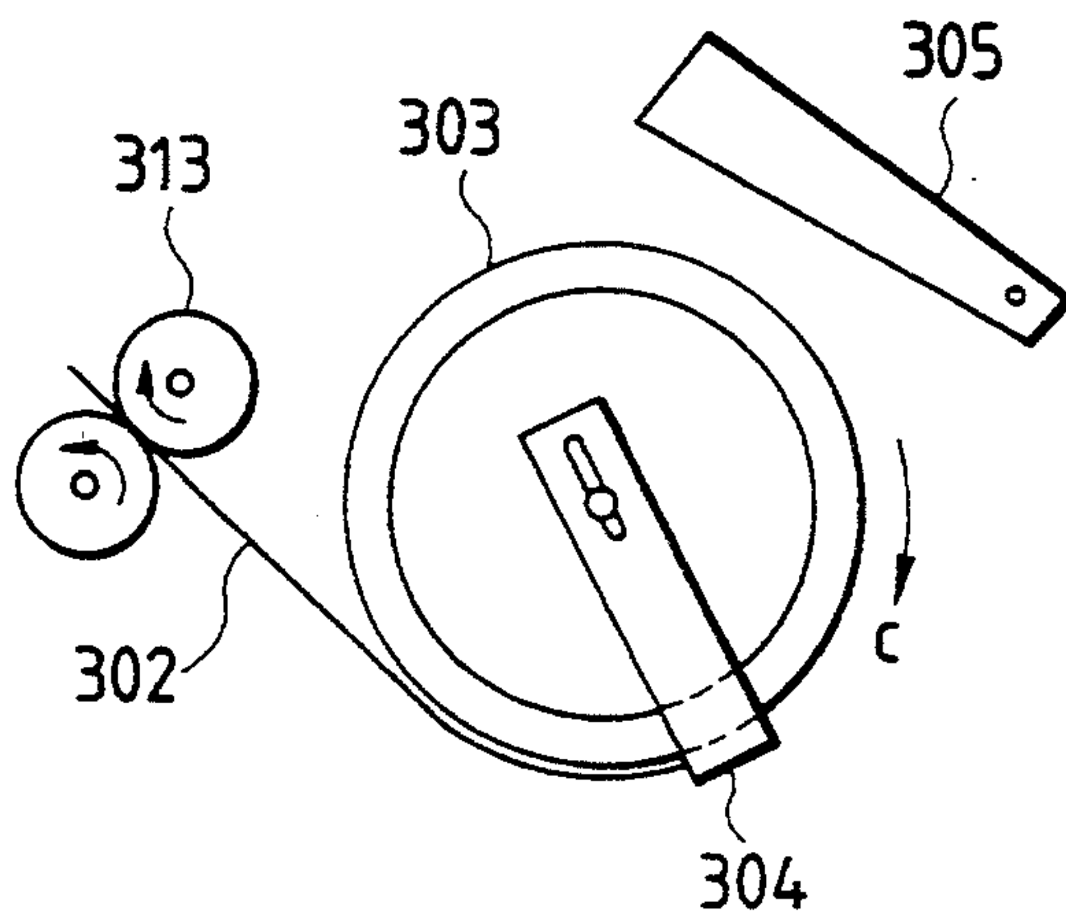
FIG. 18 PRIOR ART
