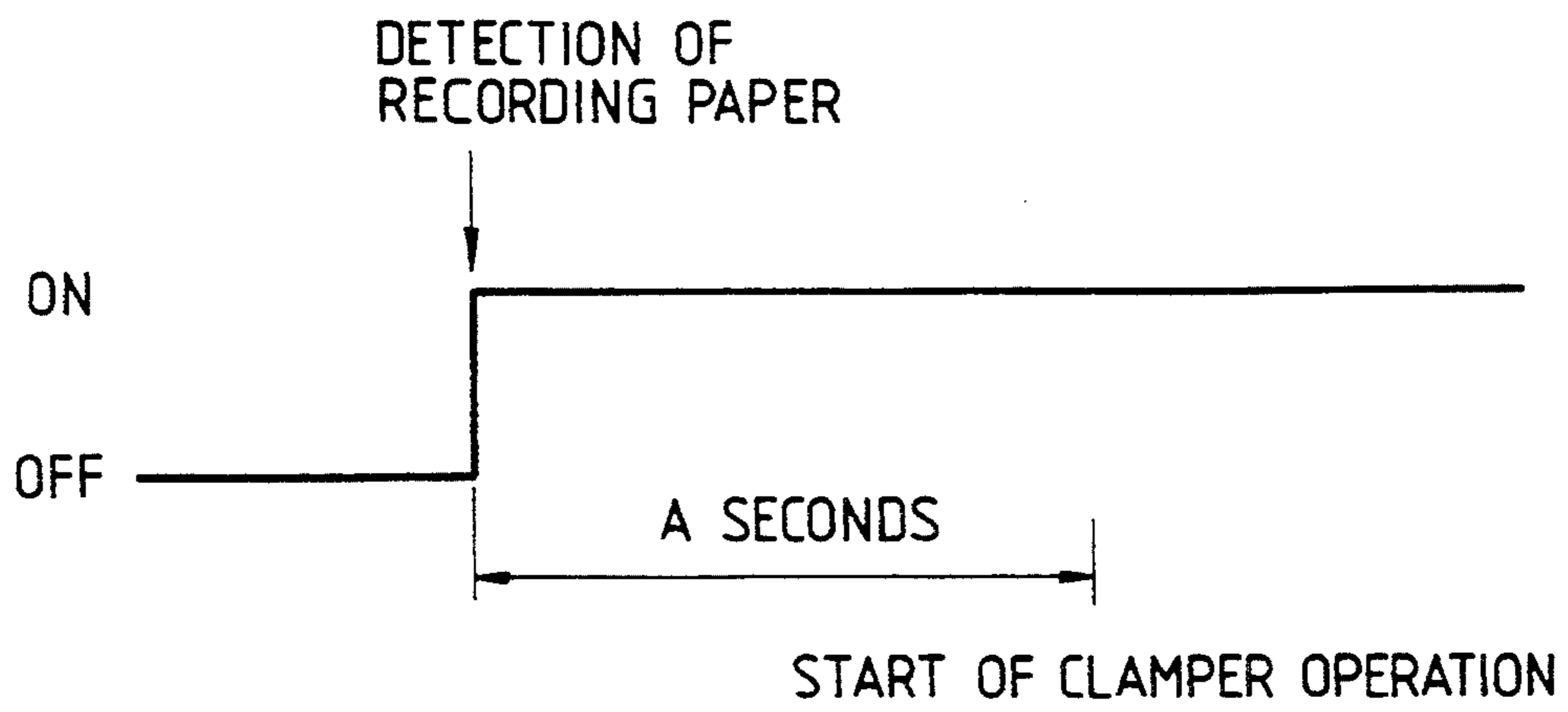
FIG. 20 PRIOR ART
