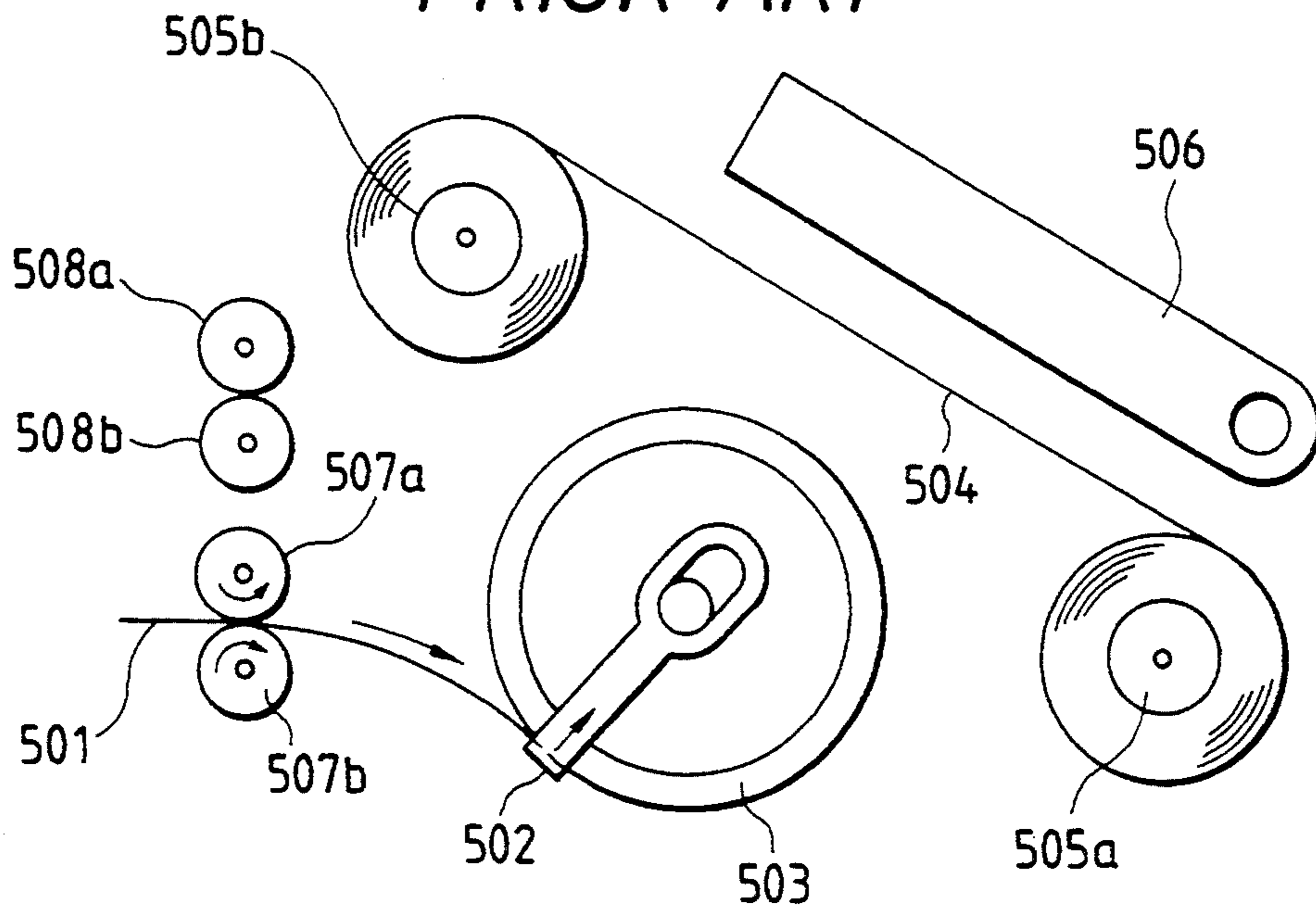
FIG. 24 PRIOR ART
