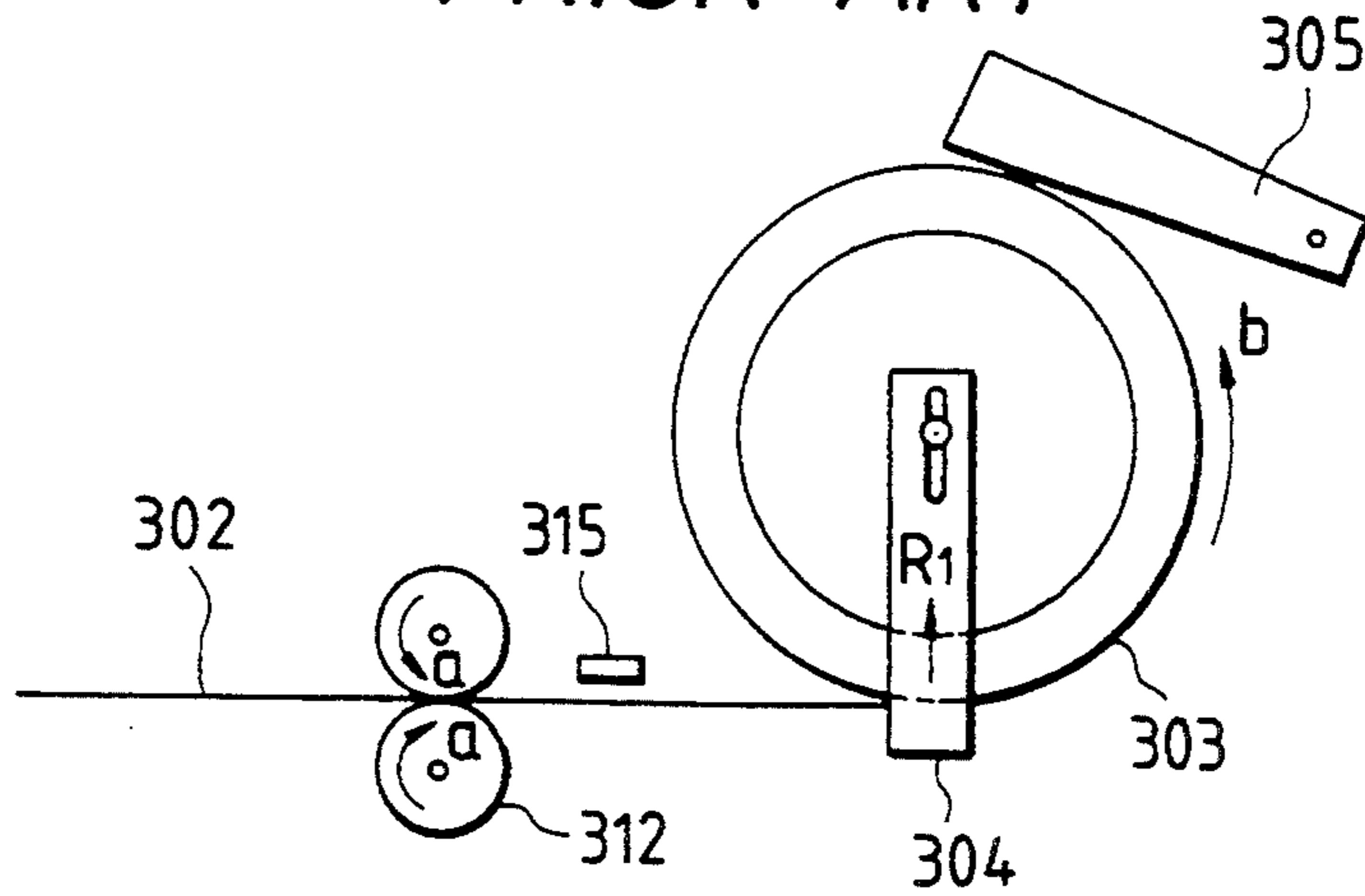
FIG. 17 PRIOR ART
