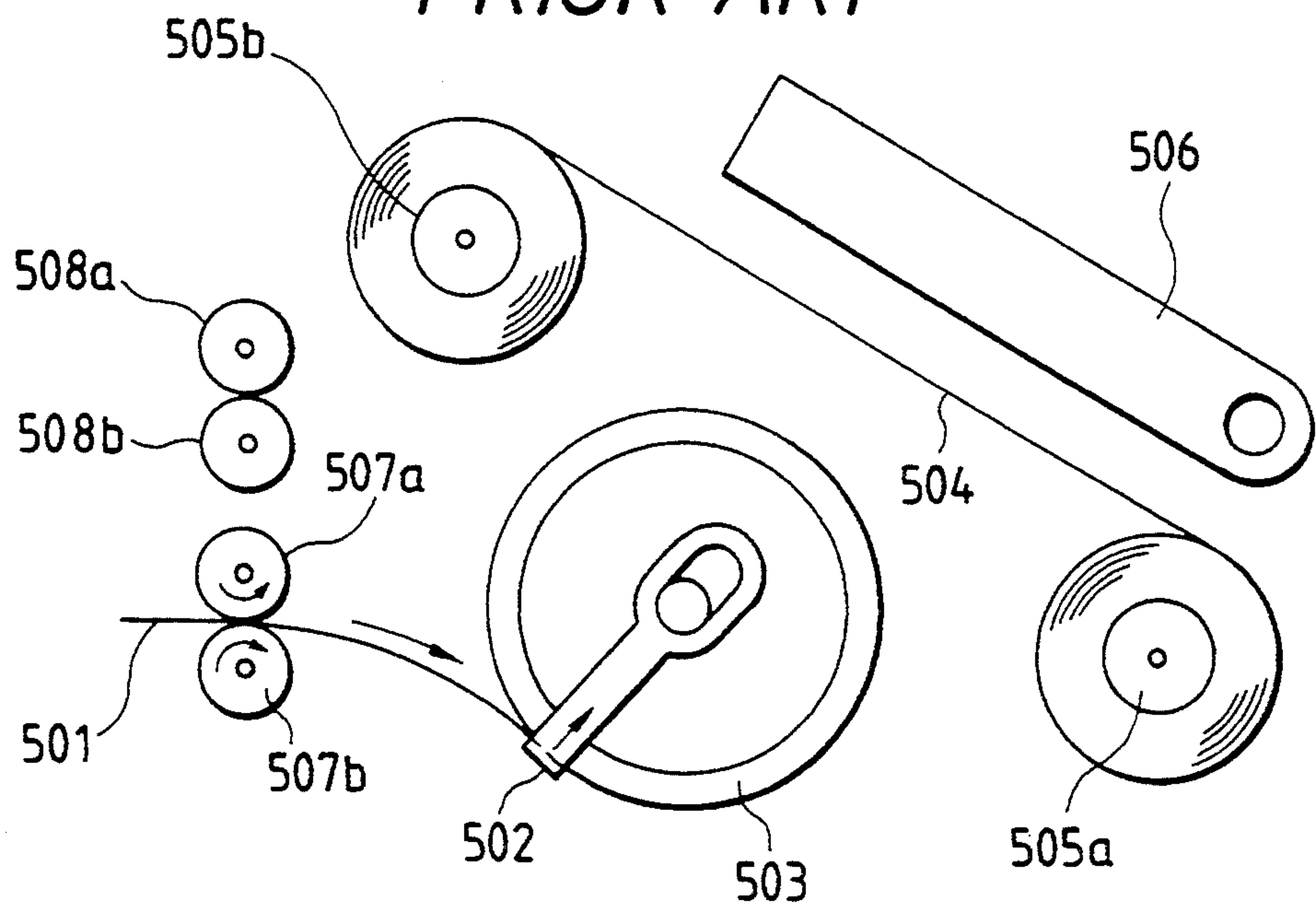
FIG. 24 PRIOR ART
