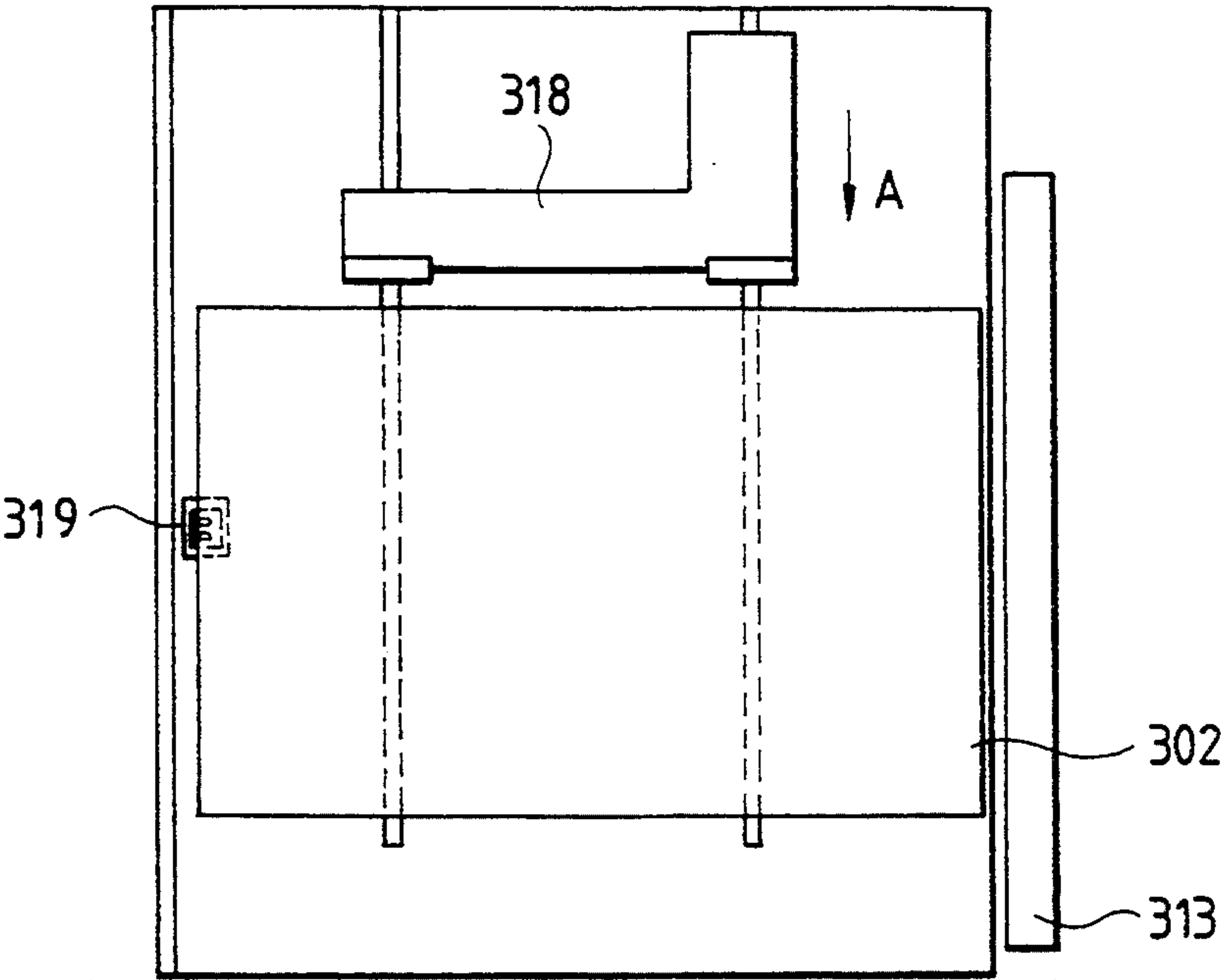
FIG. 21 PRIOR ART
