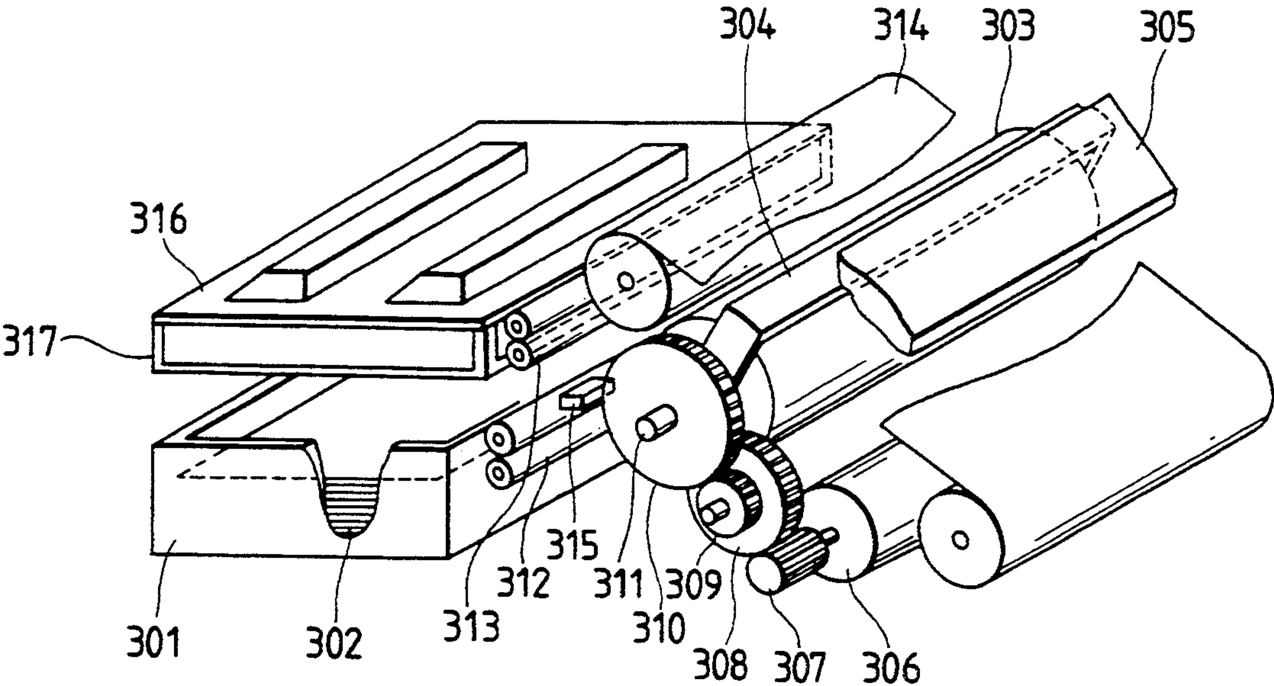
FIG. 14 PRIOR ART
