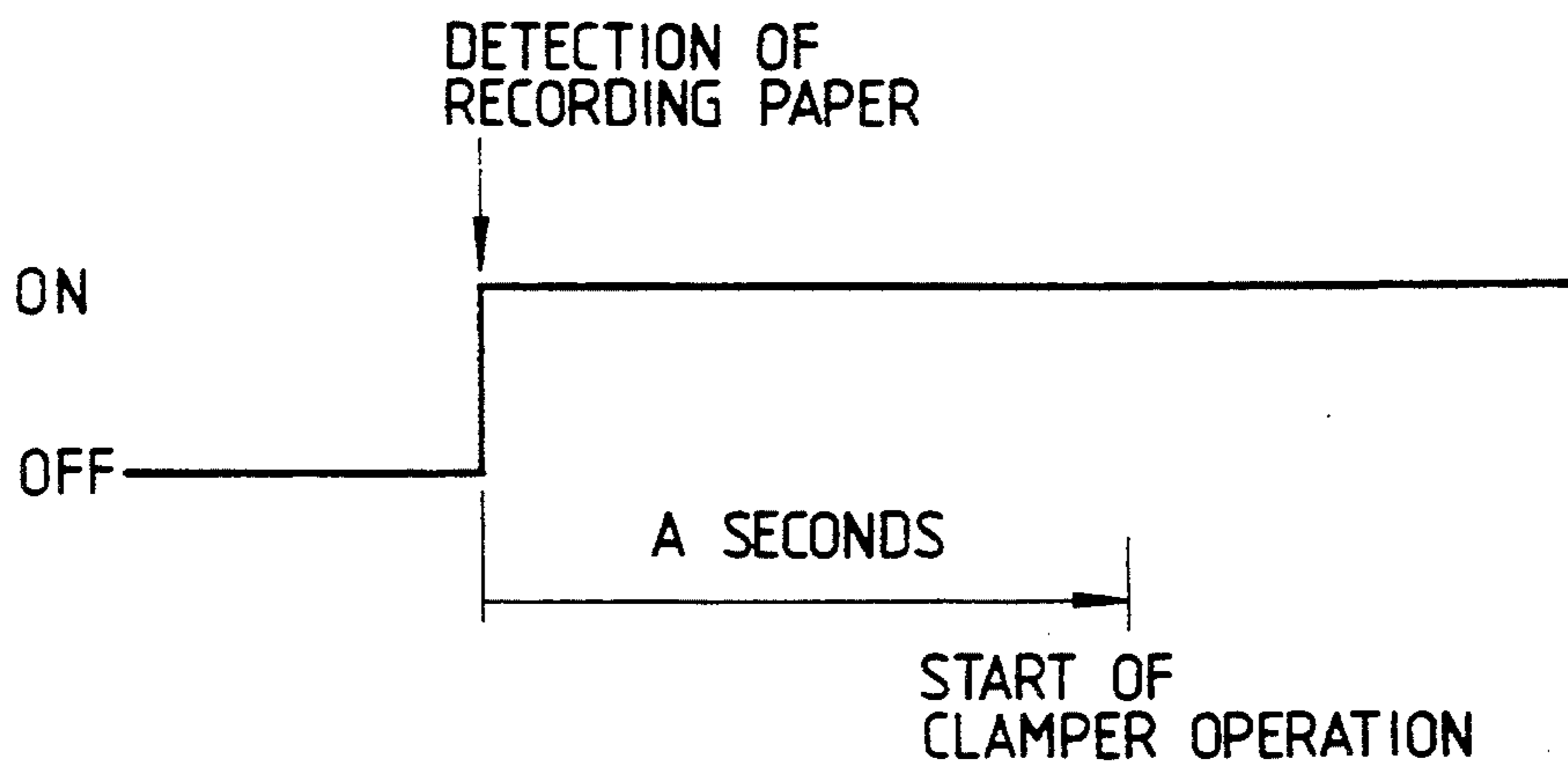
FIG. 5 PRIOR ART
