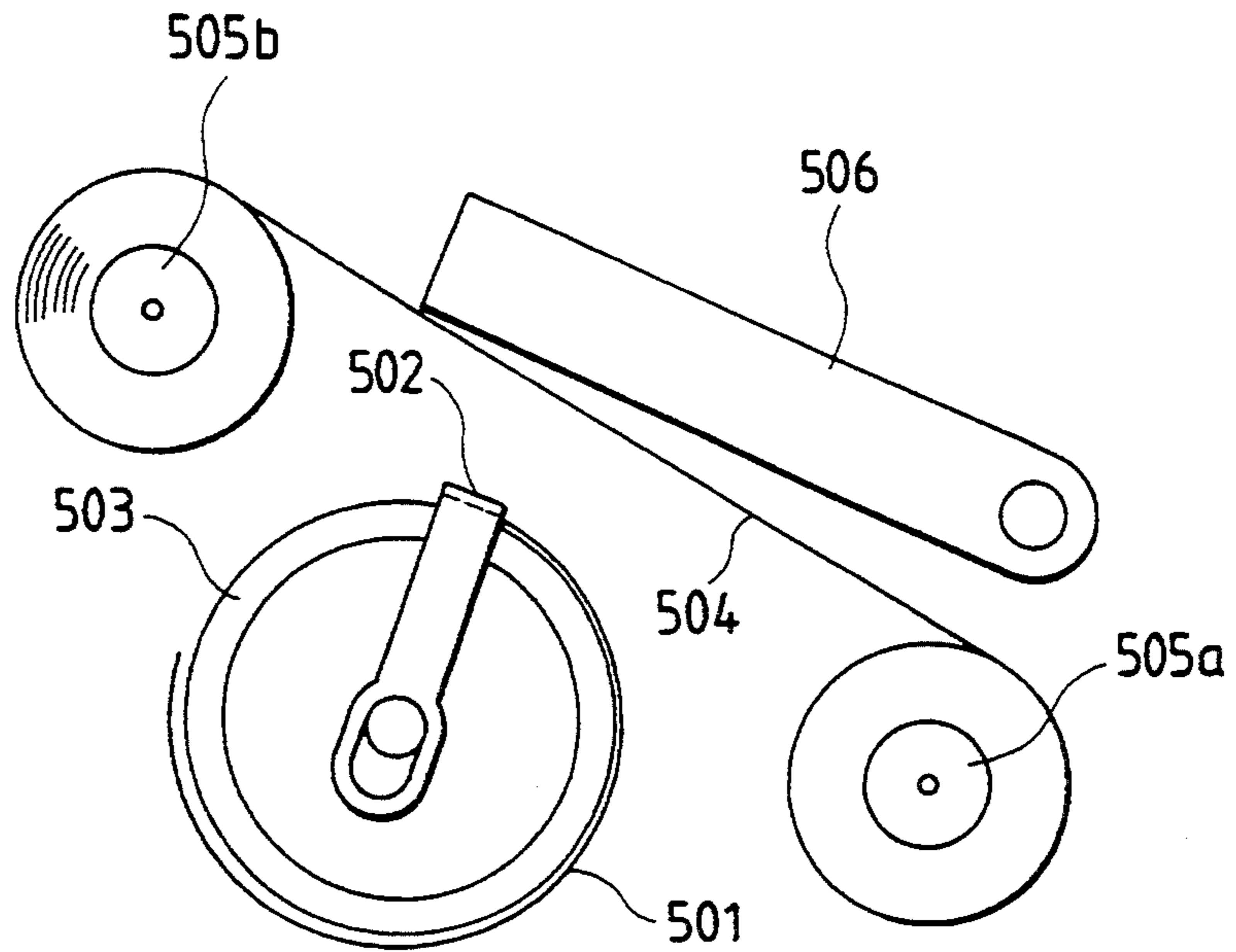
FIG. 26 PRIOR ART
