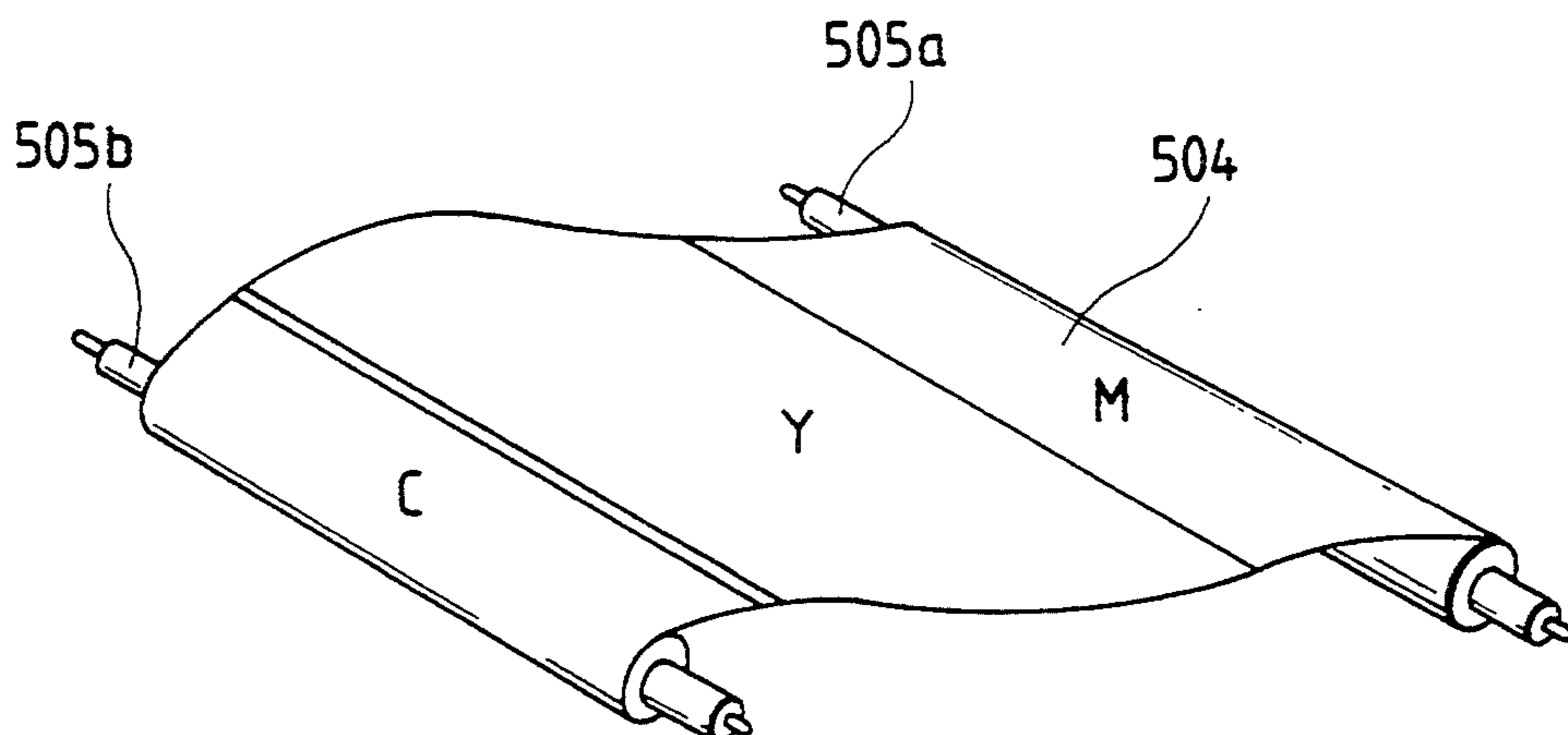
FIG. 29 PRIOR ART
