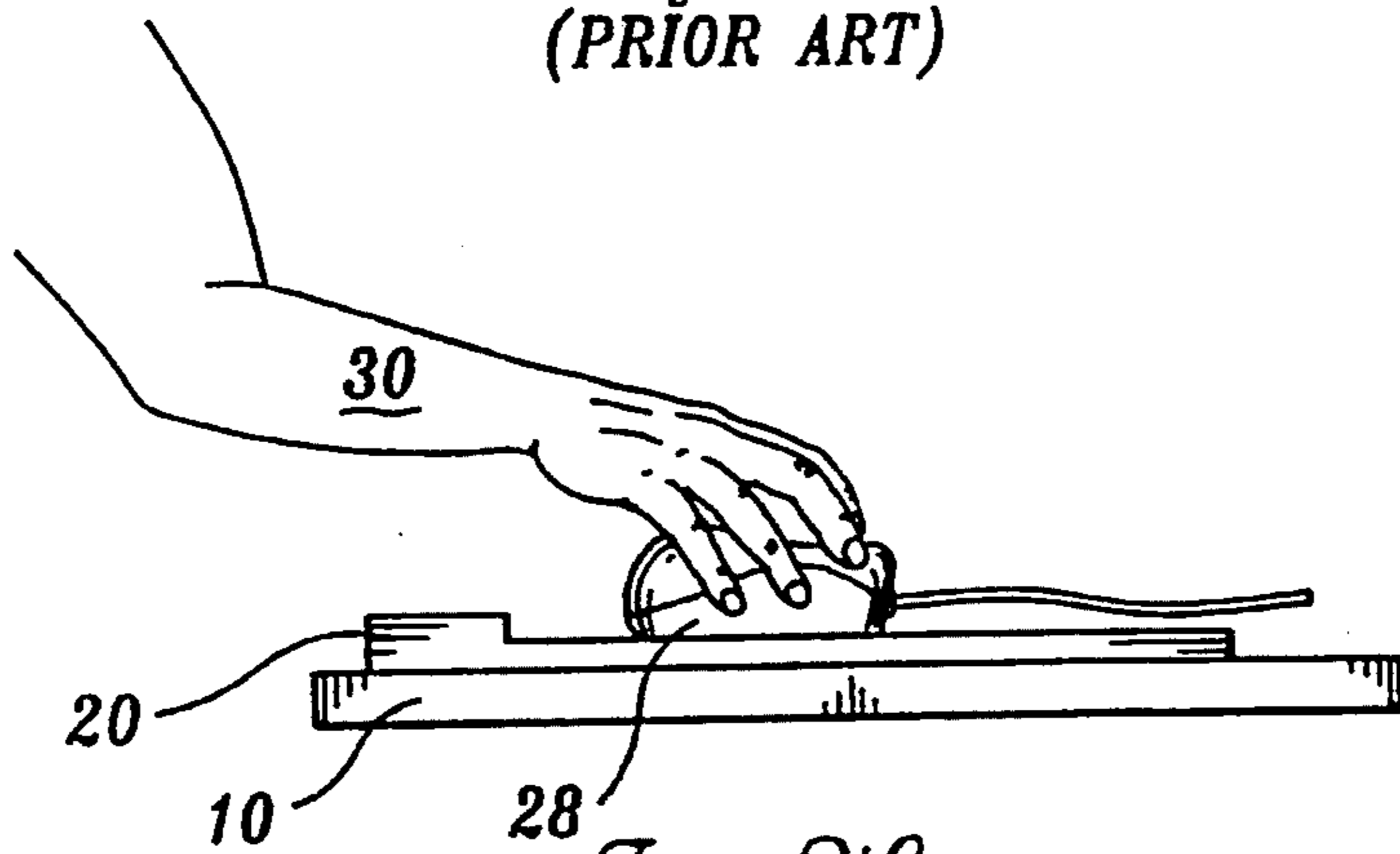
Fig. 2C. (PRIOR ART)
