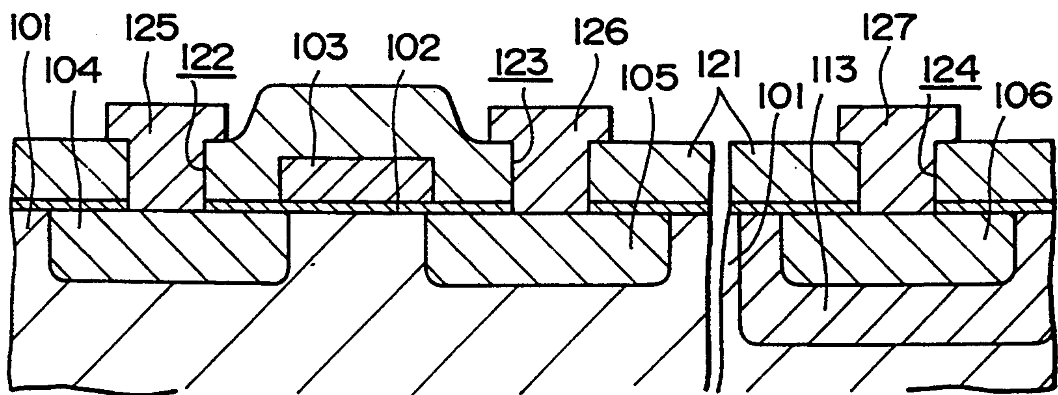
FIG. 11 (PRIOR ART)
