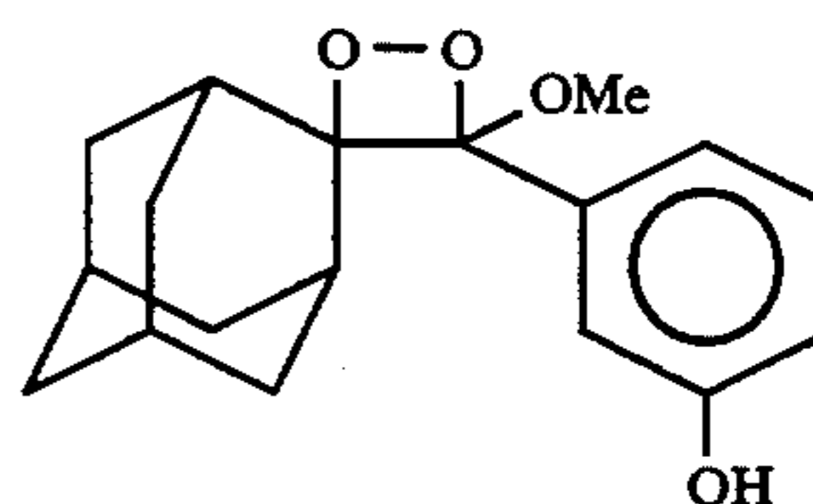
Enhancement of Chemiluminescence from Sodium Hydroxide-Triggering of Dioxetane 5.
