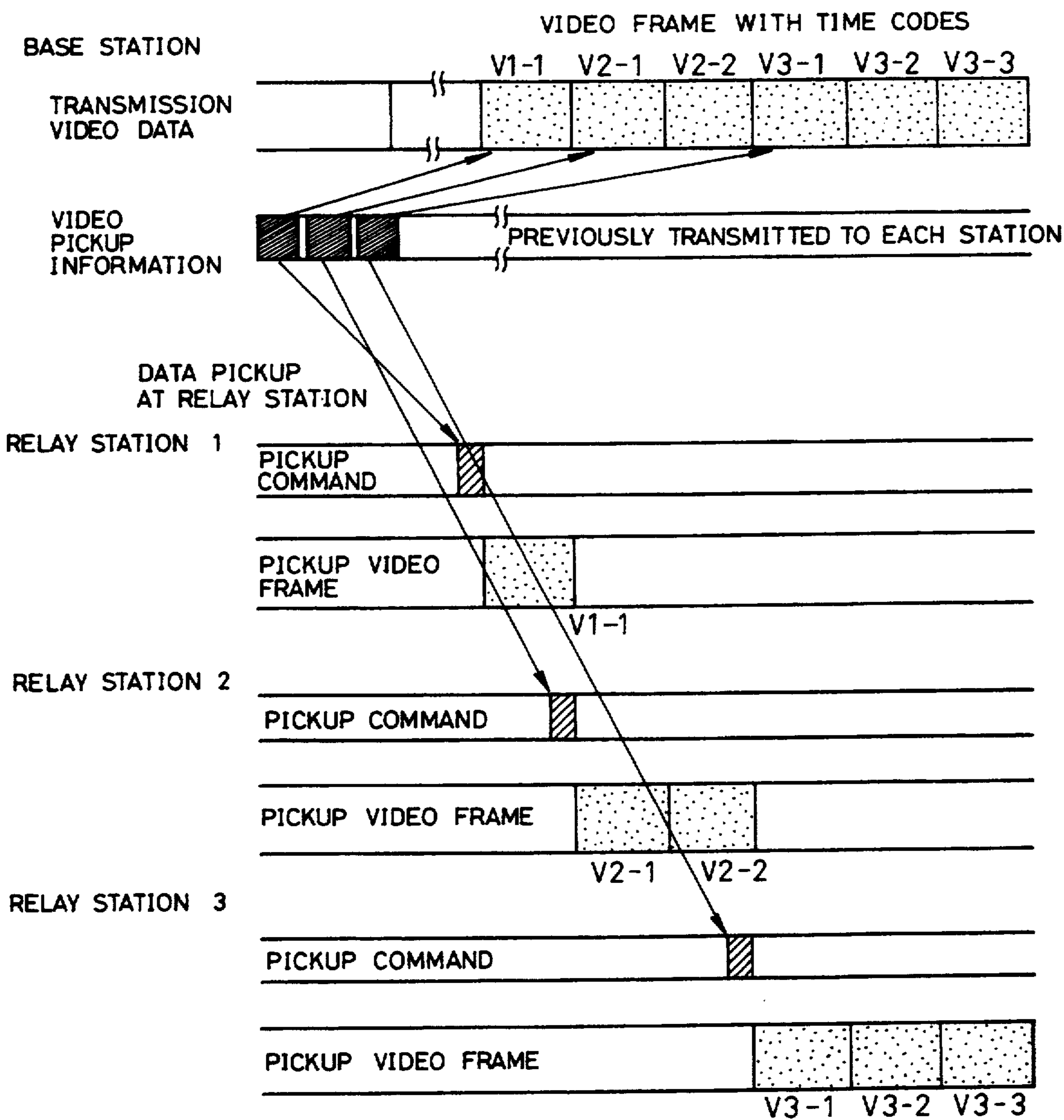
VIDEO PICKUP TIMING
