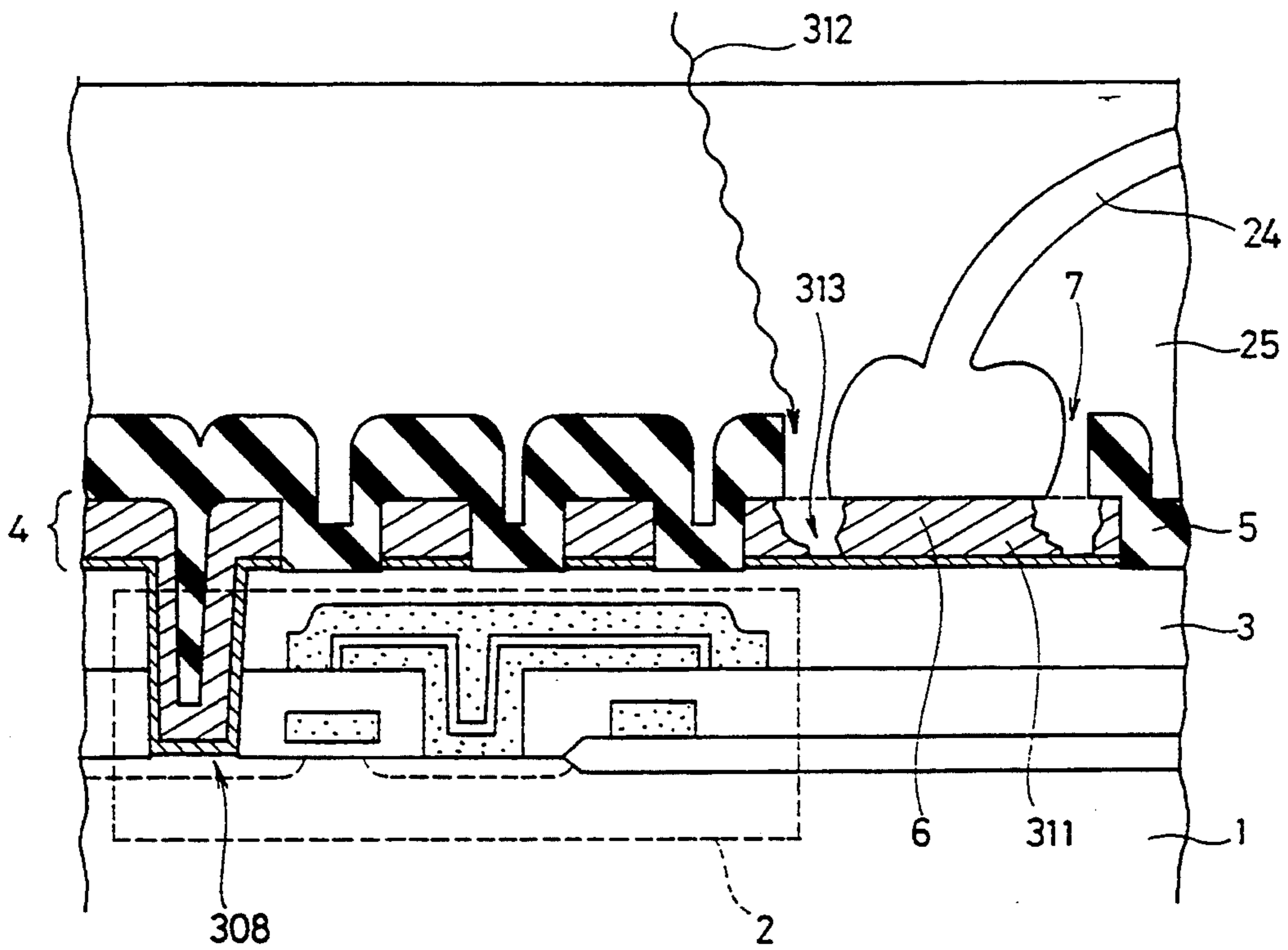
FIG. 4 PRIOR ART
