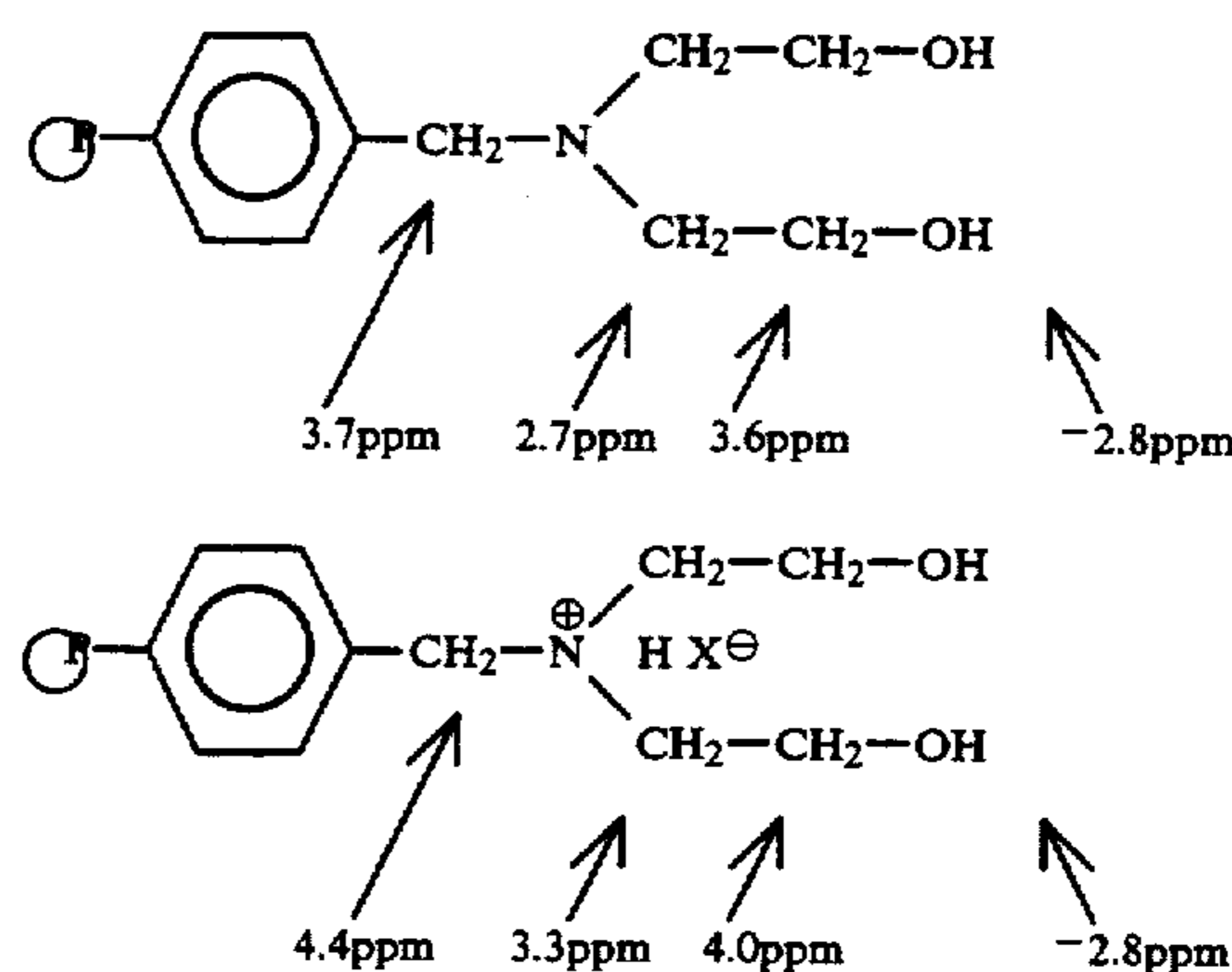
Proton NMR Resonances for Enchained Pendant Functional "mer"Units
