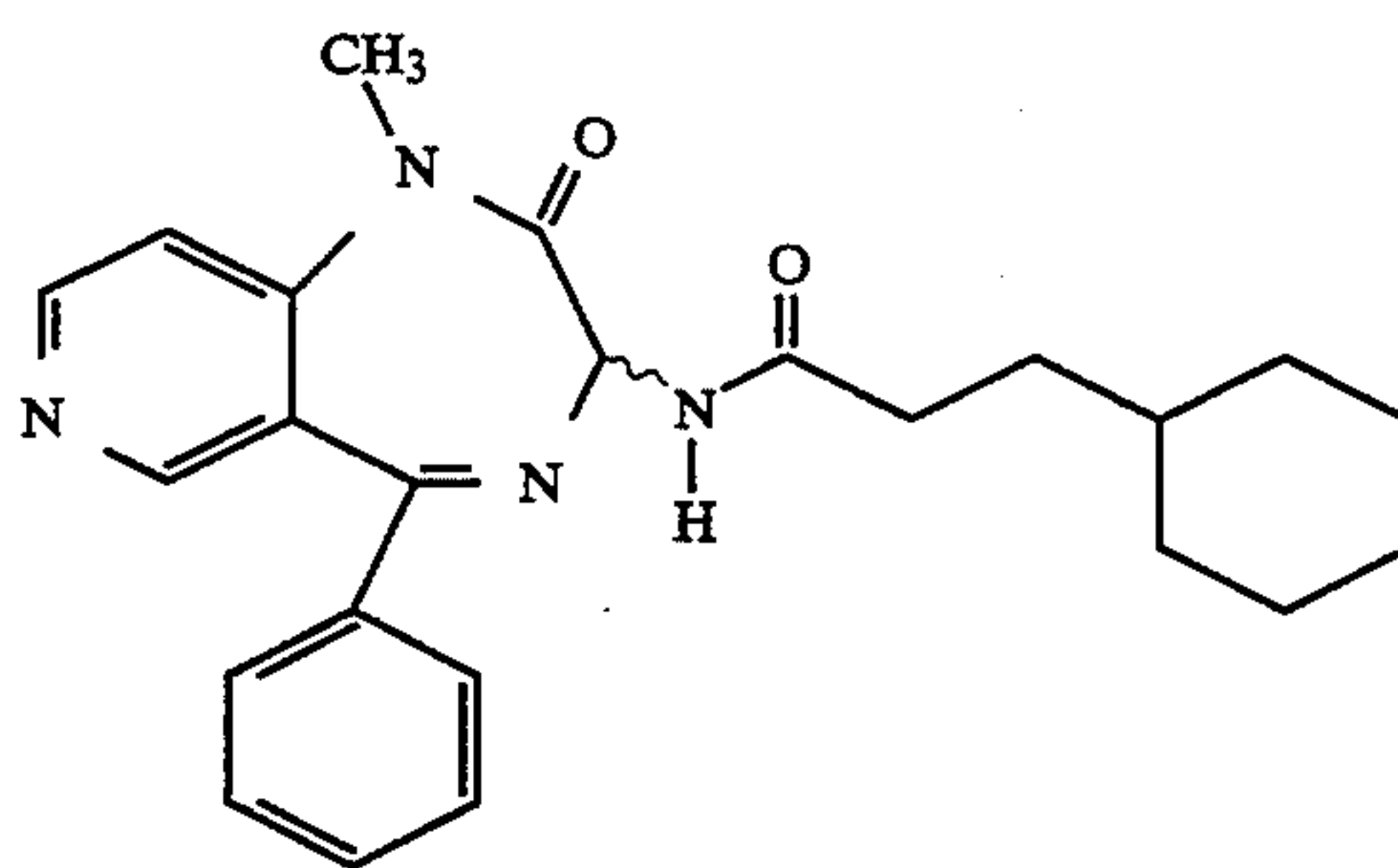
N-(2,3-Dihydro-1-methyl-2-oxo-5-phenyl-1H-pyrido[4,3-e]-1,4-diazepin-3-yl)-3-(cyclohexyl)propanamide
