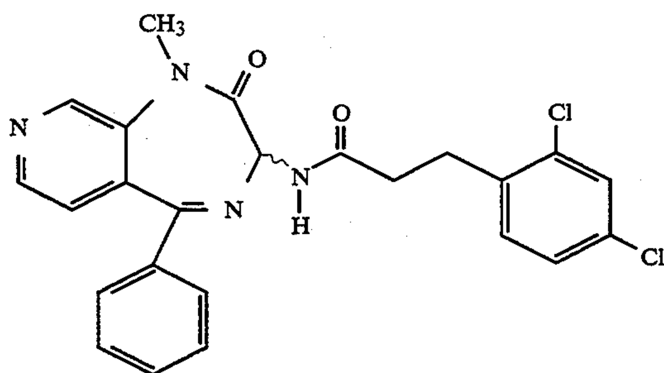
N-(2,3-Dihydro-1-methyl-2-oxo-5-phenyl-1H-pyrido[3,4-e]-1,4-diazepin-3-yl)-3-(2,4-dichlorophenyl)propanamide
