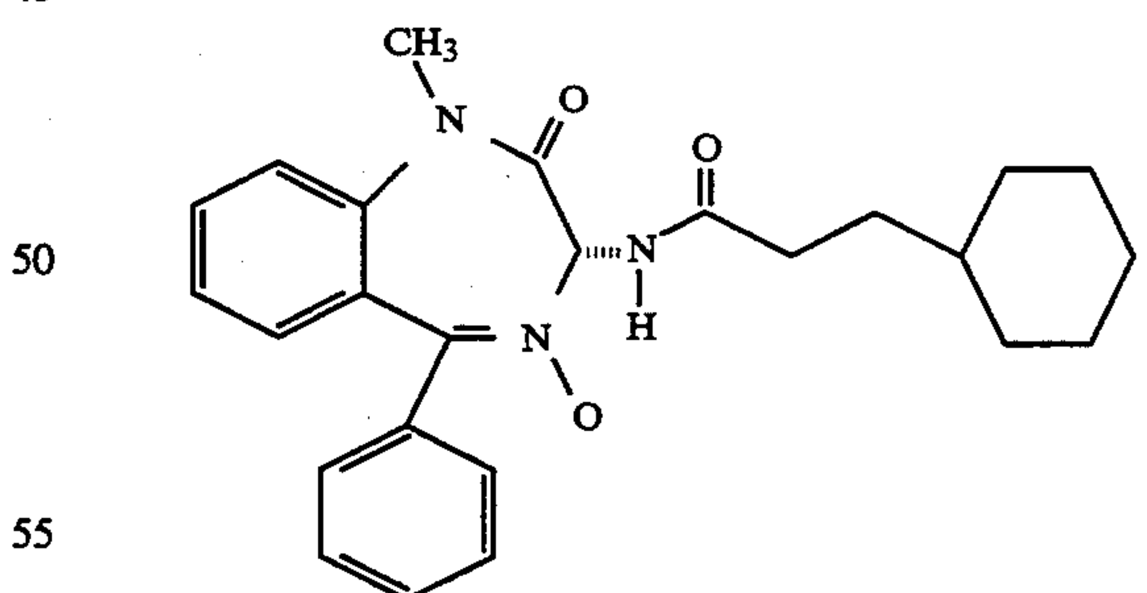
(-)-3-Cyclohexyl-N-[(3R)-2,3-dihydro-1-methyl-2-oxo-4-oxido-5-phenyl-1H-1,4-benzodiazepin-3-yl]propanamide
