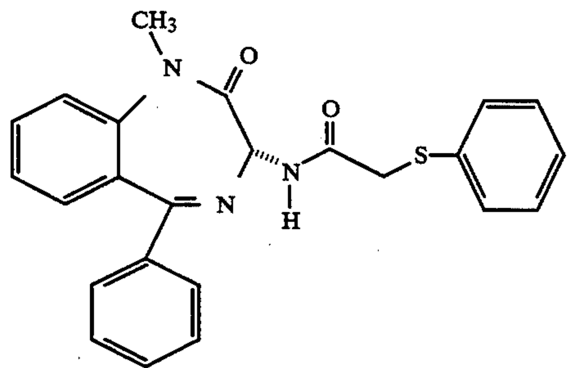
(+)-N-[(3R)-2,3-Dihydro-1-methyl-2-oxo-5-phenyl-1H-1,4-benzodiazepin-3-yl]-2-(phenylthio)acetamide
