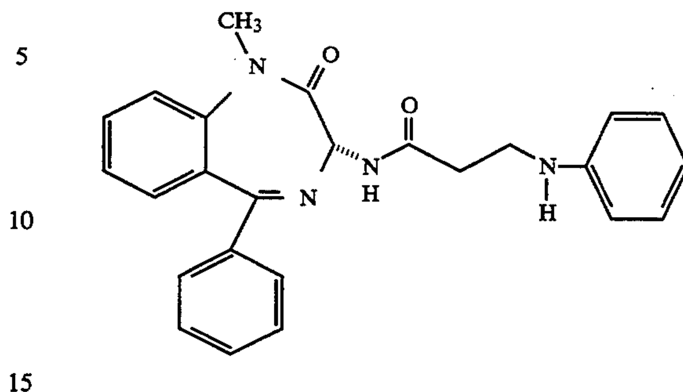
(+)-N-[(3R)-2,3-Dihydro-1-methyl-2-oxo-5-phenyl-1H-1,4-benzodiazepin-3-yl]-3-(phenylamino)propanamide
