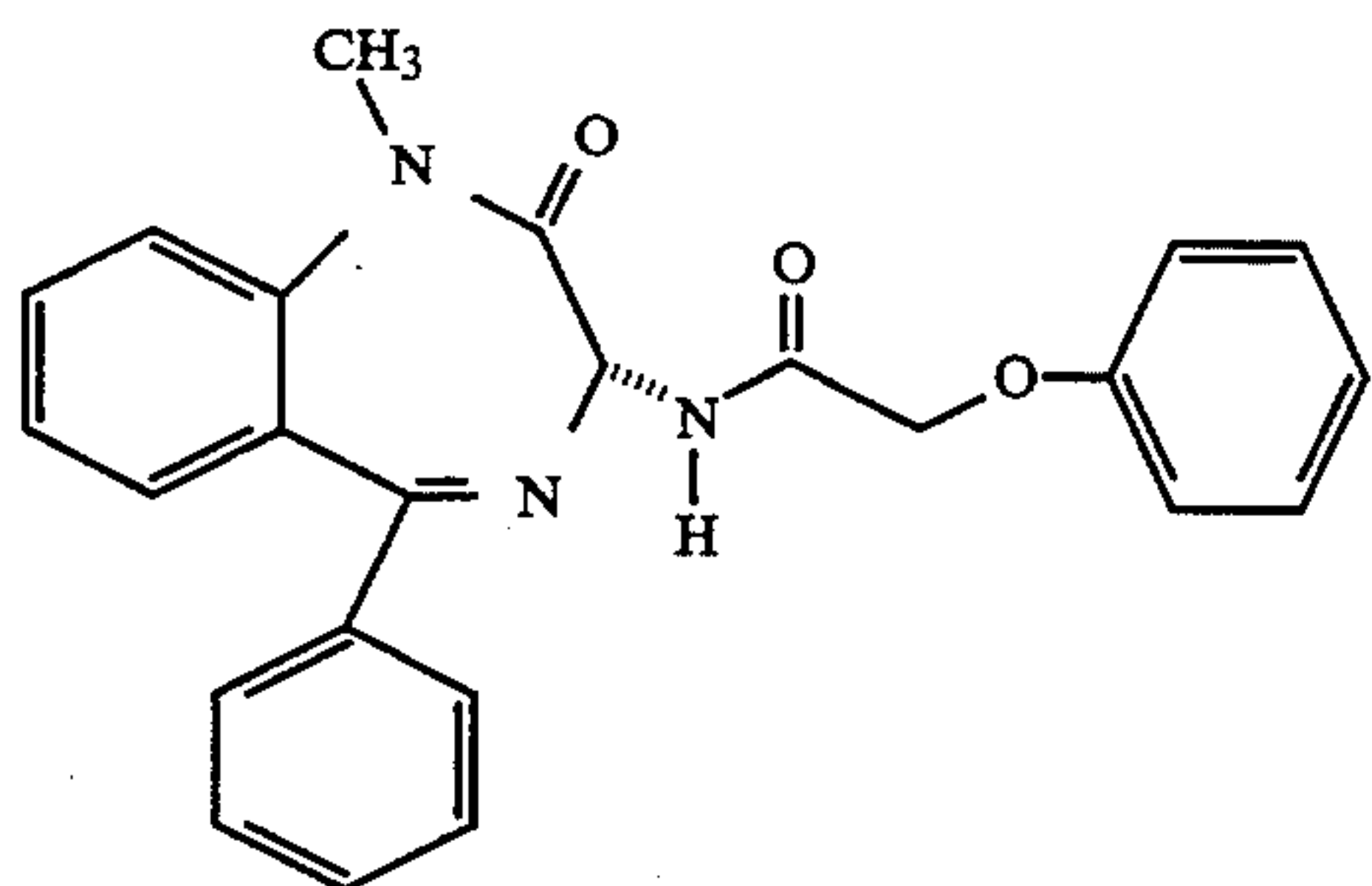
(+)-N-[(3R)-2,3-Dihydro-1-methyl-2-oxo-5-phenyl-1H-1,4-benzodiazepin-3-yl]-2-(phenoxy)acetamide
