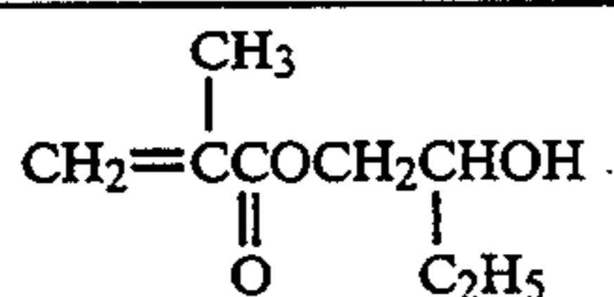
1 Molecular structural formula (K)
