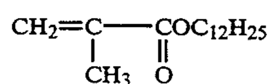
Molecular structural formula (e)
