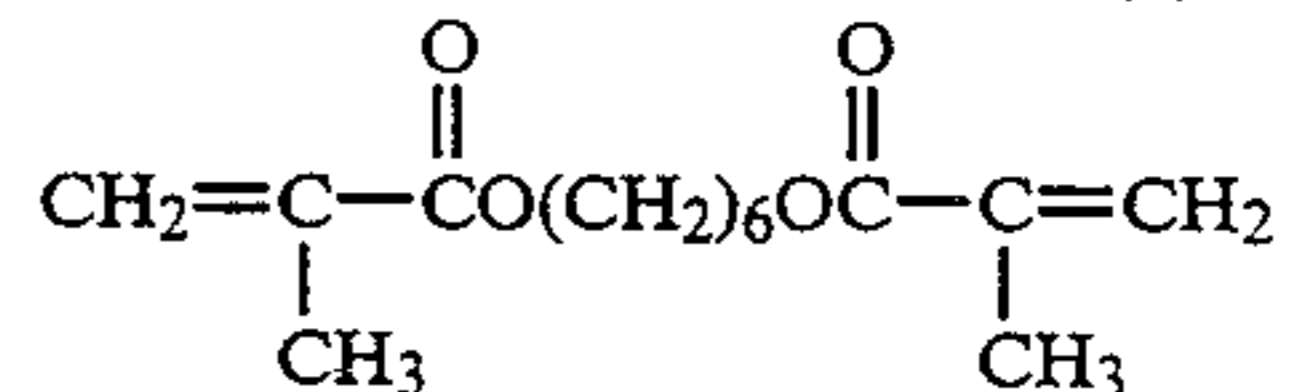
Molecular structural formula (o)
