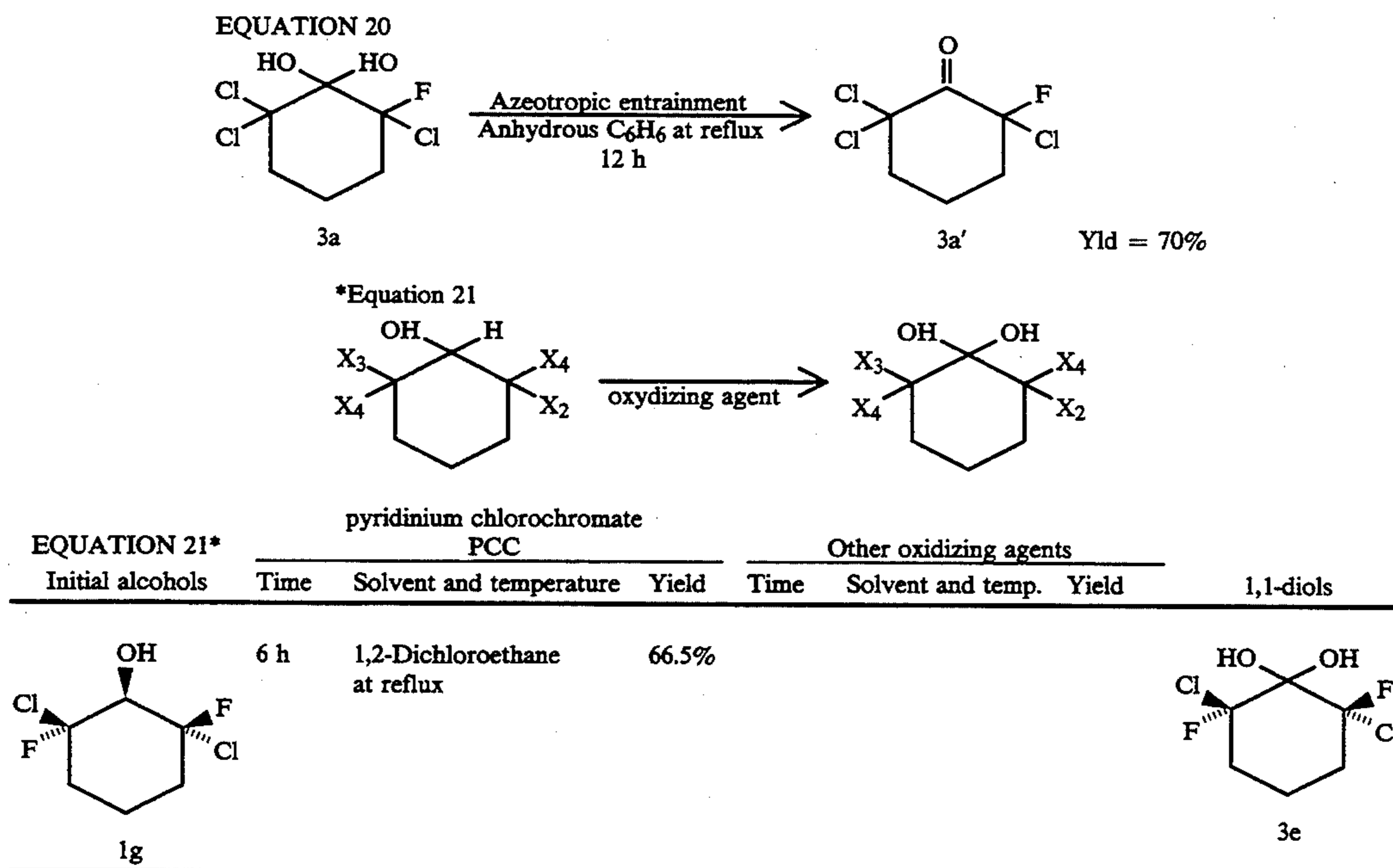
Scheme 5: Preparation of the tetrahalogenated hydrates and of the corresponding ketones
