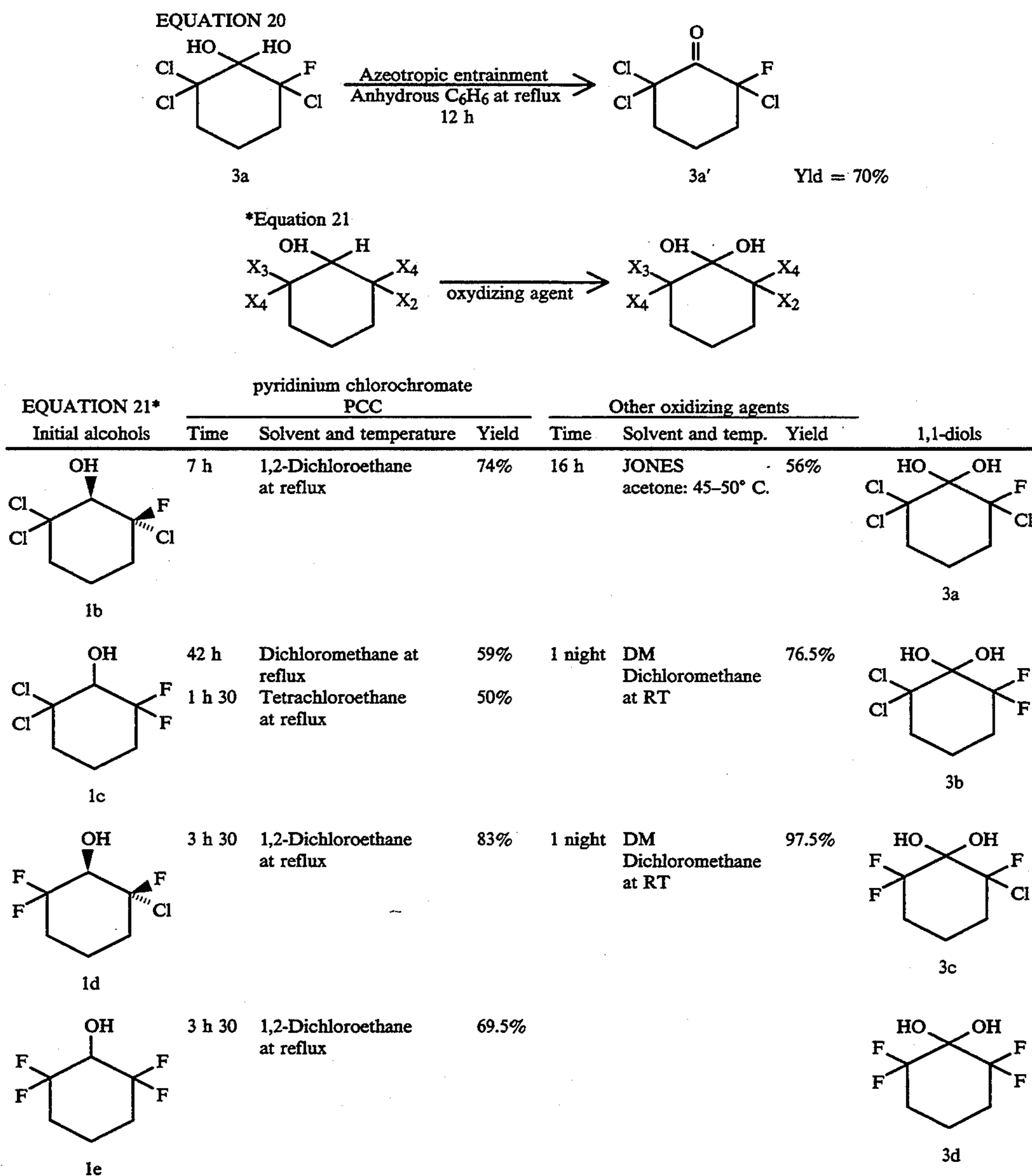
Scheme 5: Preparation of the tetrahalogenated hydrates and of the corresponding ketones
