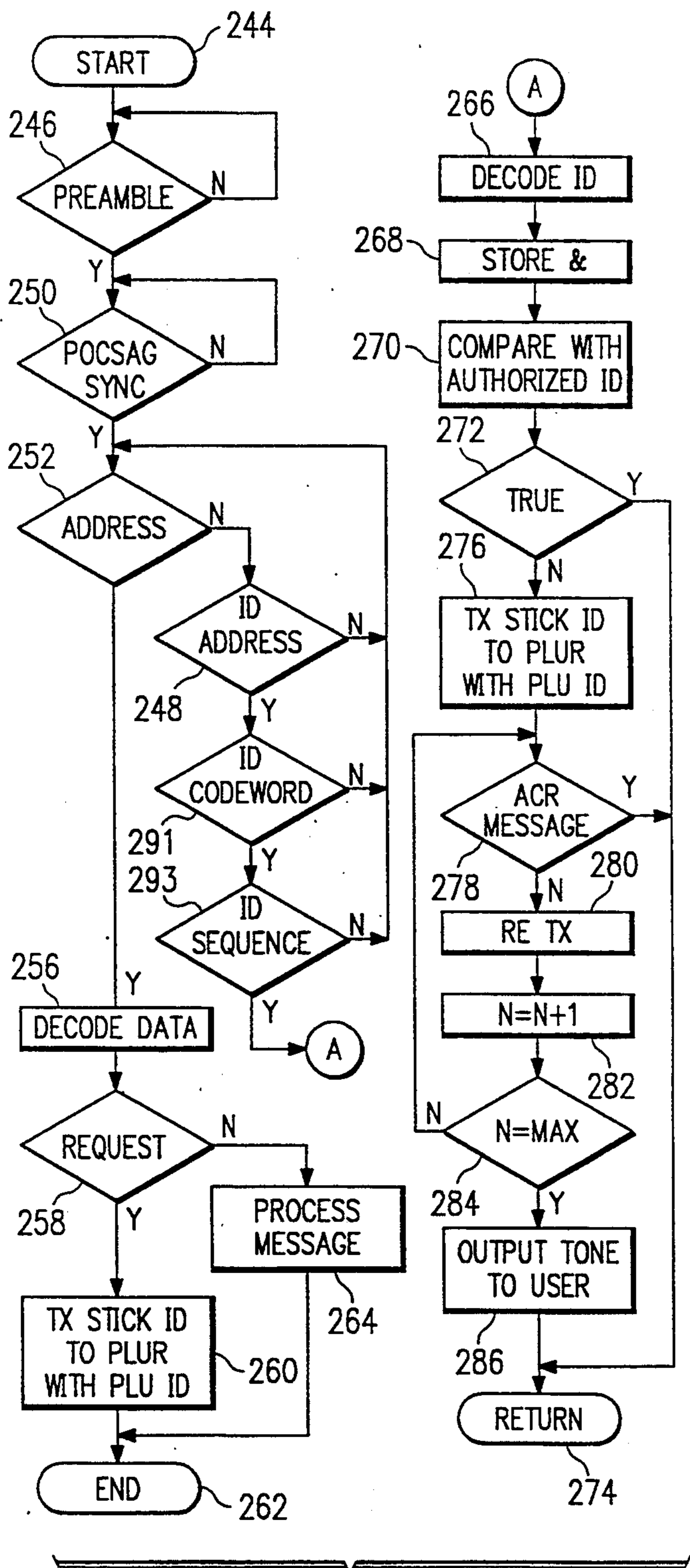
FIG. 9 PLU FLOW CHART
