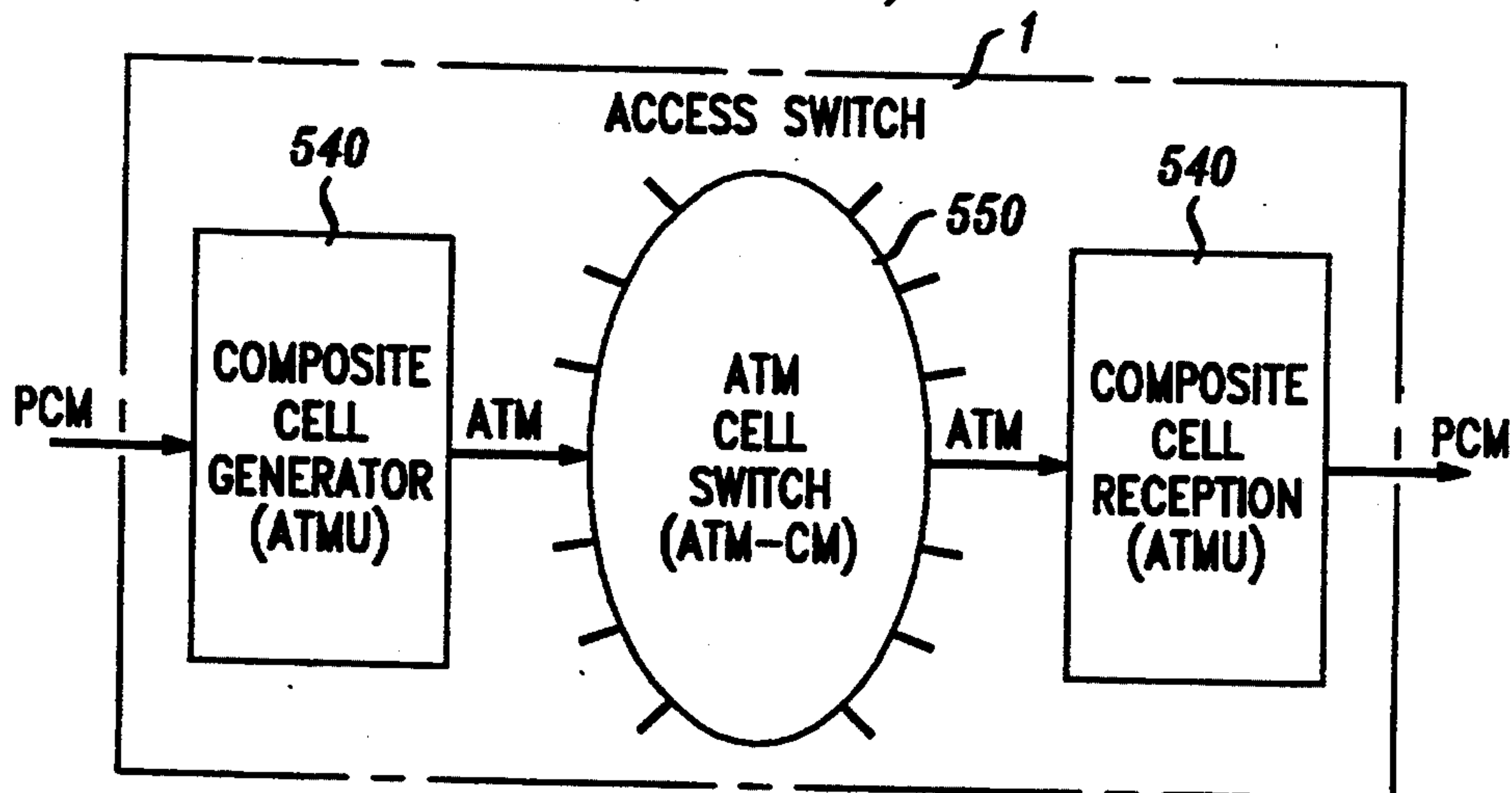
FIG. 1 (PRIOR ART)
