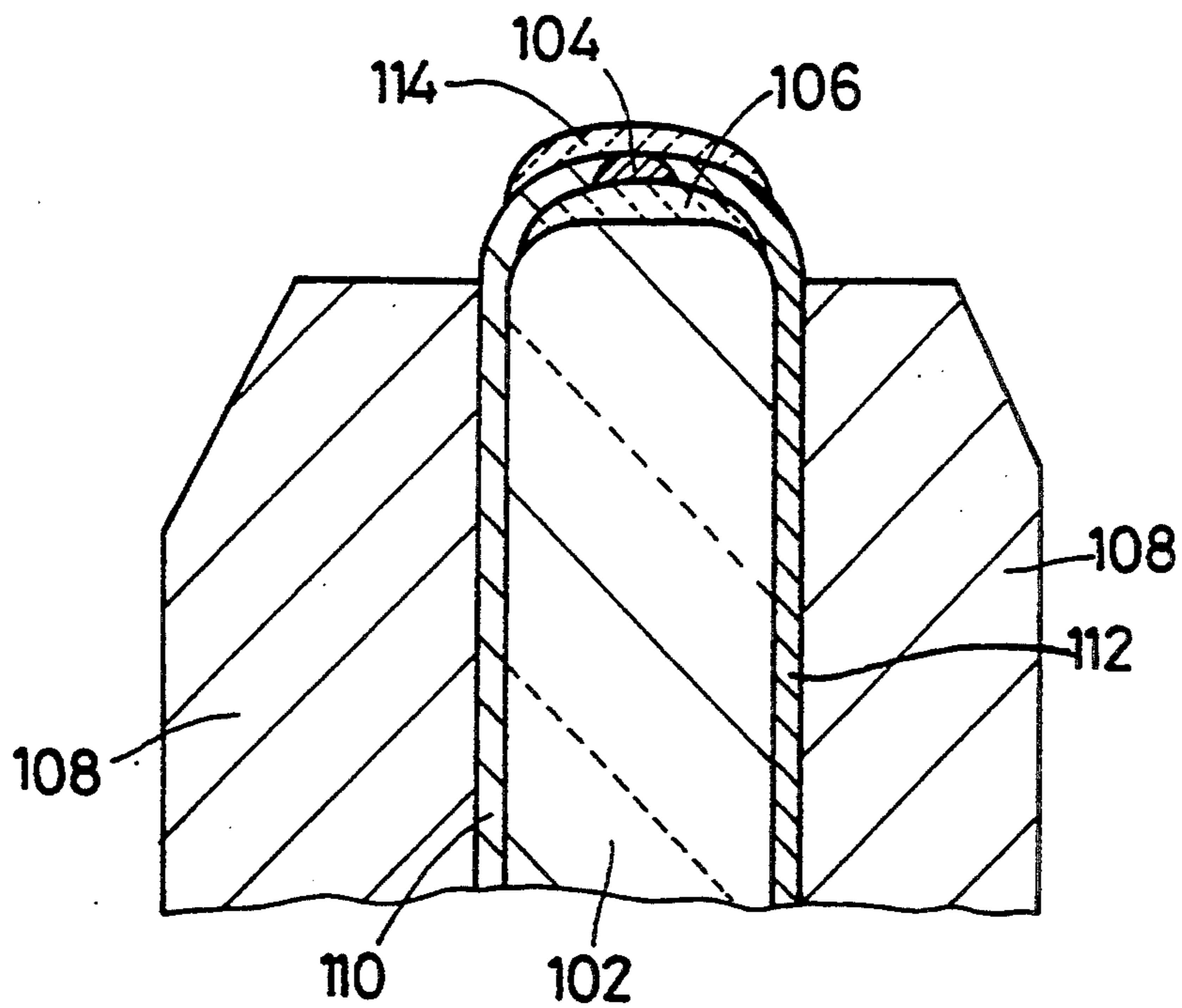
FIG. 38 PRIOR ART
