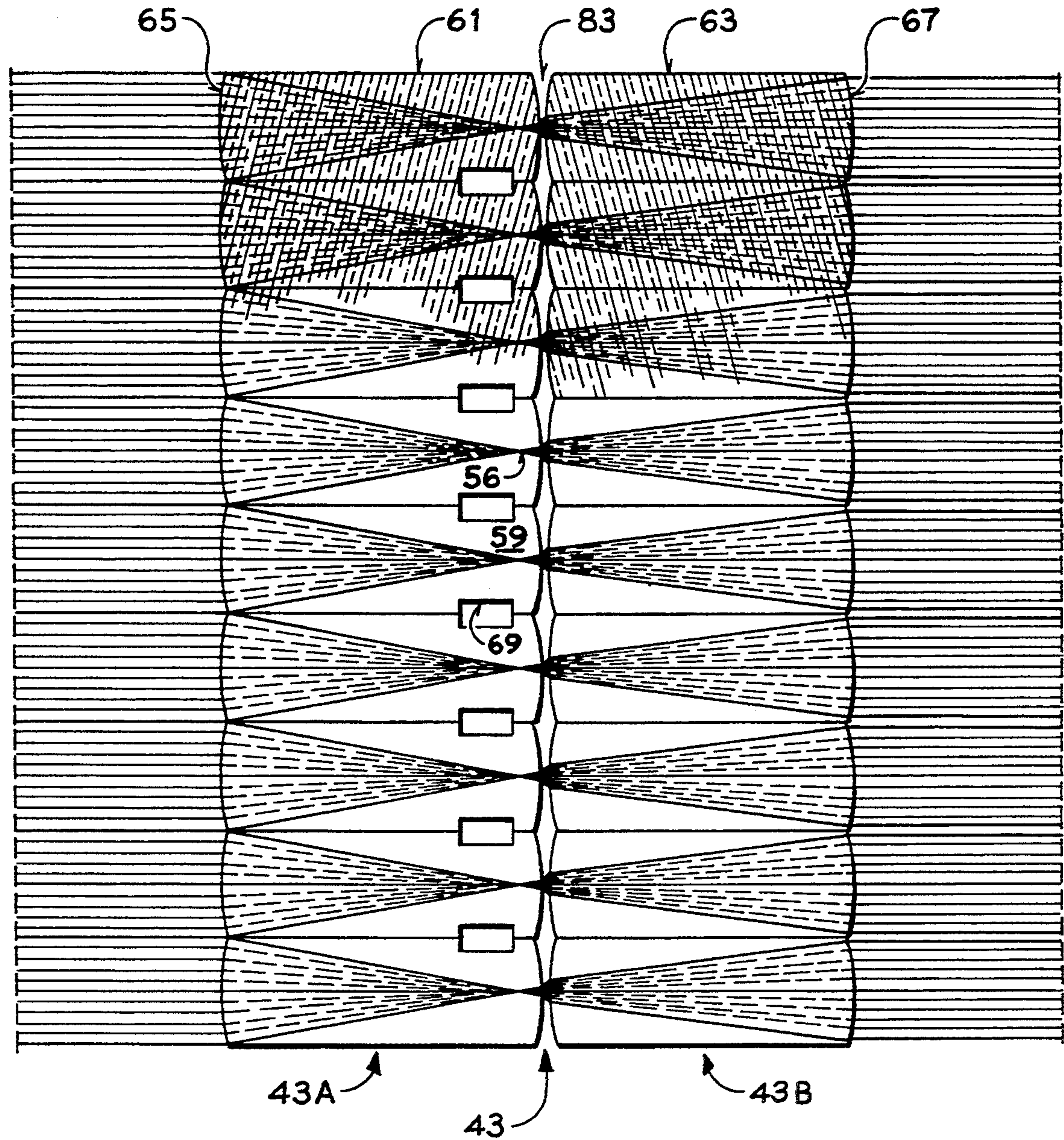
ARRAY CROSS-SECTION FOR 0-deg SCAN
