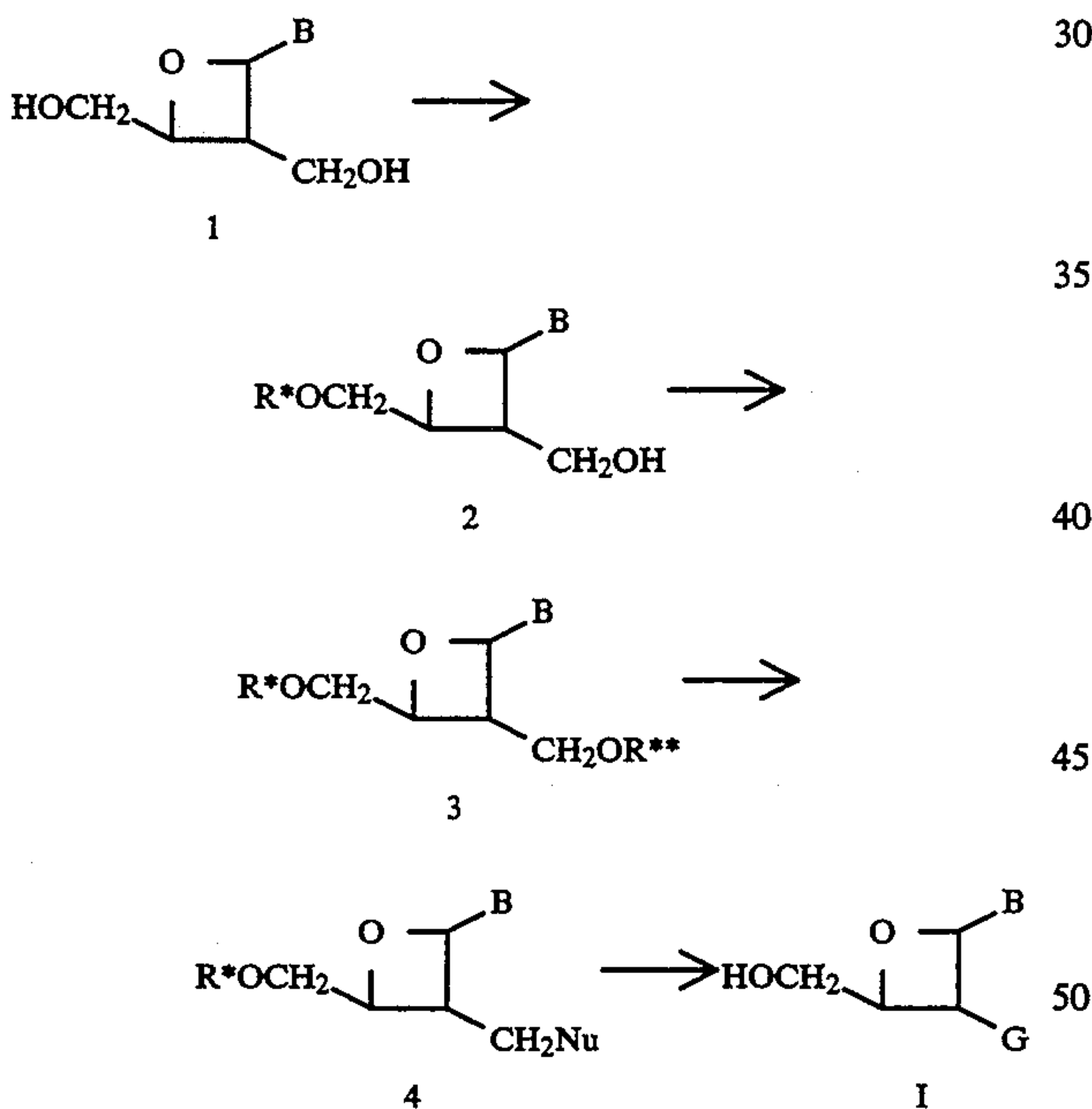
SCHEME 1
