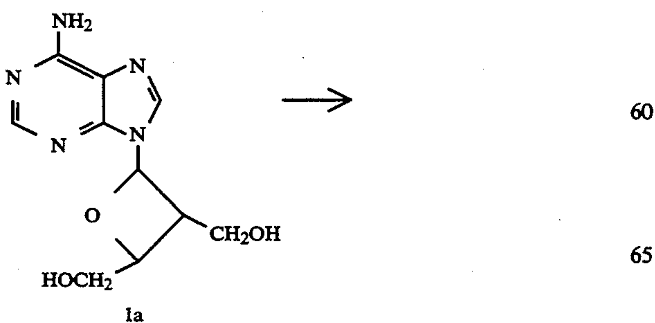
SCHEME 2
