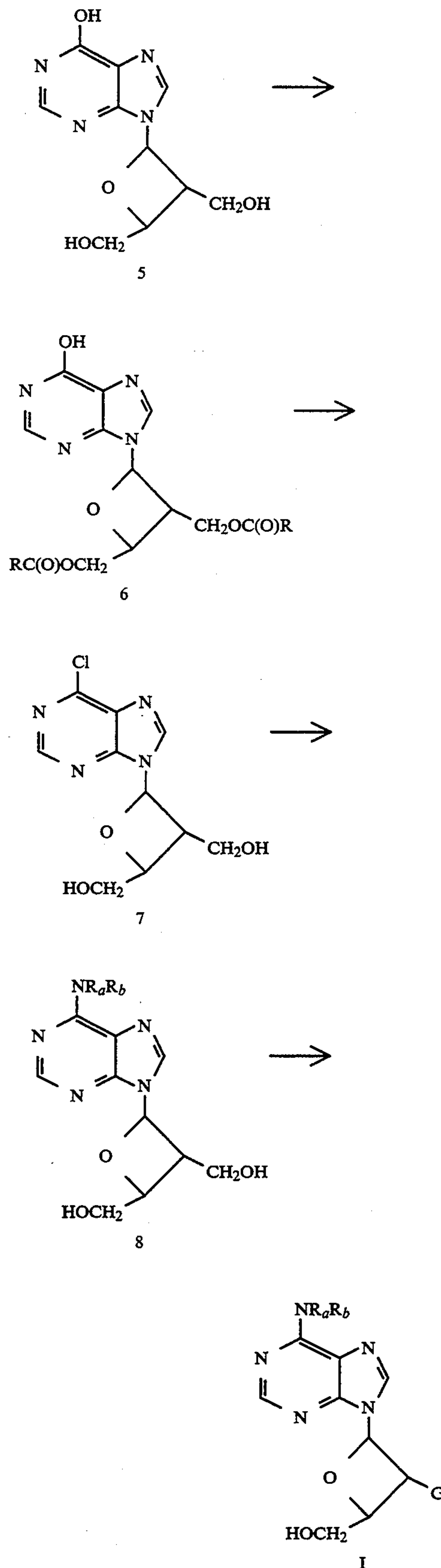
SCHEME 2
