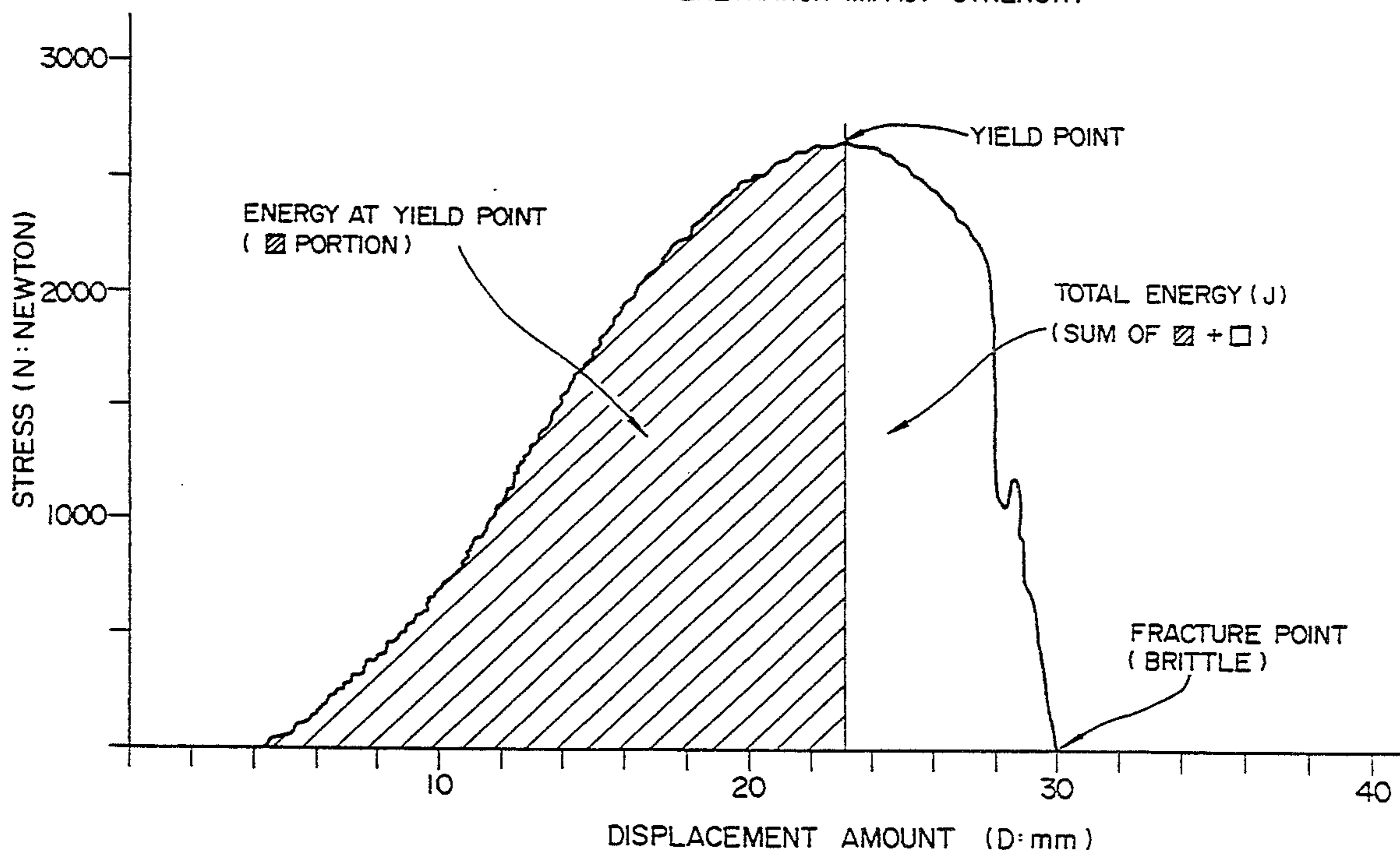
MEASUREMENT OF PENETRATION IMPACT STRENGTH
