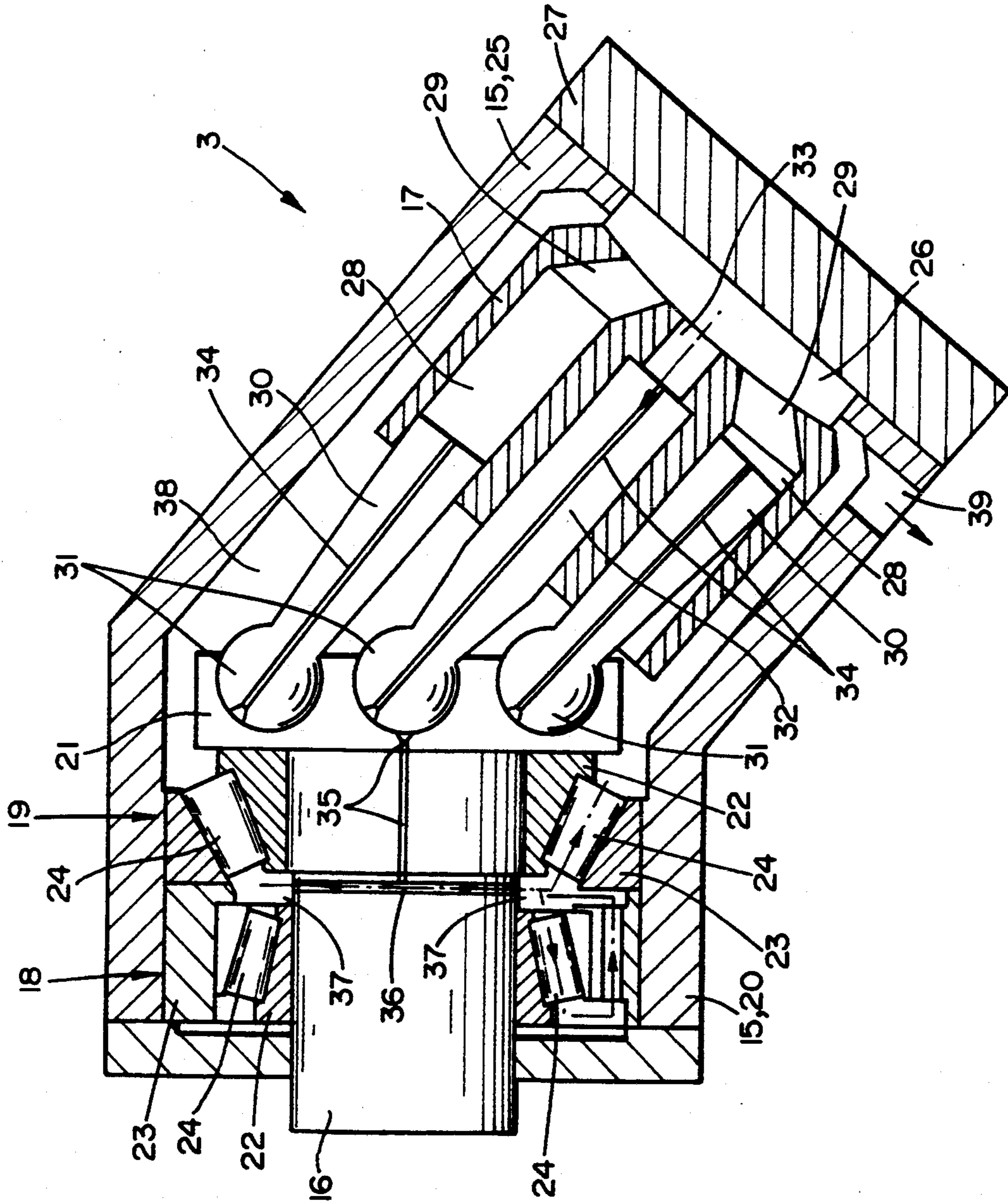
FIG. 4 PRIOR ART
