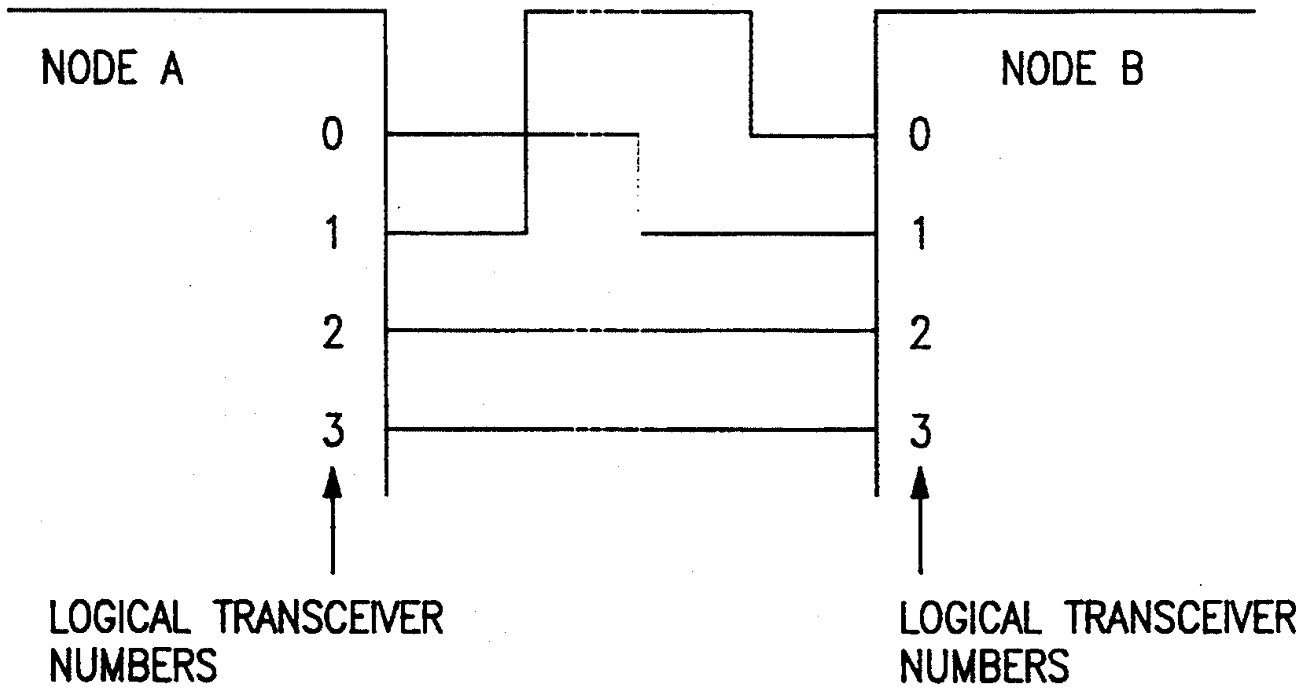
CROSSED TRANSCEIVER MISMATCH
