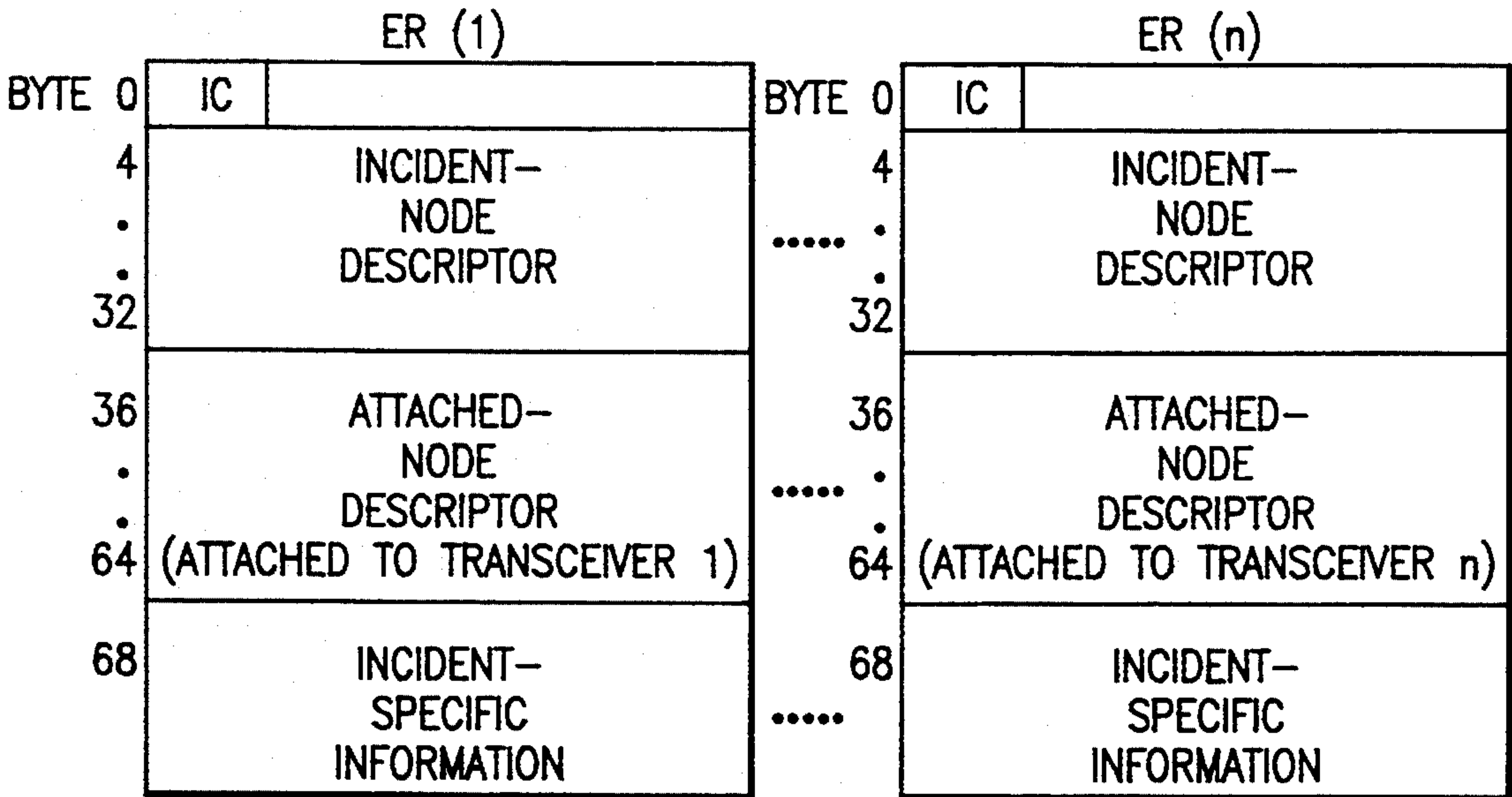
CHAINED ERROR RECORDS (ERs) FIG.16
